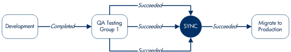
Figure 3-7. SYNC example
