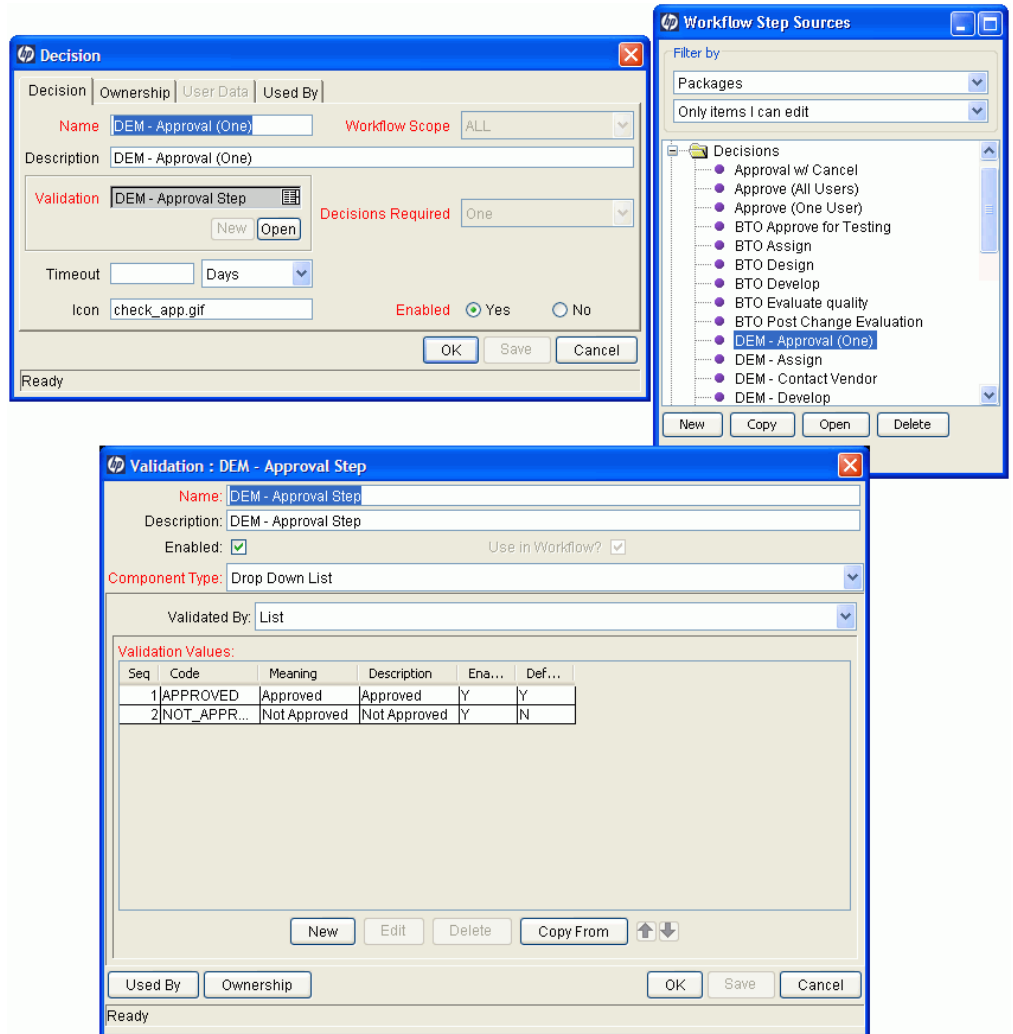
Figure 3-14. Workflow step sources and validations
