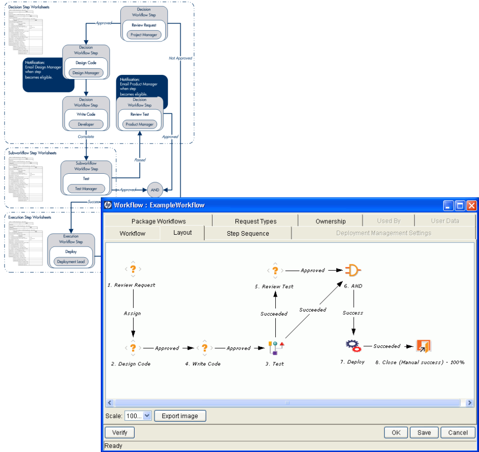
Figure 3-2. Stage 2. Create the workflow
