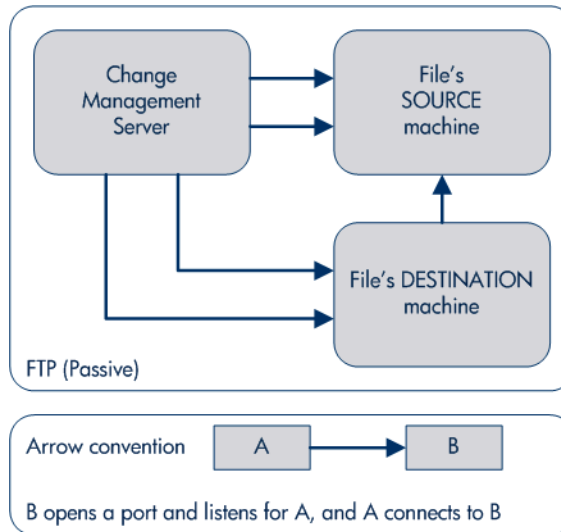
Figure 7-3. FTP (passive)
