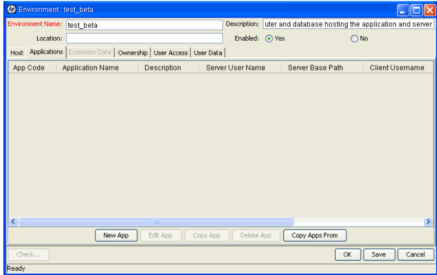
Figure 7-5. Applications tab
