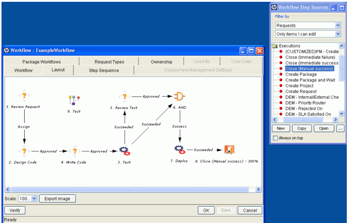
Figure 3-9. Close step
