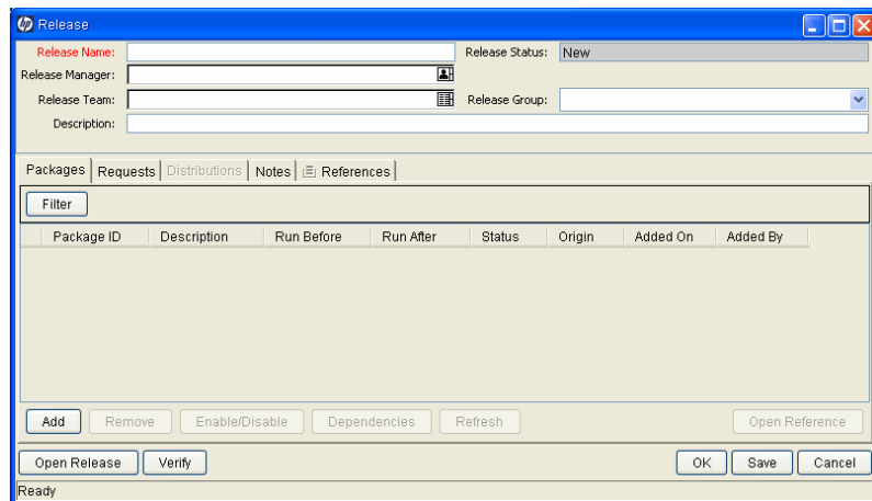
Figure 6-5. Release window
