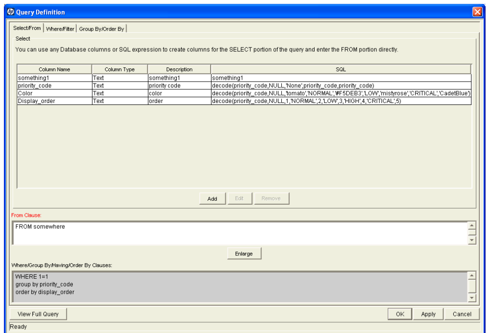
Figure 3-14. Color map in the portlet data source
