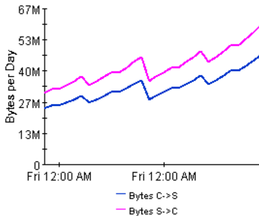
Bytes Client159
