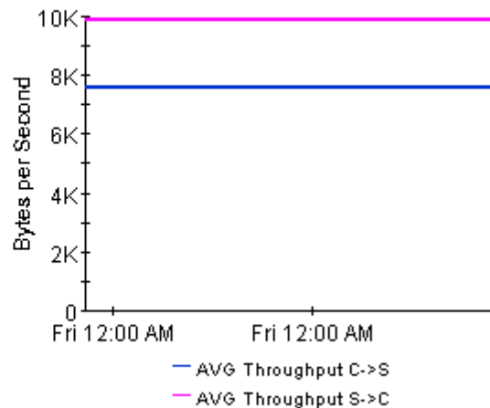
Throughput Client159
