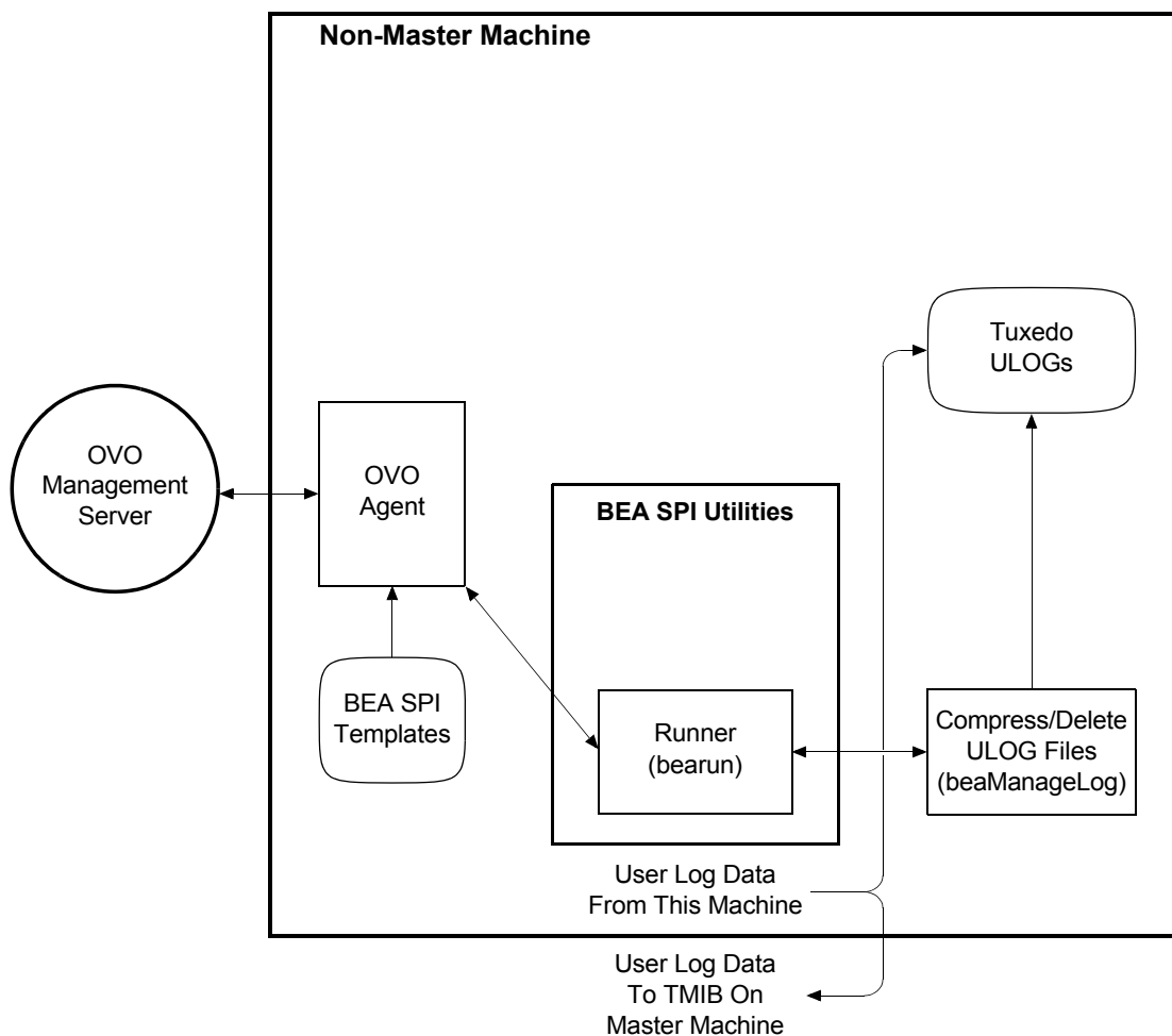
Figure 5 OVO and Tuxedo SPI Software on a Tuxedo Non-Master Machine
