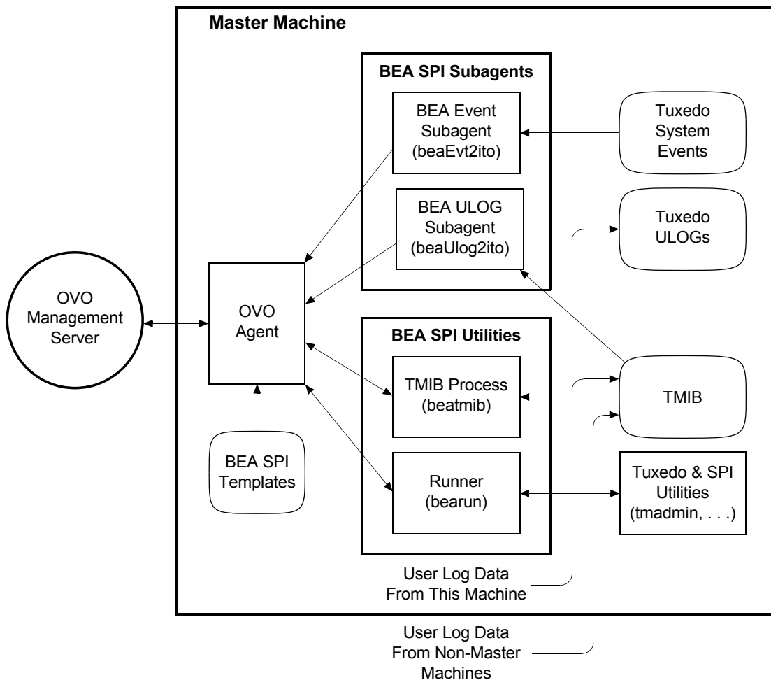
Figure 4 OVO and Tuxedo SPI Software on a Tuxedo Master Machine
