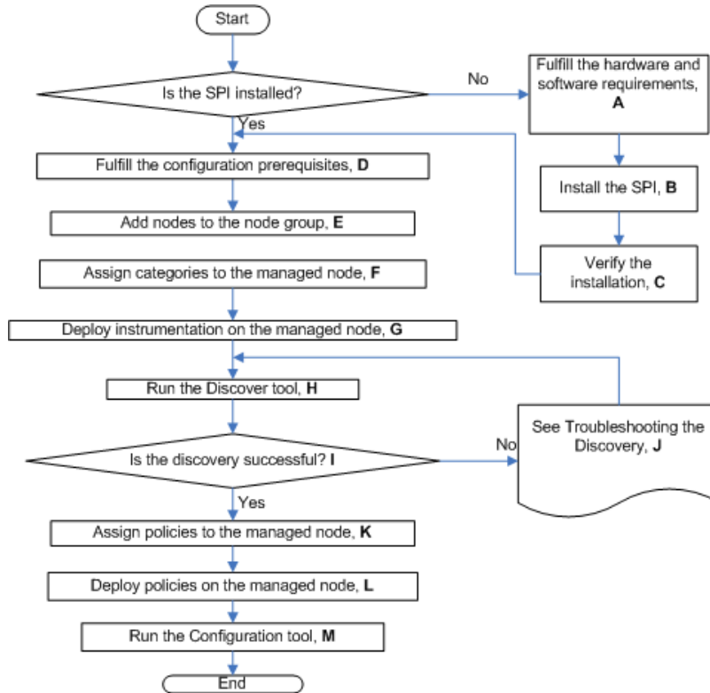
Figure 7 Flowchart for installing and configuring the SPI for Linux or Solaris
