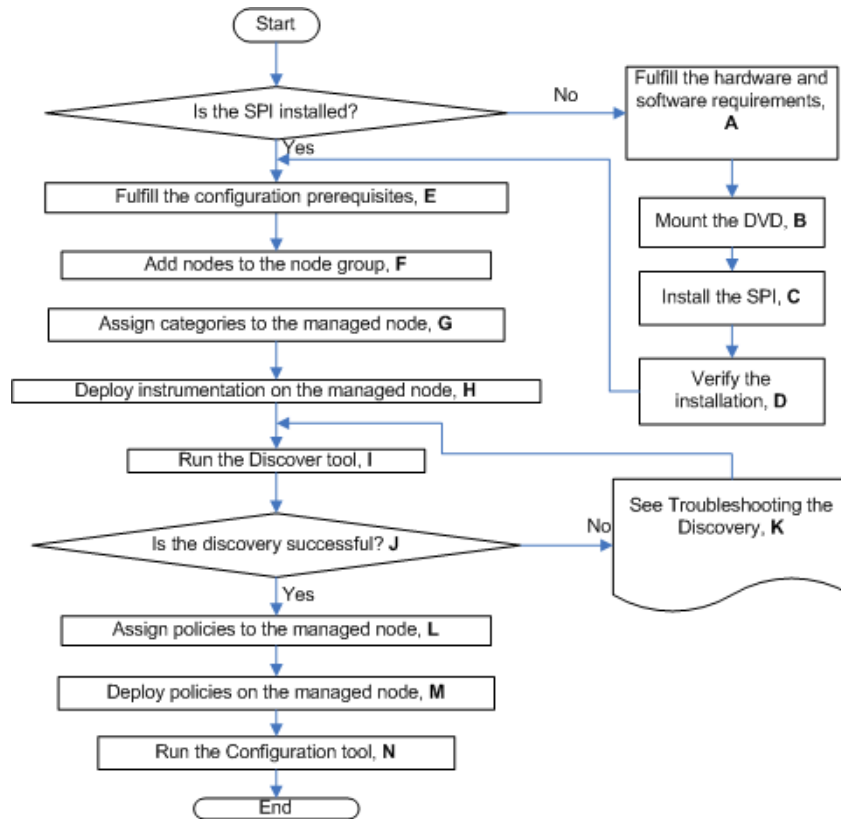
Figure 6 Flowchart on steps for installing and configuring the SPI for HP-UX
