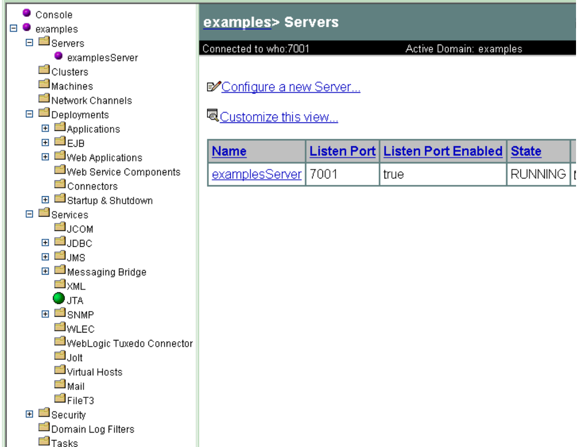
Figure 9 The WebLogic Admin Server console
