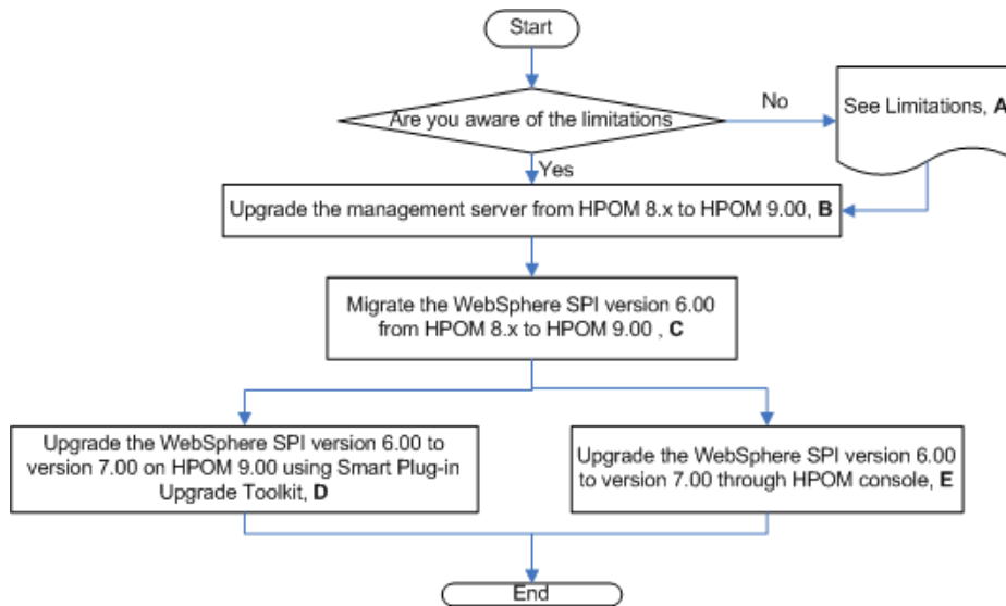
Figure 8 Flowchart on steps for upgrading the SPI on HP-UX and Solaris
