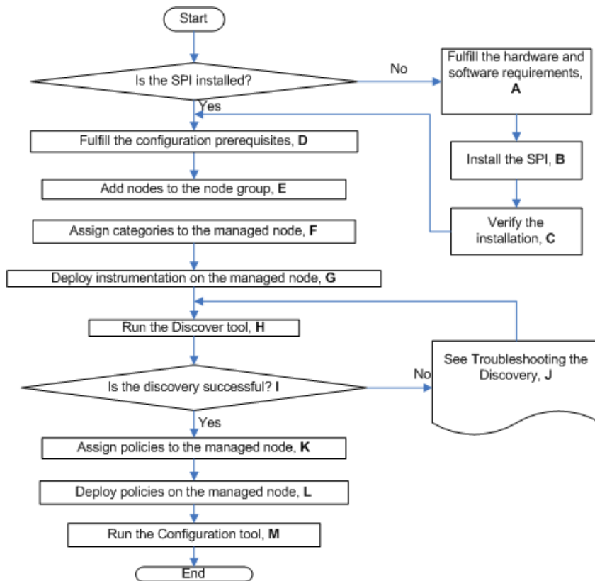
Figure 6 Flowchart for installing and configuring the SPI for Linux and Solaris
