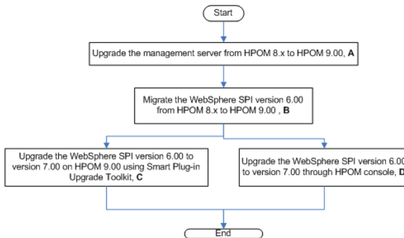
Figure 7 Flowchart to upgrade the WebSphere SPI for HP-UX and Solaris
