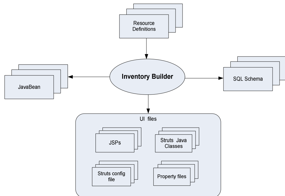
Figure 3-1 Inventory Builder
