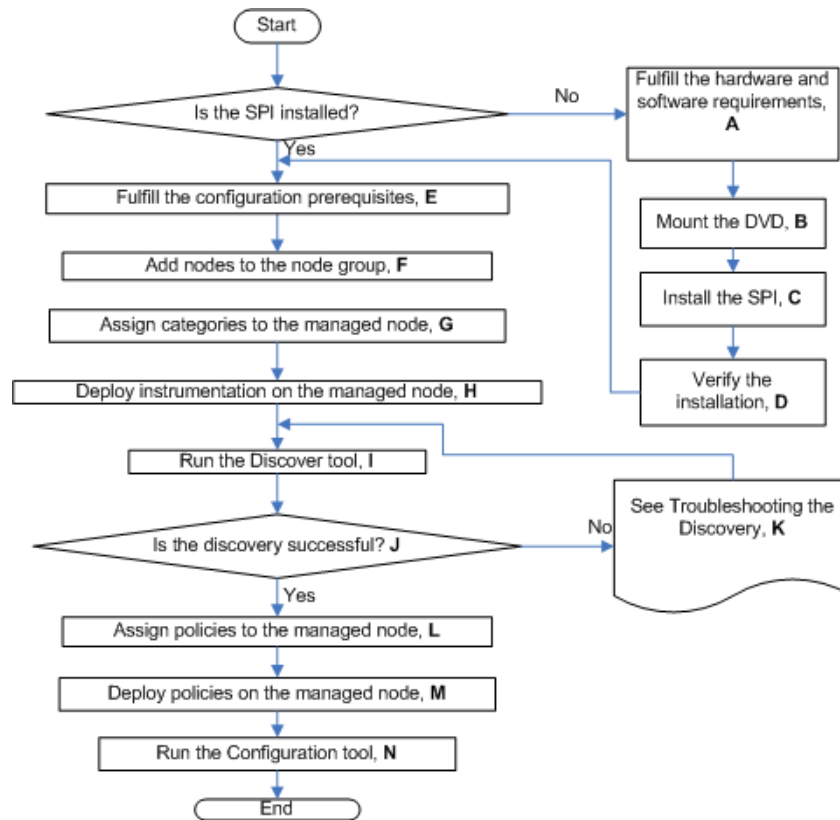
Figure 3 Flowchart on steps for installing and configuring the SPI
