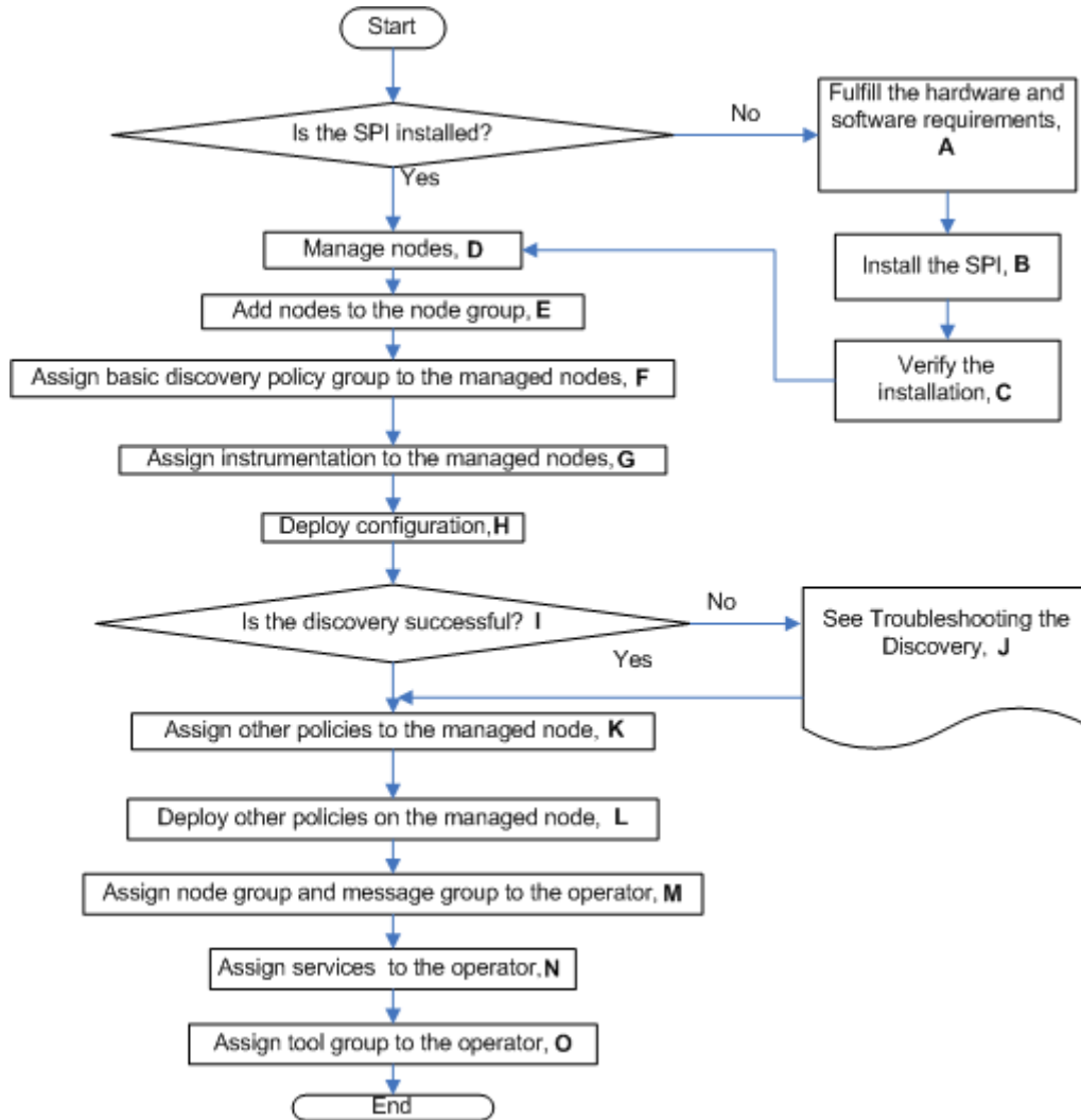
Figure 2 An Overview of Installation and Configuration Steps on Linux
