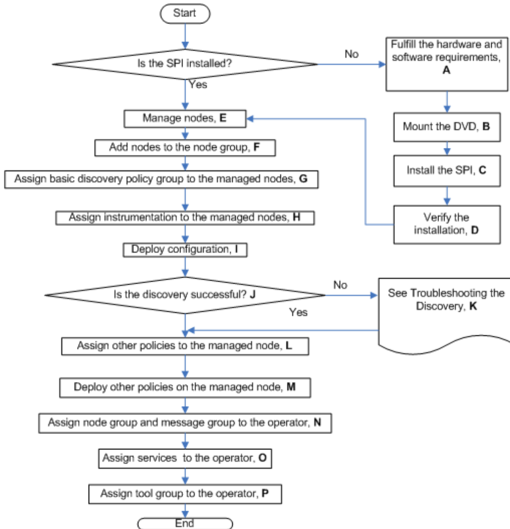
Figure 1 An Overview of Installation and Configuration Steps on HP-UX
