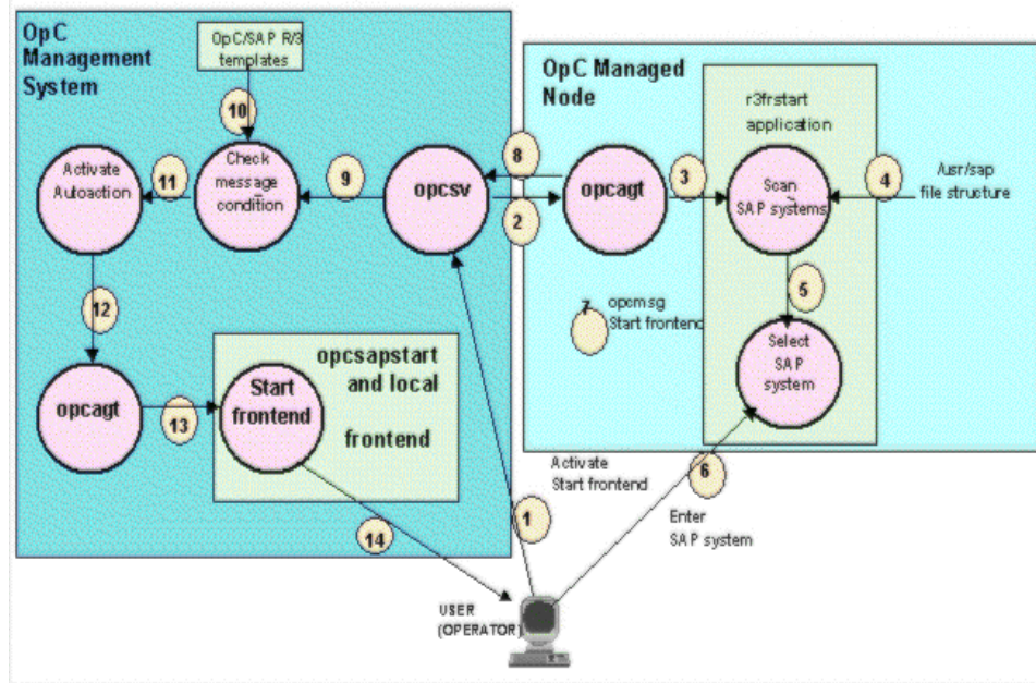
Figure 32 Message Flow between HP Operations Manager and SAP
