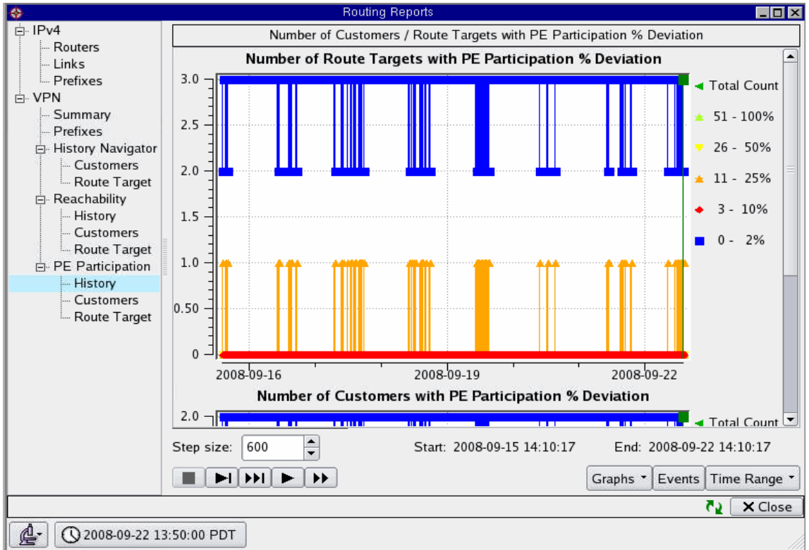
Figure 133 VPN PE Participation Report
