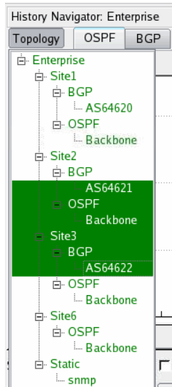
Figure 65 Topology Drop-Down List
