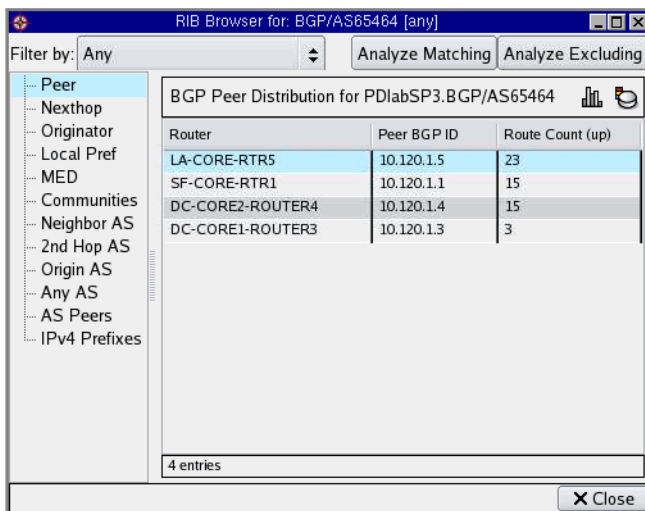
Figure 73 RIB Browser for BGP
