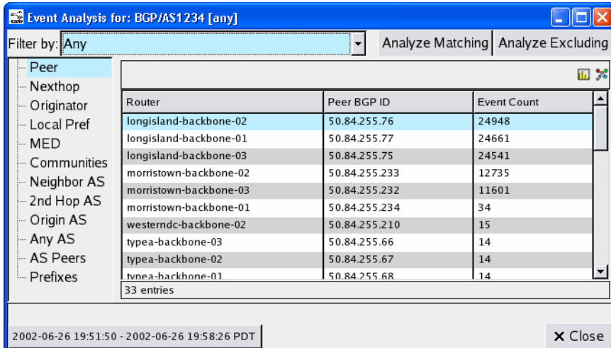
Figure 87 Event Analysis Window
