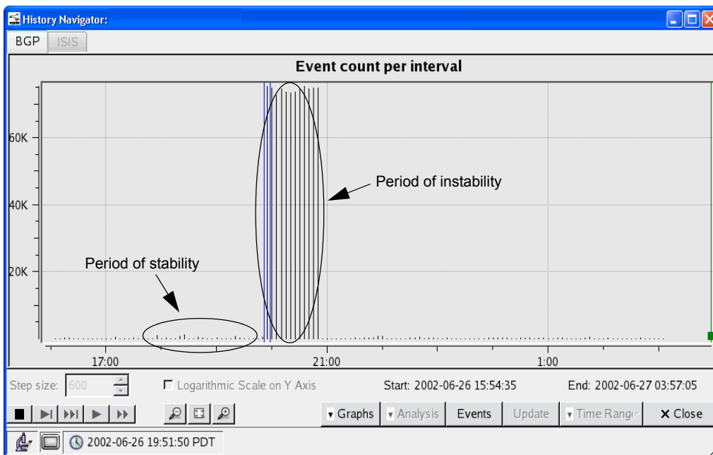
Figure 86 Stability and Instability
