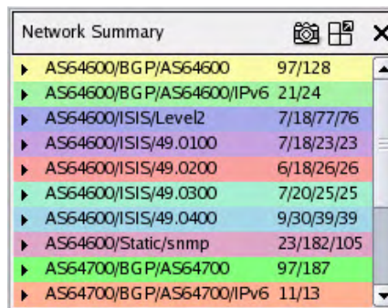
Figure 8 Network Summary Panel
