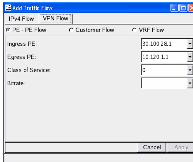
Figure 105 Add PE-PE Selection for VPN Traffic Flow
