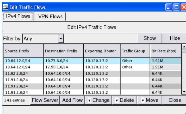
Figure 108 Edit Traffic Flows
