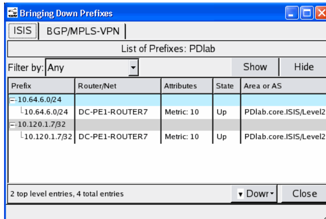
Figure 114 Bringing Down Prefixes
