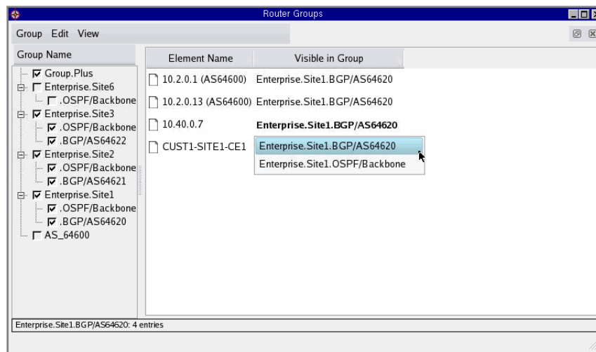
Figure 50 Changing Router Group Visibility
