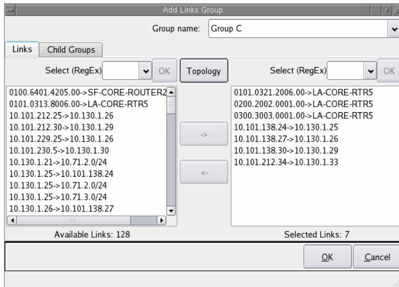
Figure 47 Creating a New Group
