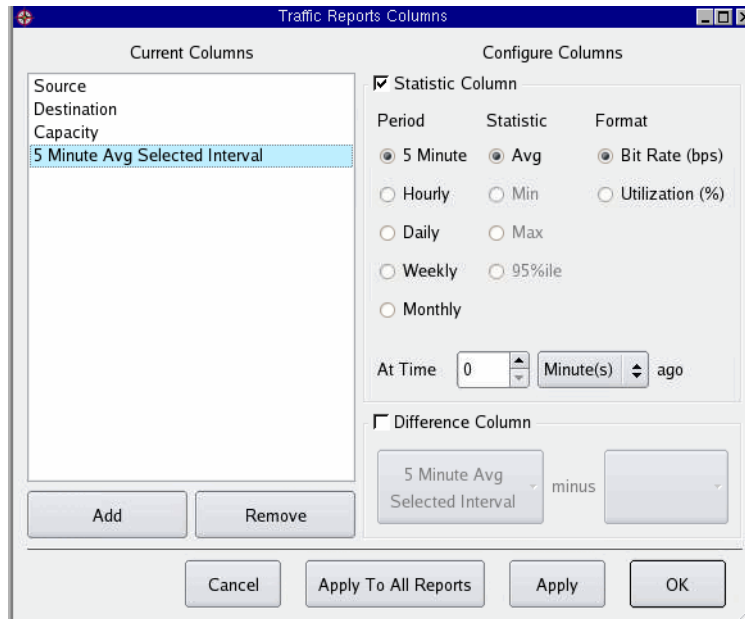
Figure 136 Traffic Reports Columns
