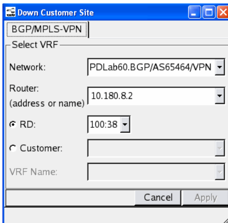
Figure 115 Down Customer Site
