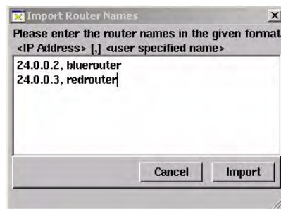
Figure 29 Import Router Names Dialog B
