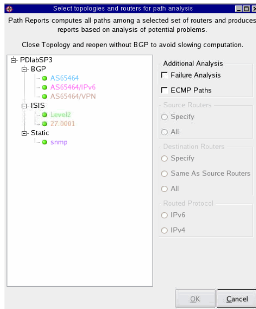
Figure 146 Path Reports - Select Topology
