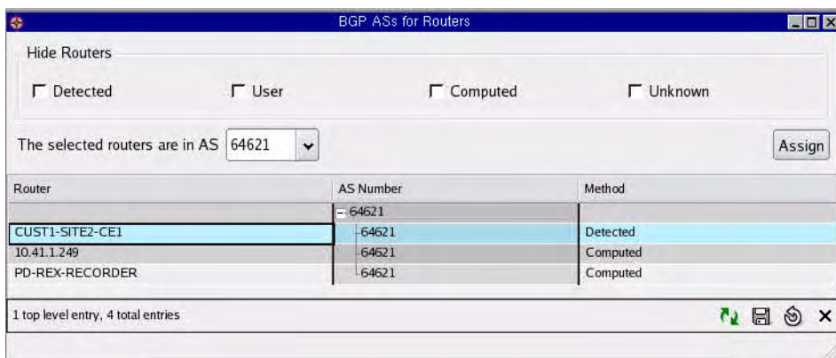
Figure 63 BGP AS to Routers
