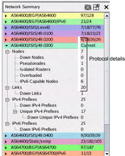
Figure 9 Network Summary Panel Expanded Row
