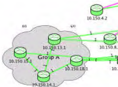
Figure 38 Viewing Elements Within a Cloud
