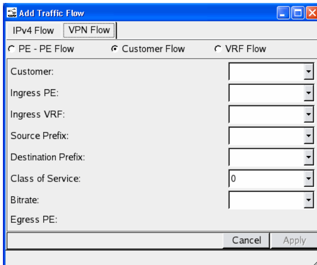
Figure 106 Add Customer Flow Selection for VPN Traffic Flow
