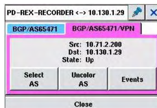
Figure 19 Link Information Panel
