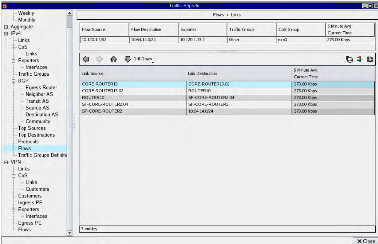
Figure 138 Example of Drill-Down to Identify BGP Flows on a Link
