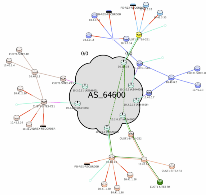
Figure 156 Paths Connecting Multiple Sites
