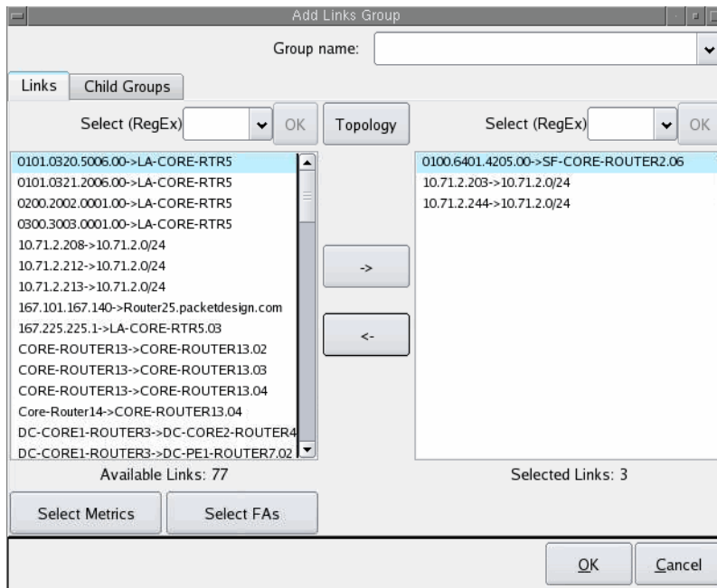
Figure 53 Link Group - Select FA Option
