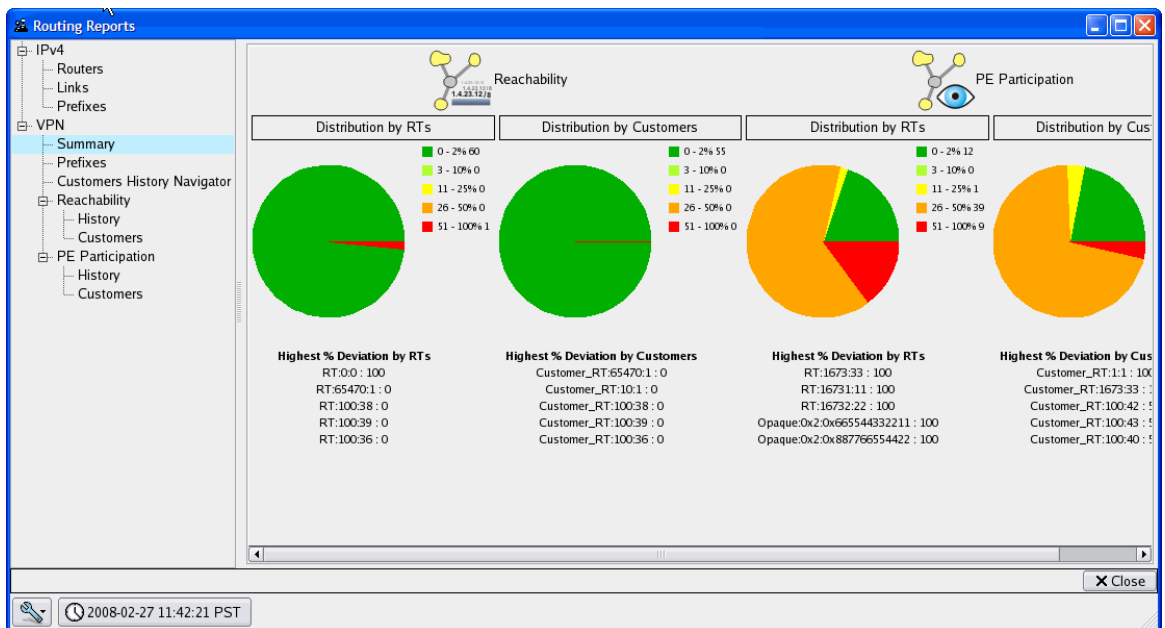
Figure 128 VPN Summary Report
