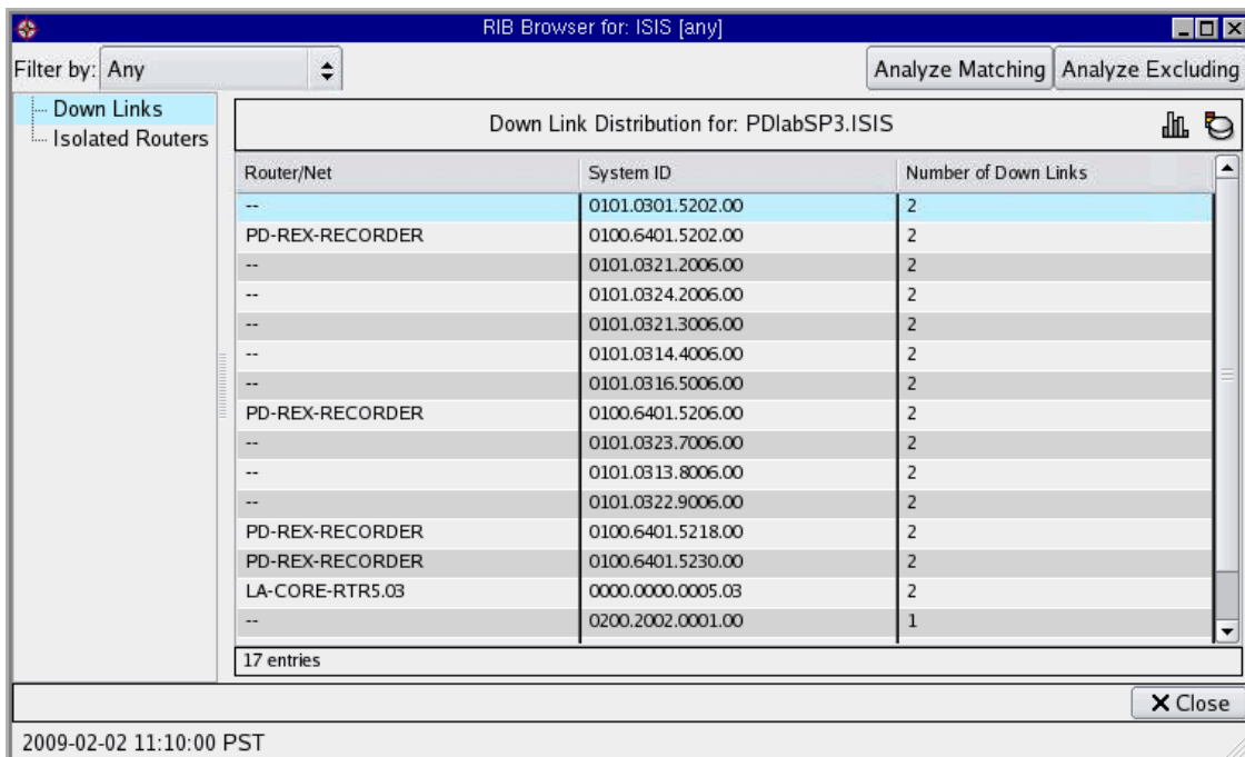
Figure 72 RIB Browser for IGP
