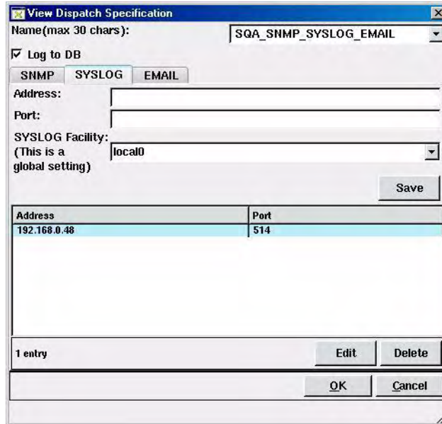
Figure 171 Defining a Syslog Dispatch Specification
