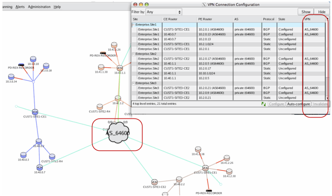
Figure 155 VPN Connection Configuration After Auto-Configuration
