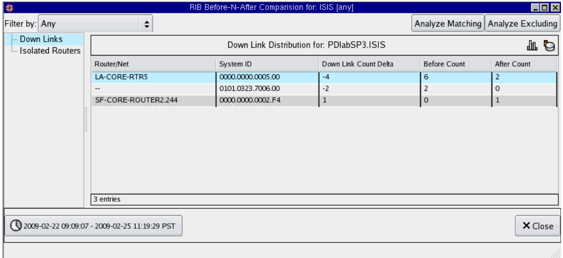
Figure 75 RIB Comparison for IGP
