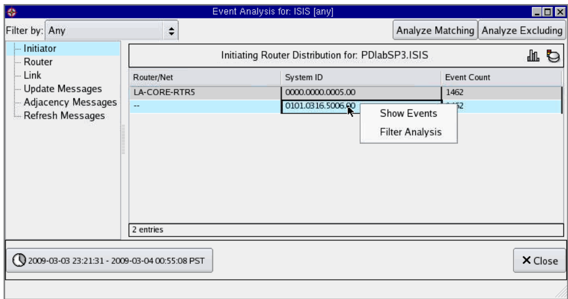
Figure 81 Event Analysis for IGP
