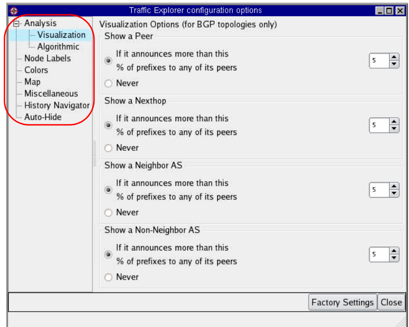
Figure 16 Configuration Options Window
