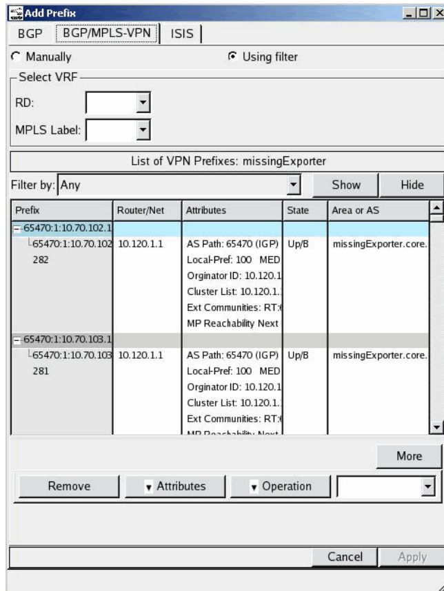
Figure 101 Using Filters Radio Button
