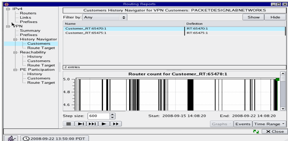
Figure 130 VPN Customers History
