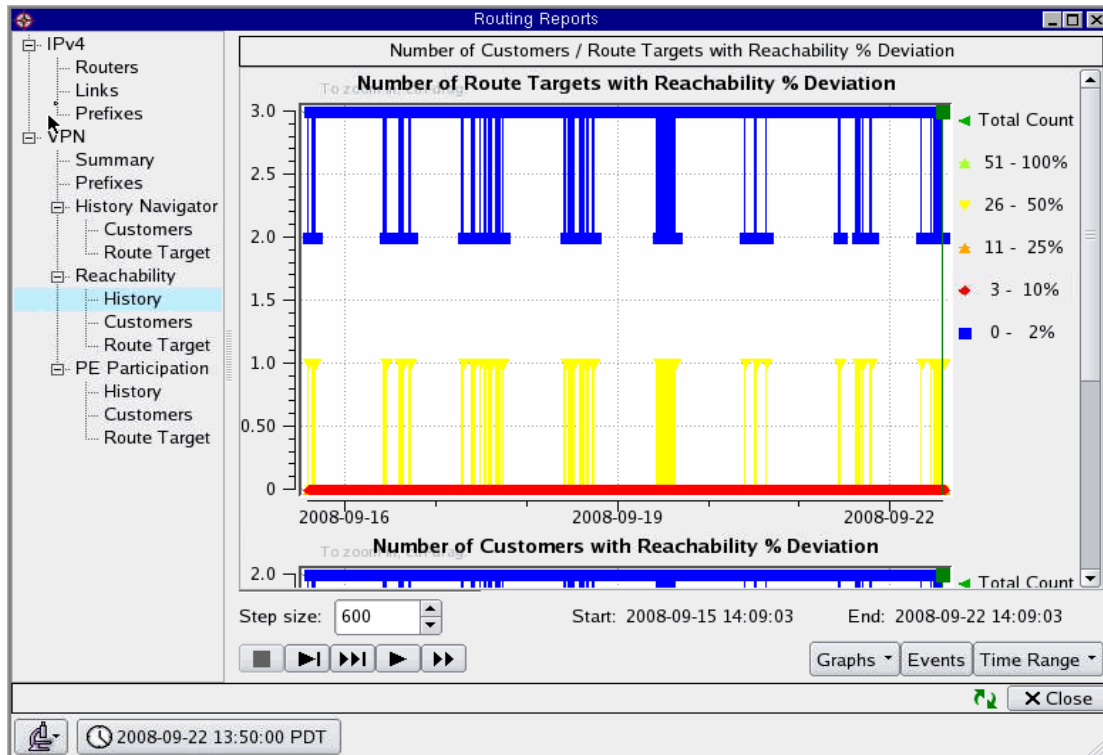
Figure 131 VPN Reachability History Report
