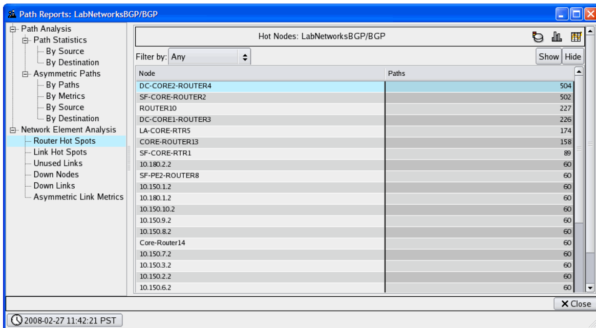
Figure 151 Router Hot Spots Table
