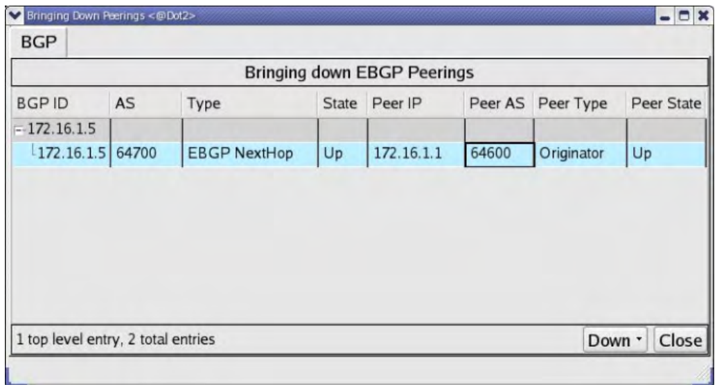
Figure 113 Bringing Down Peerings
