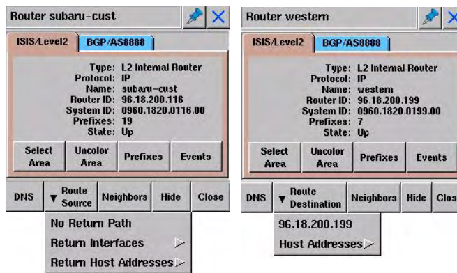
Figure 54 Source and Destination Node Information Panels
