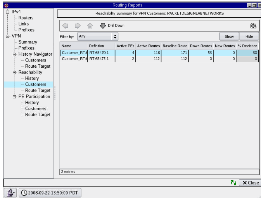
Figure 132 VPN Reachability History Report
