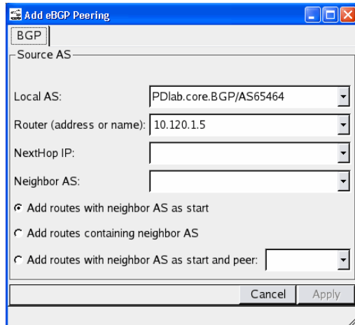
Figure 99 Add eBGP Peering
