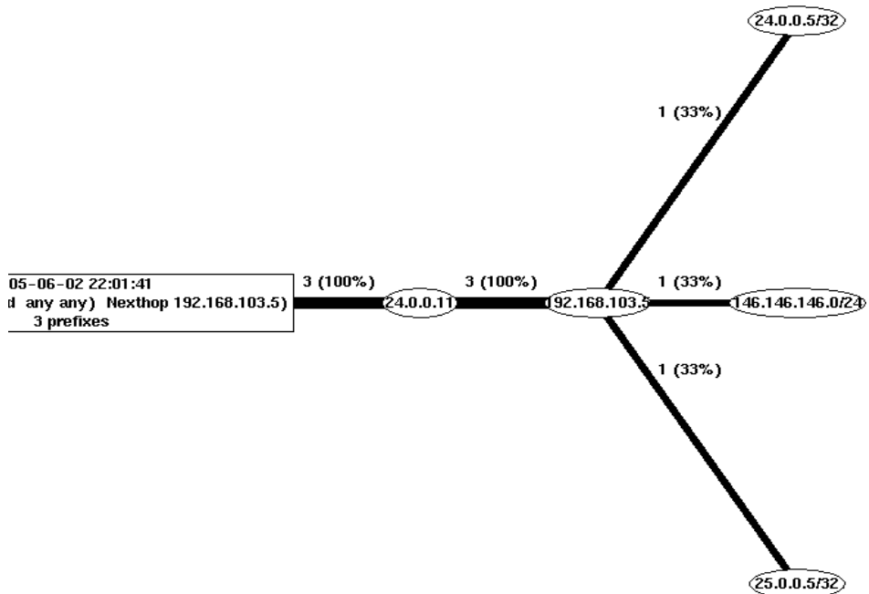
Figure 70 RIB Visualization with Show an Edge to a Prefix Option
