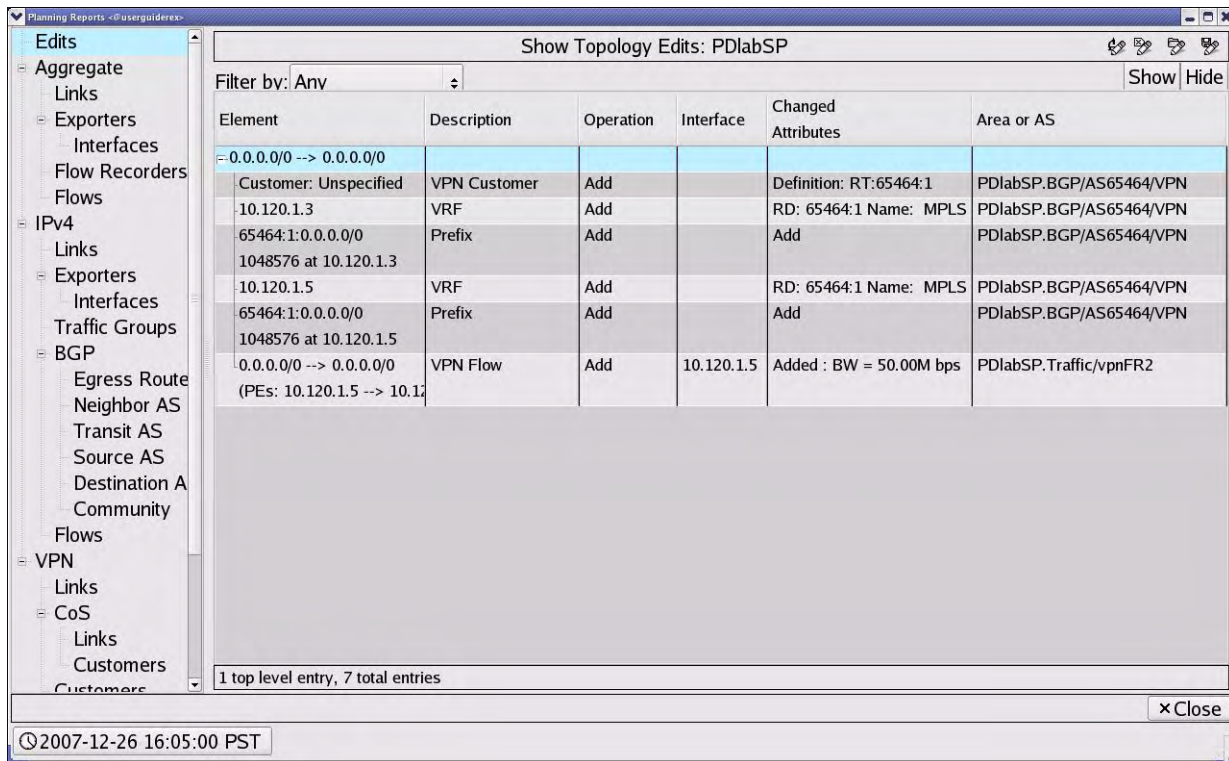
Figure 116 Show Topology Edits Window
