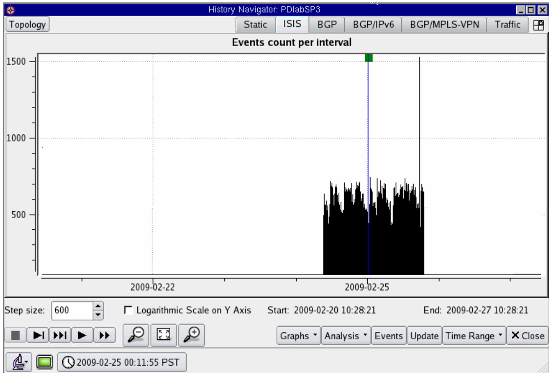
Figure 74 Large Number of Events in Short Space of Time
