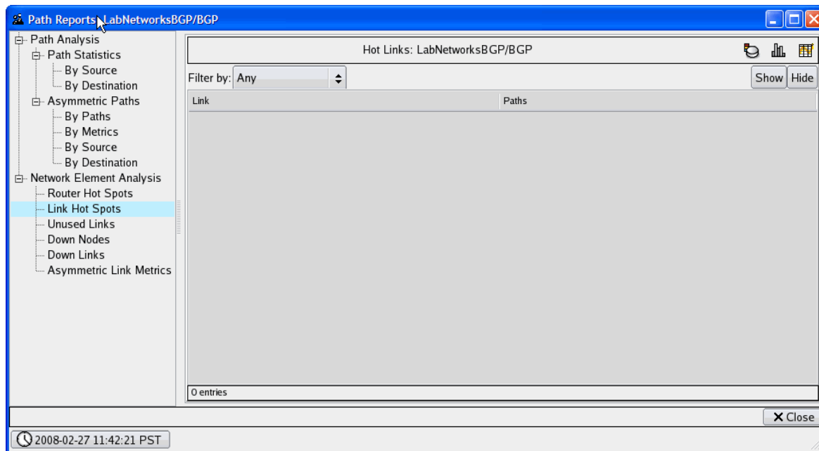
Figure 152 Link Hot Spots Table
