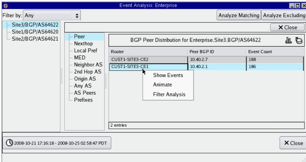
Figure 82 Event Analysis for BGP
