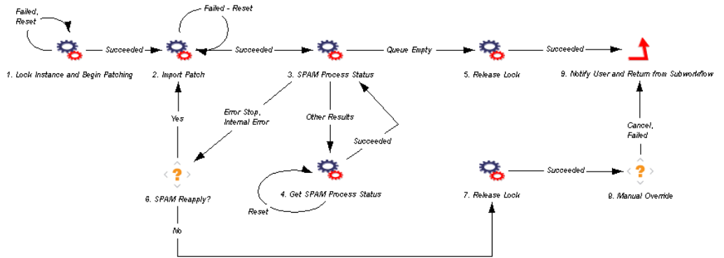
Figure 4-26. SAP - SPAM Update Subworkflow
