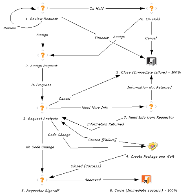
Figure 4-18. SAP - Bug/Enhancement Workflow
