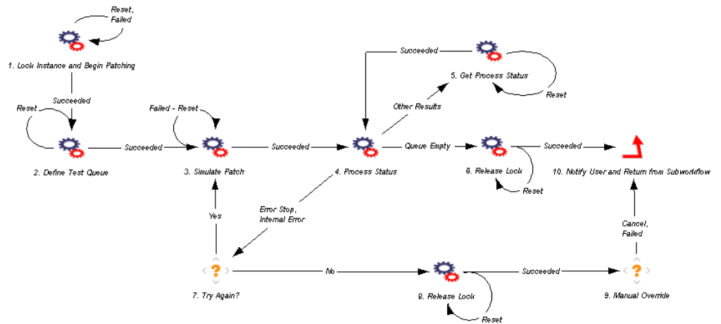
Figure 4-27. SAP - Patch Simulation Subworkflow
