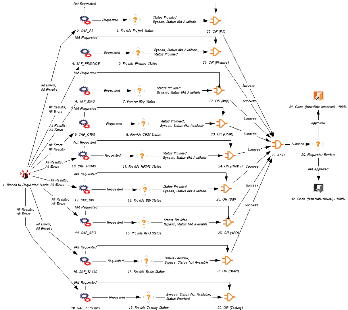
Figure 4-30. SAP - Status Update Req workflow
