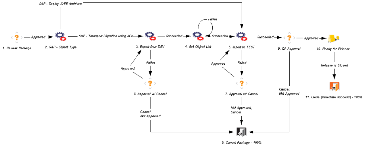
Figure 4-31. SAP - Transport and J2EE Deployments workflow
