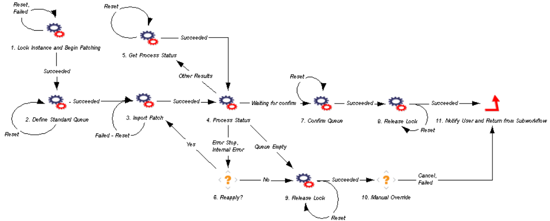
Figure 4-28. SAP - Patch Application Subworkflow
