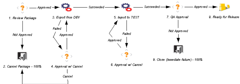
Figure 4-32. SAP - Transport Migration with Release Management workflow
