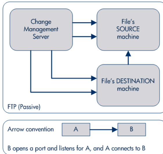
Figure 7-3. FTP (passive)
