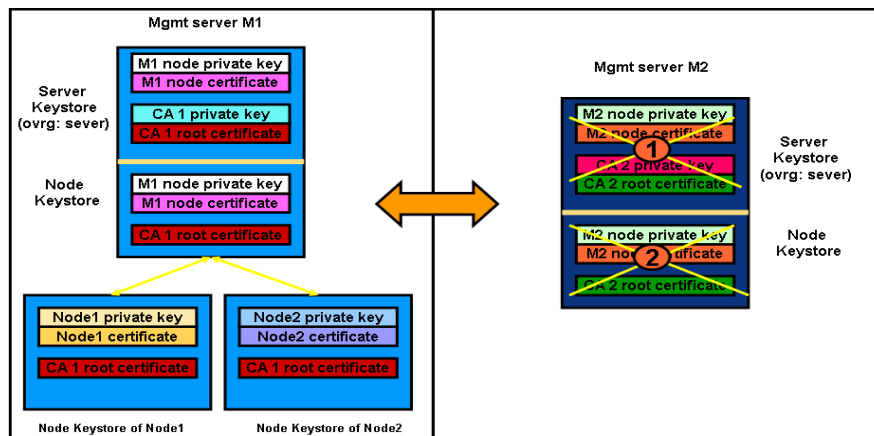
Figure 3-5 Removing Certificates from the M2 Management Server
