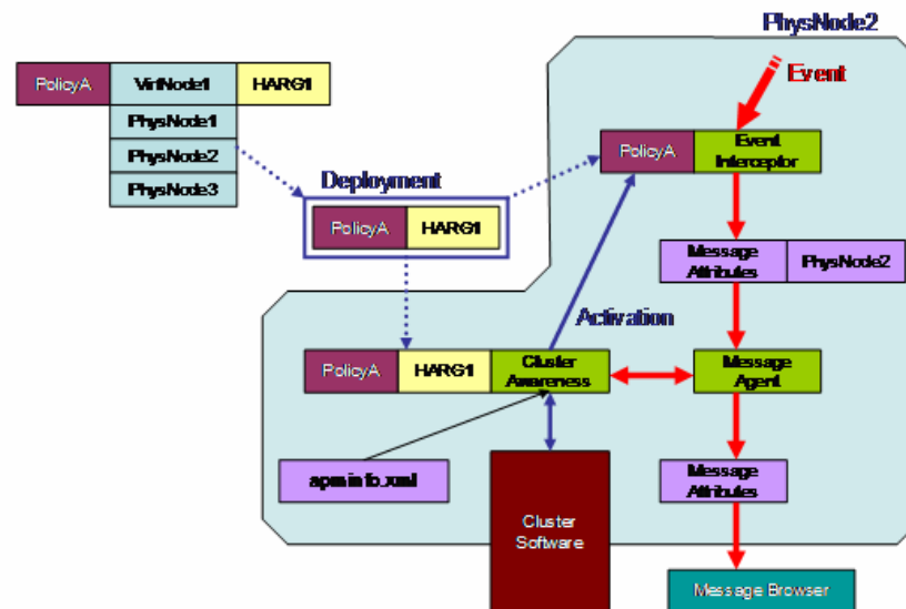
Figure 7-3 Virtual Node Concept with ClAw
