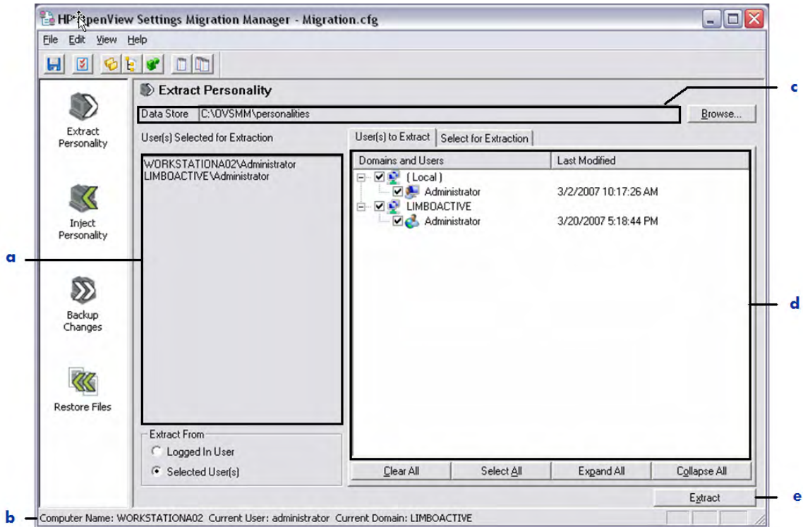
Figure 8 Extract Personality view
