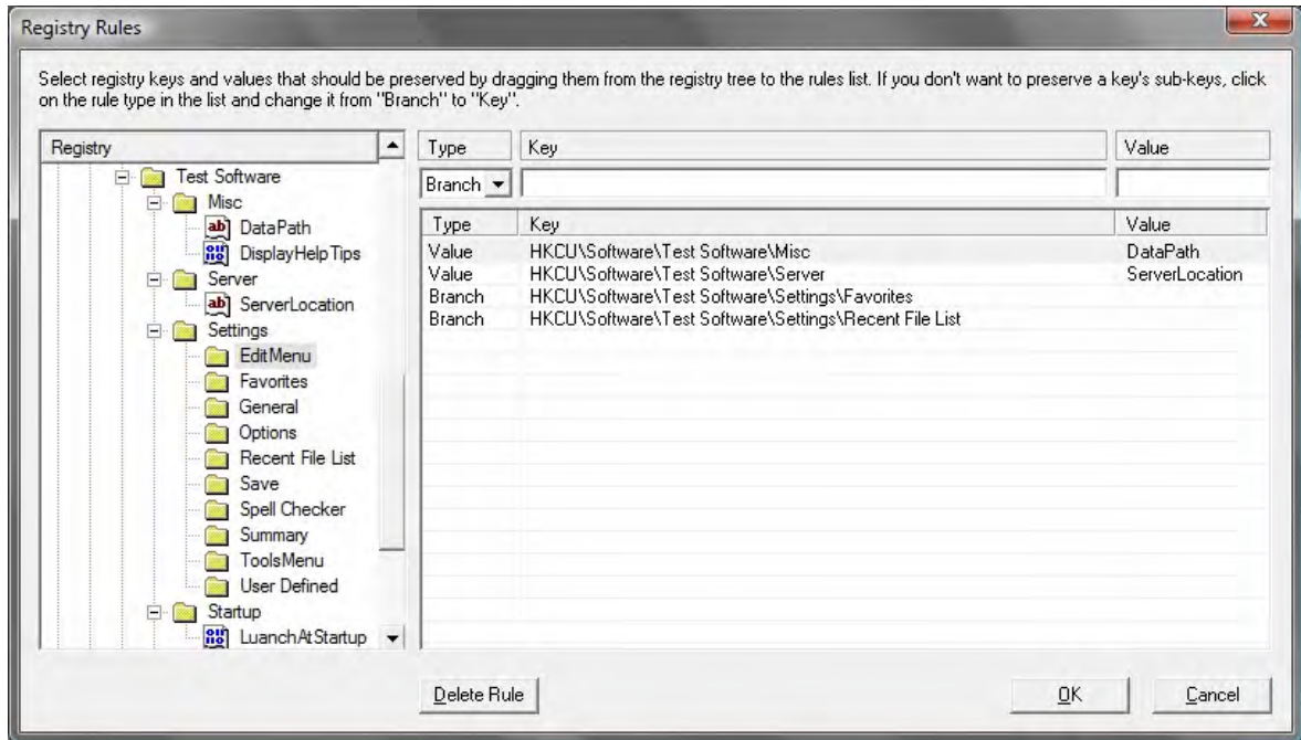
Figure 27 Registry rule definitions
