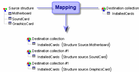
Figure 4.16. Field-to-collection mapping
