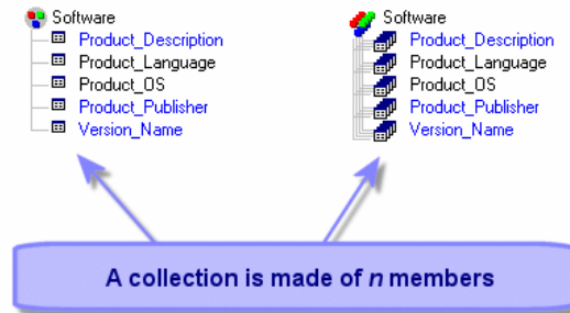
Figure 4.14. Collection
