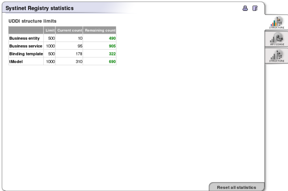
Figure 183. Statistics - Publication Limits
