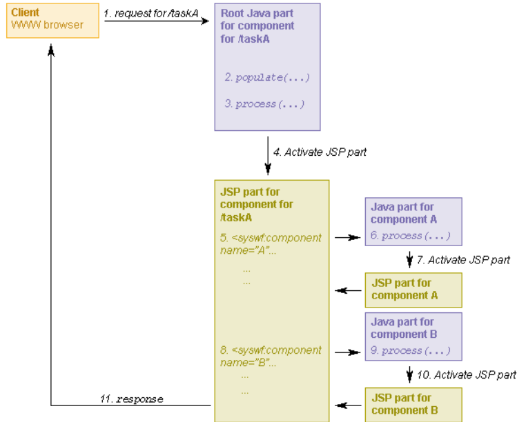
Figure 229. Nesting Components Diagram
