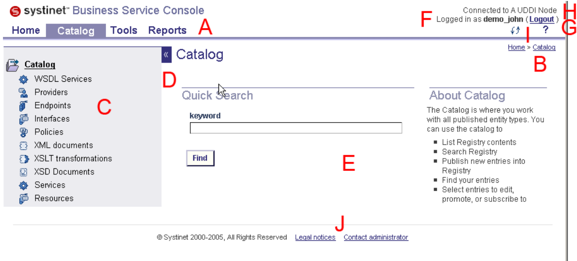
Figure 62. Example Business Service Console page
