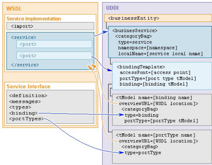
Figure 232. WSDL Mapping to UDDI
