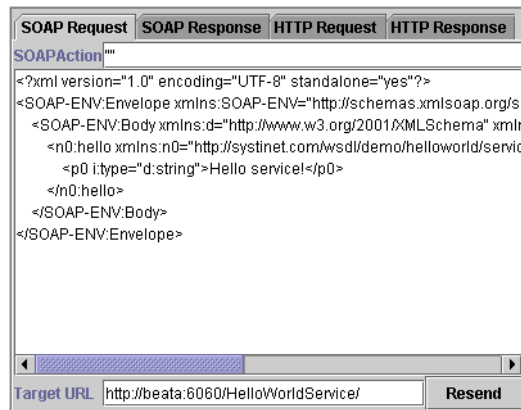
Figure 243. Request Tab
