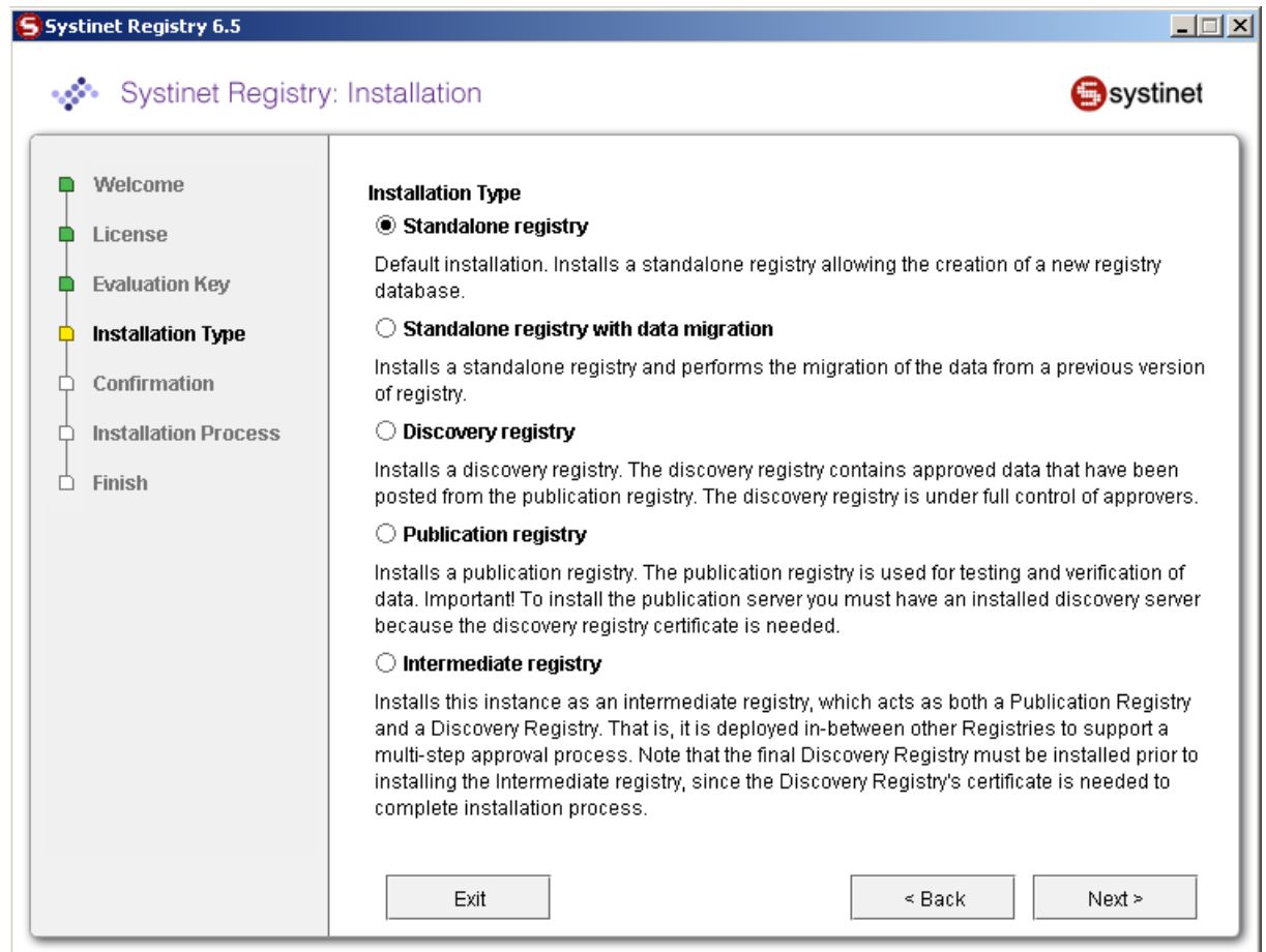
Figure 4. Installation Type
