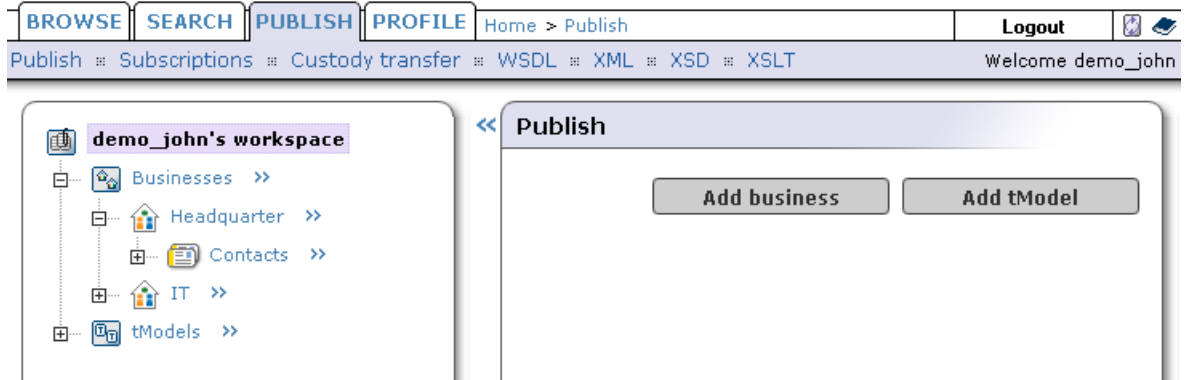
Figure 129. Add Business
