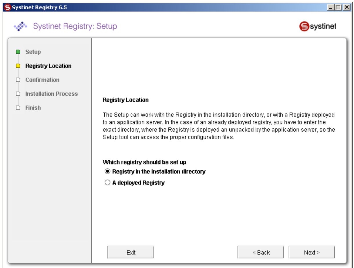
Figure 21. Setup
