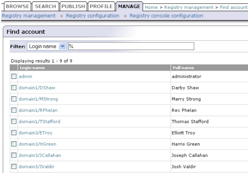
Figure 45. Registry Users
