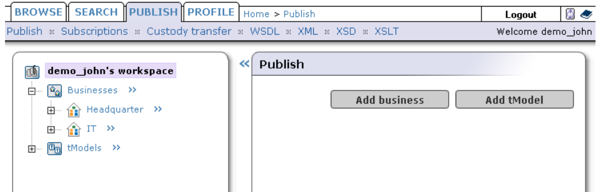
Figure 128. Publish Page
