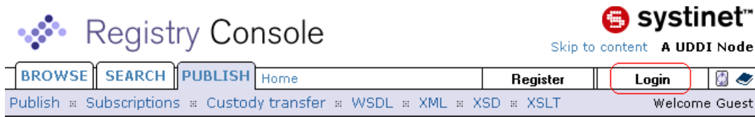
Figure 106. Login Tab
