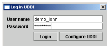
Figure 154. Login Dialog
