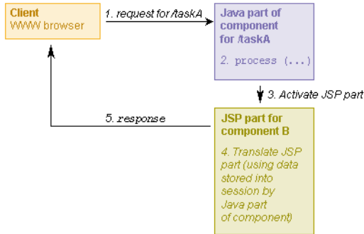
Figure 228. Request Diagram
