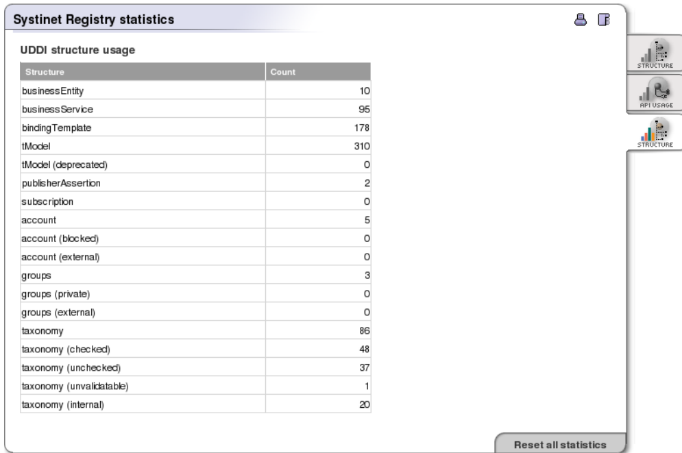
Figure 185. Statistics - Structure
