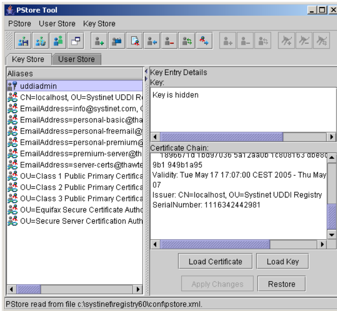
Figure 213. PStore Tool
