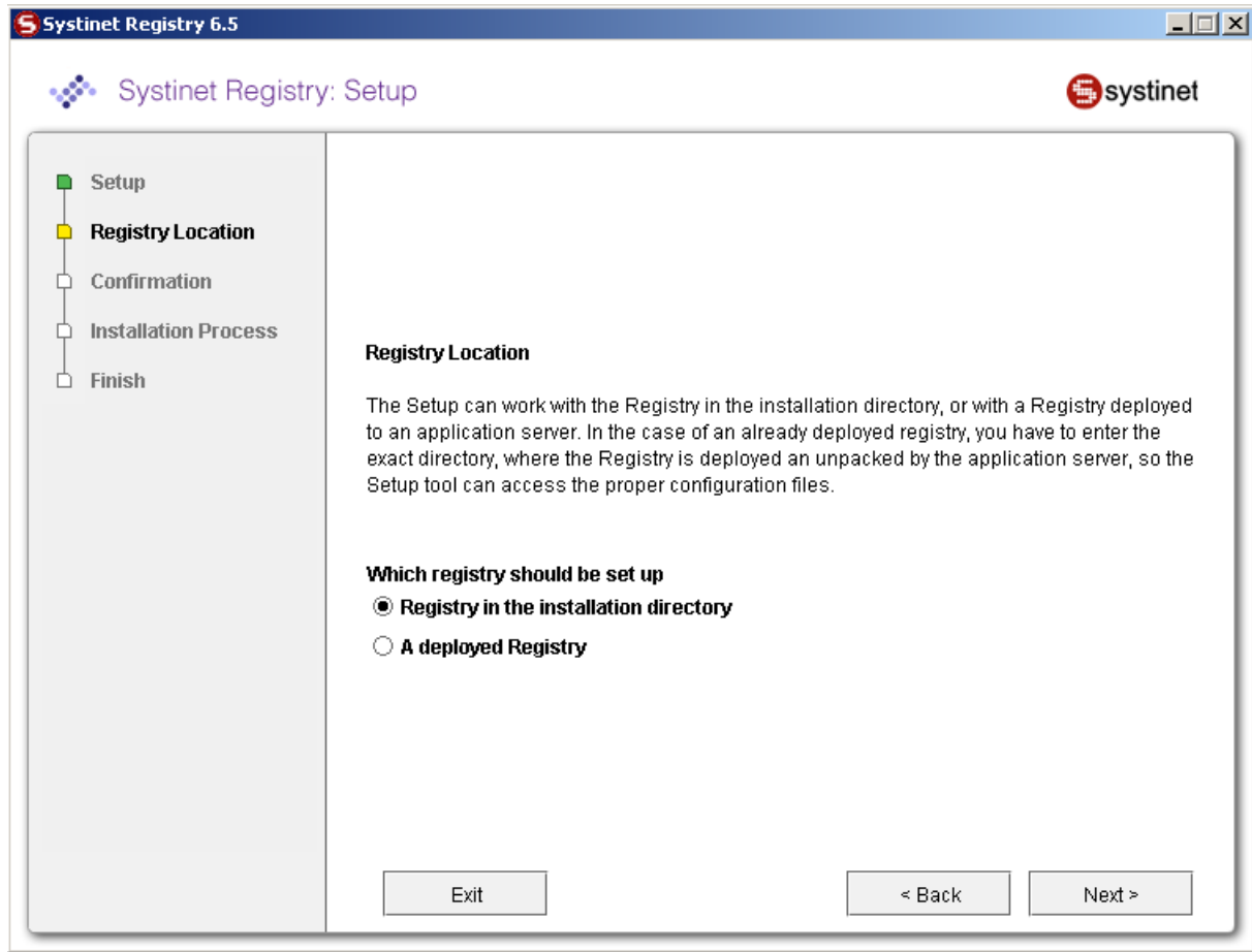
Figure 59. Setup
