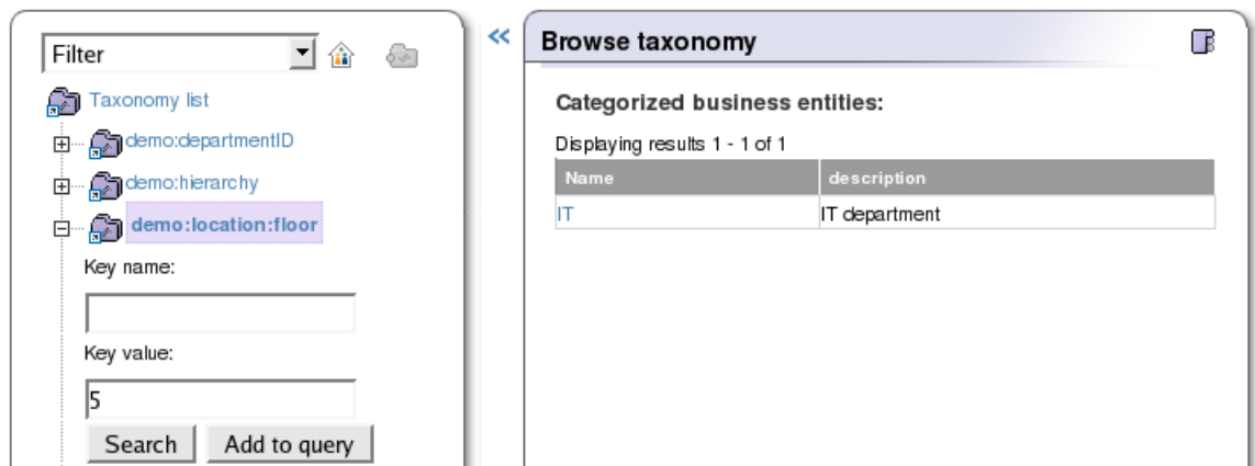
Figure 115. Browse Demo
