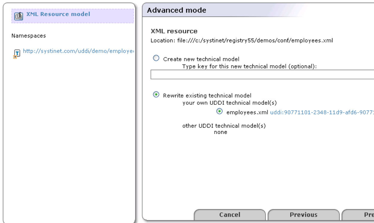
Figure 146. Publish XML Document - Advanced
