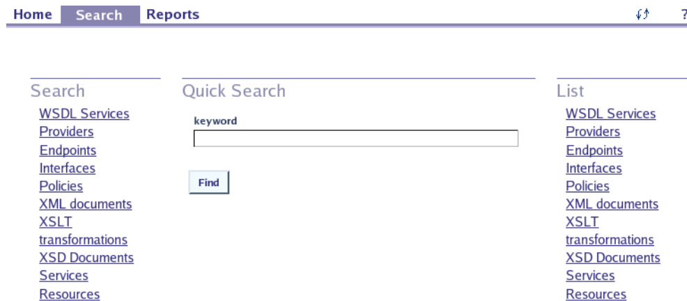
Figure 66. Search Tab
