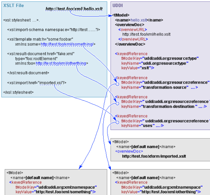
Figure 220. XSLT TO UDDI
