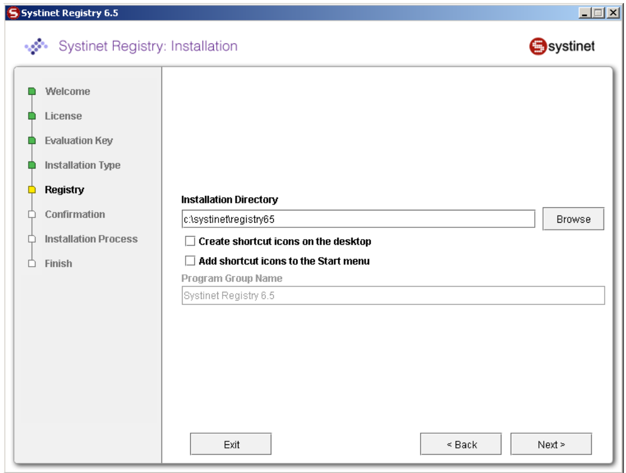
Figure 5. Installation Directory
