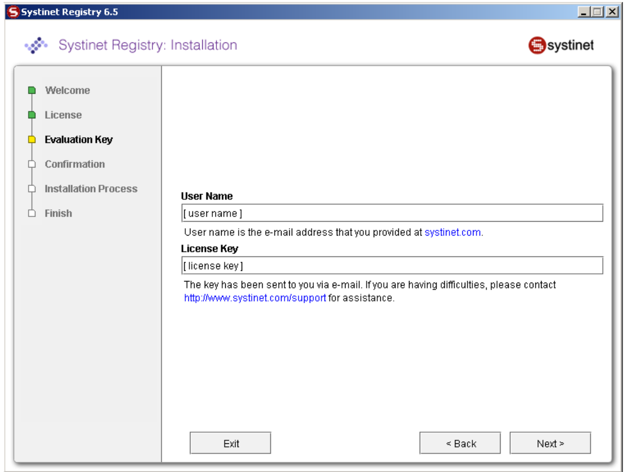
Figure 19. Evaluation Key
