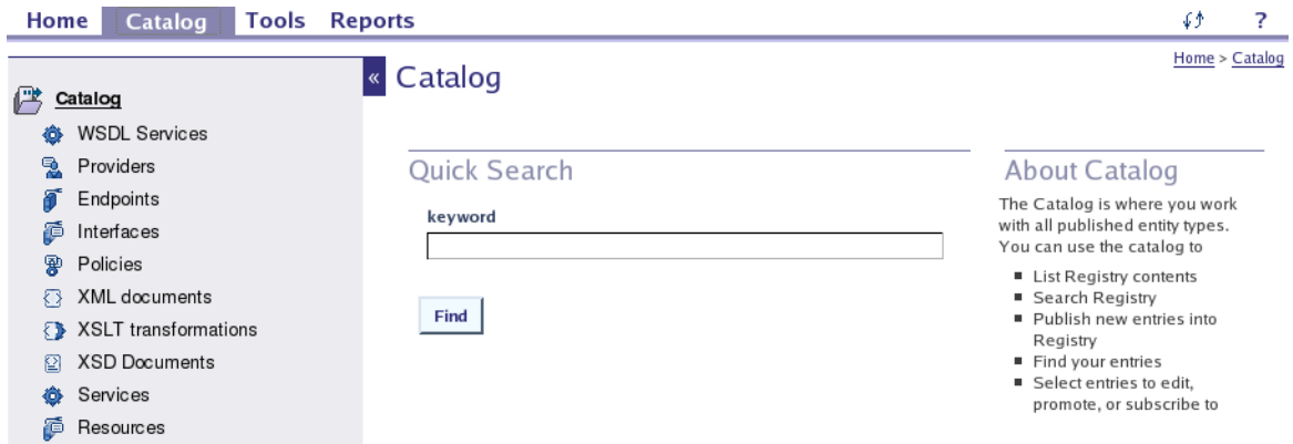
Figure 72. Catalog Tree
