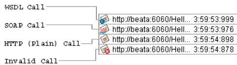
Figure 242. Call Types
