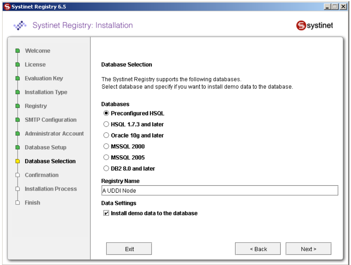
Figure 9. Select Database
