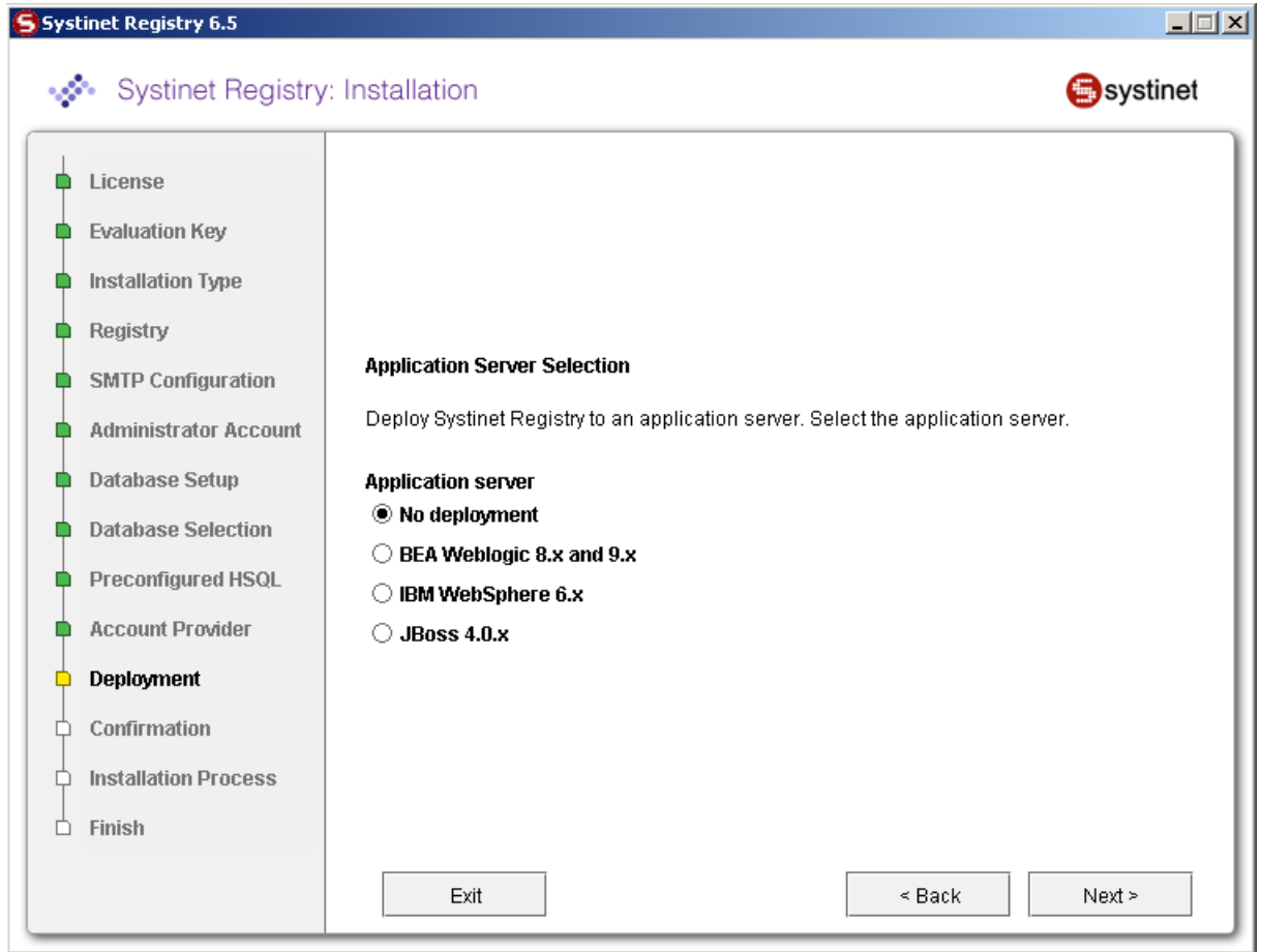
Figure 13. Direct deployment
