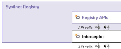
Figure 225. Registry Interceptors
