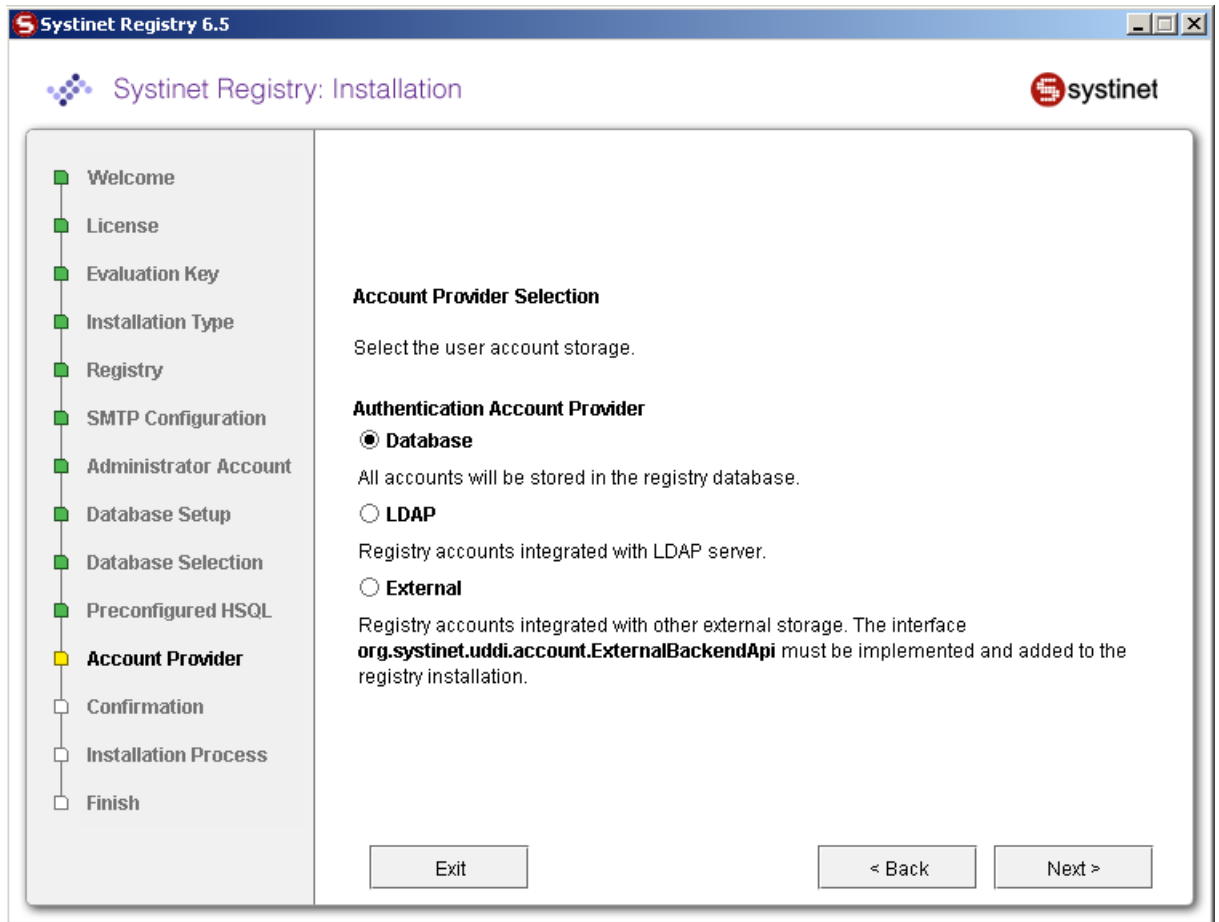
Figure 12. Authentication Provider
