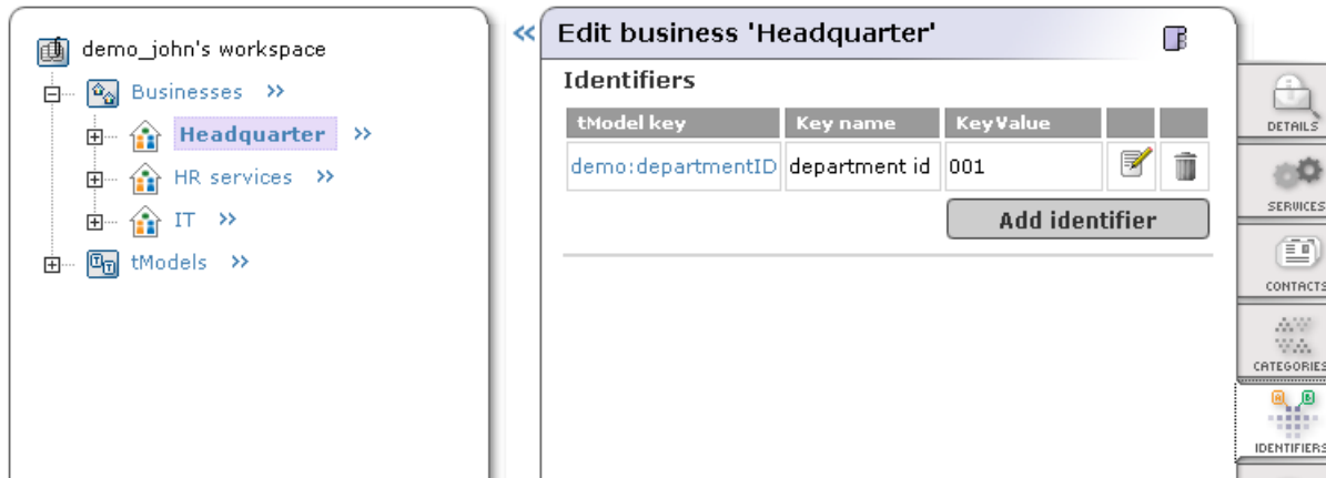
Figure 130. Edit Business
