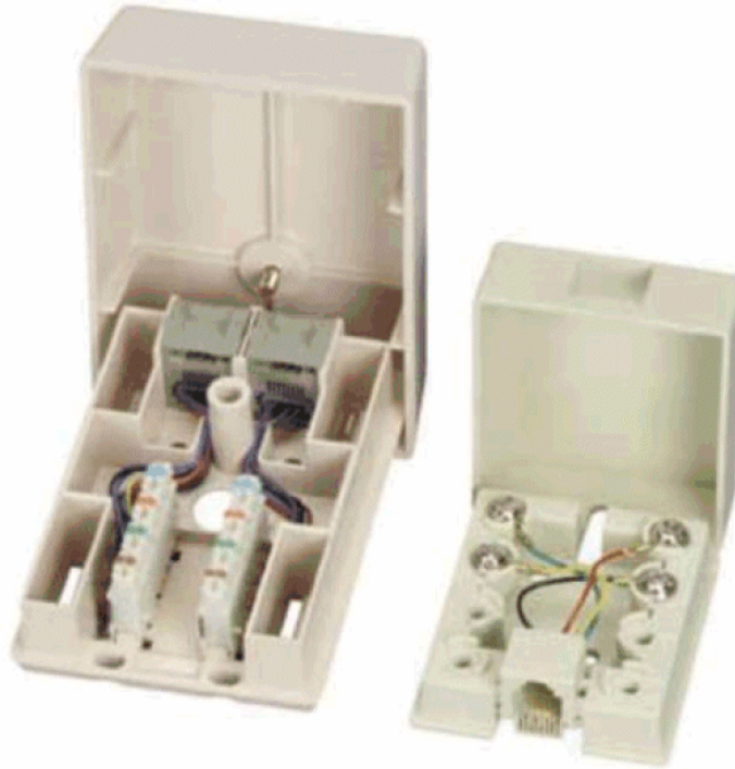
Figure 8.8. Punchdown block - photos
