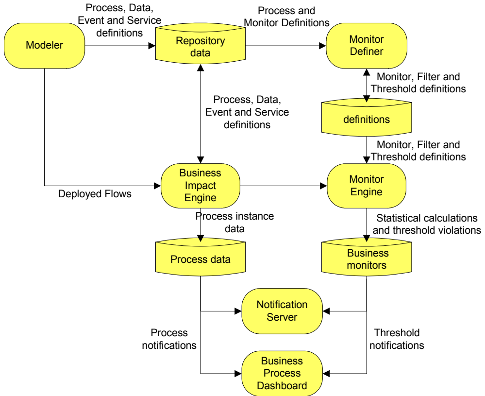
Figure 11 Process Impact and Monitor Data Relationship
