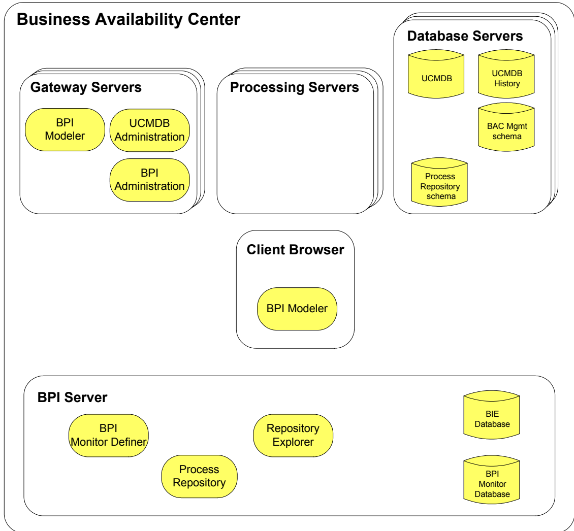
Figure 2 Design-Time - Process Instance Tracking Enabled
