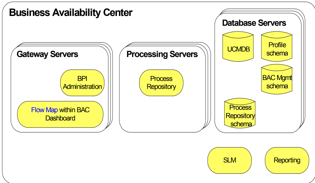
Figure 3 Run-Time - Process Instance Tracking Disabled
