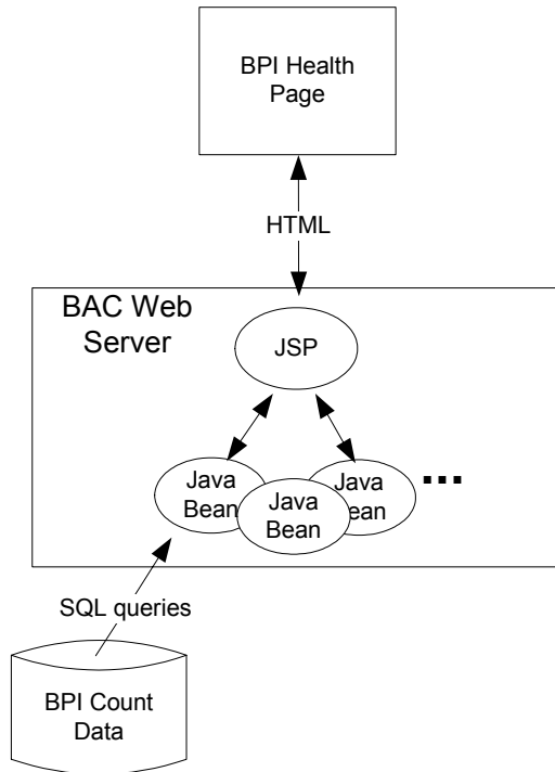
Figure 30 Health Page Count Data
