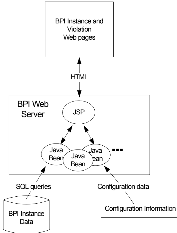
Figure 31 Instance and Violation Information
