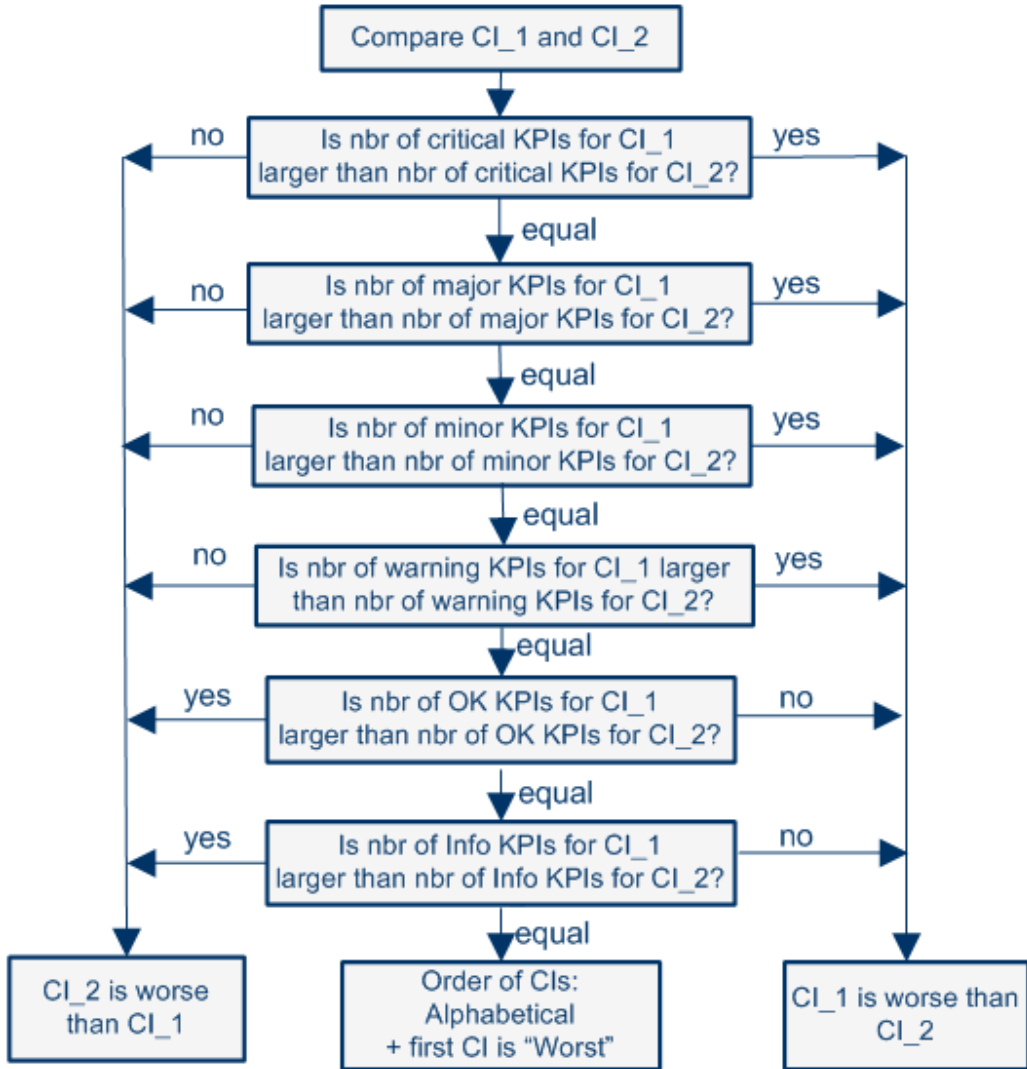
Figure 19 Scorecard Sorting Process
