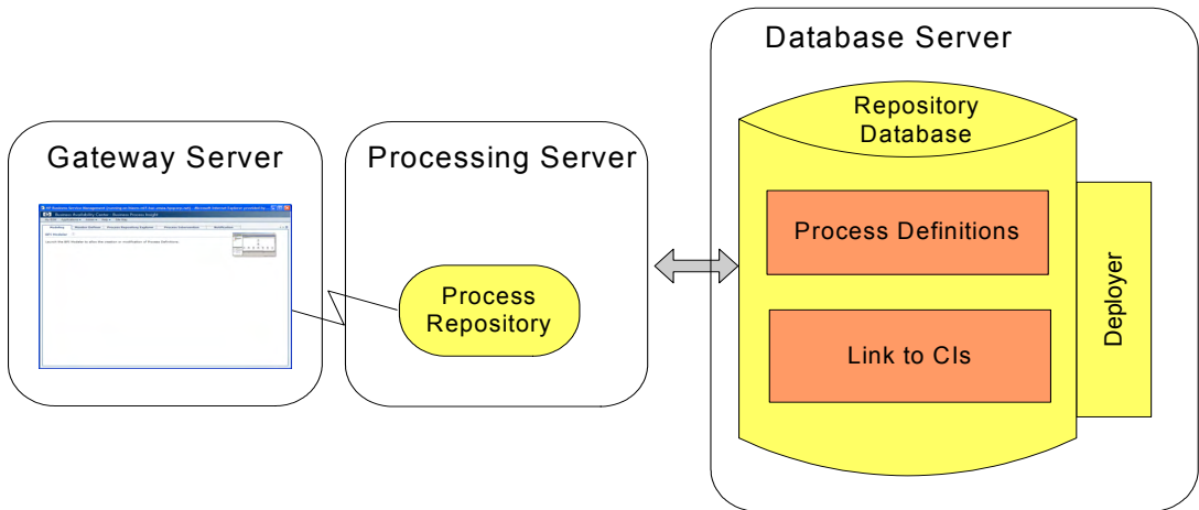
Figure 7 BPI Modeler
