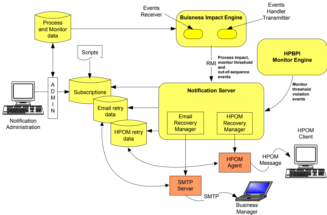
Figure 16 Notification Server
