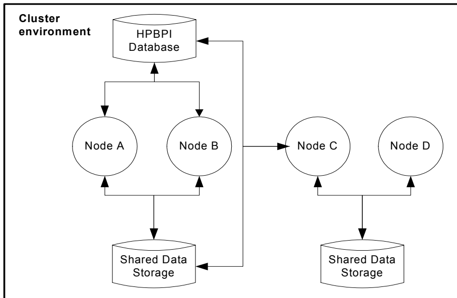
Figure 47 BPI Operating on Three Nodes in a Cluster
