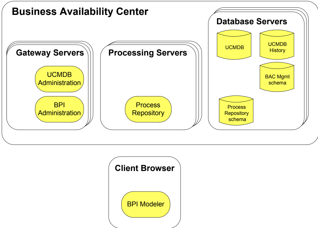
Figure 1 Design-Time - Process Instance Tracking Disabled
