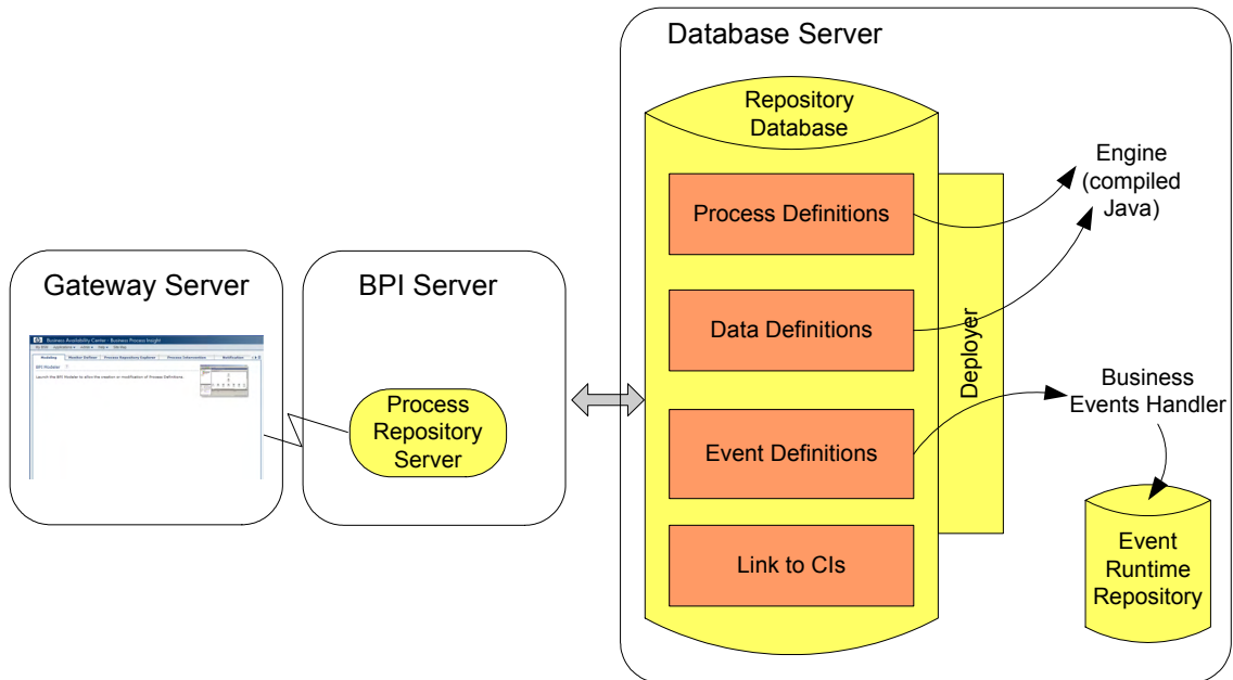
Figure 8 BPI Modeler when the BPI Server is Installed
