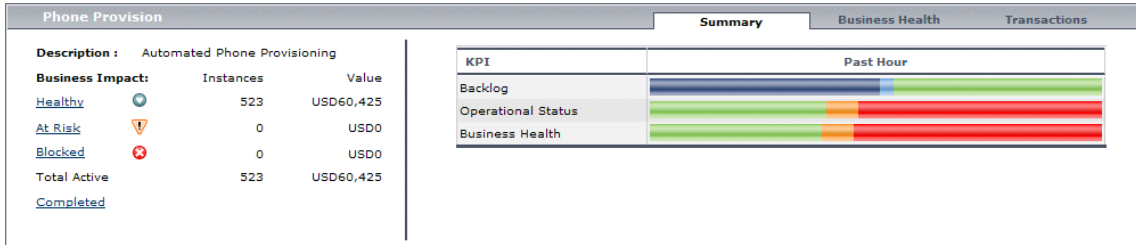
Figure 22 Summary Tab
