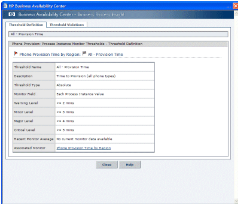
Figure 29 Monitor Threshold Dialog
