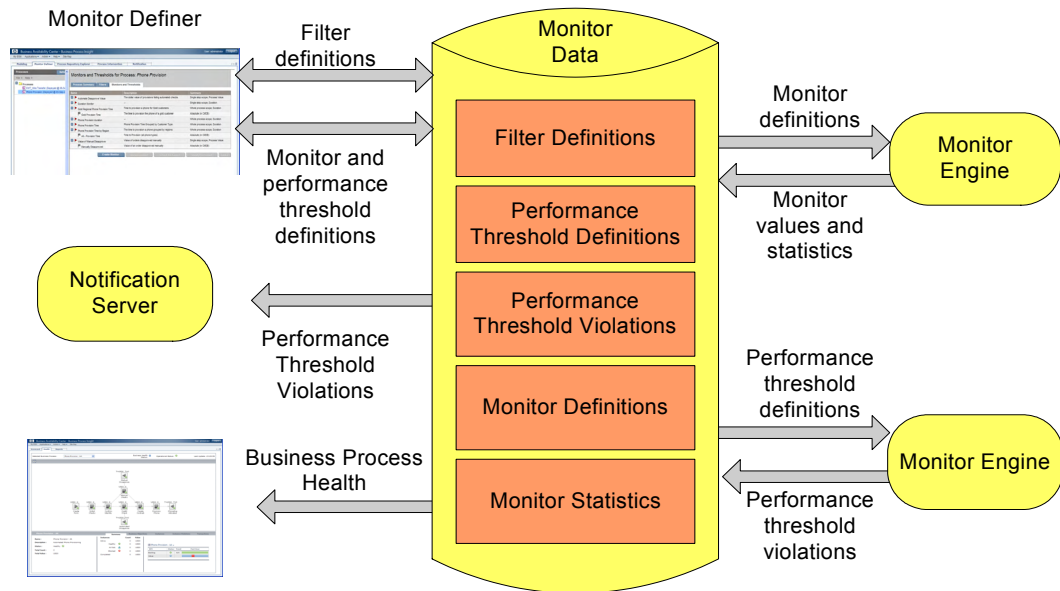
Figure 12 BPI Business Process Monitor Engine
