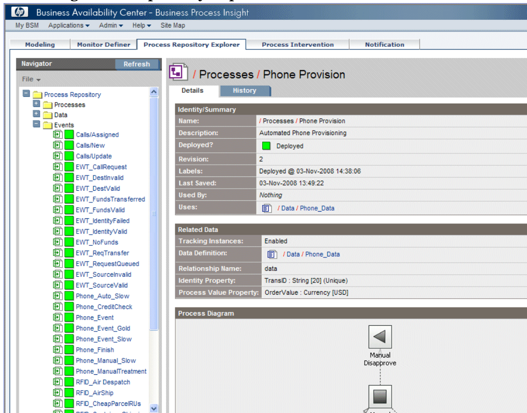
Figure 15 Repository Explorer GUI
