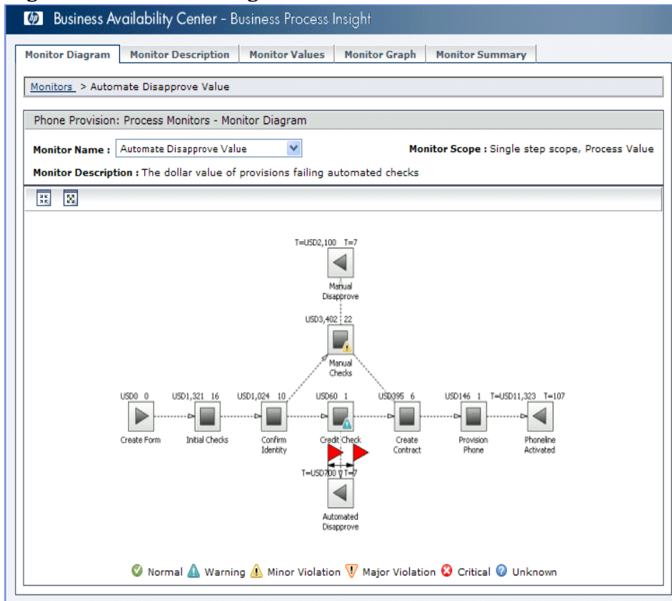
Figure 28 Monitor Dialog
