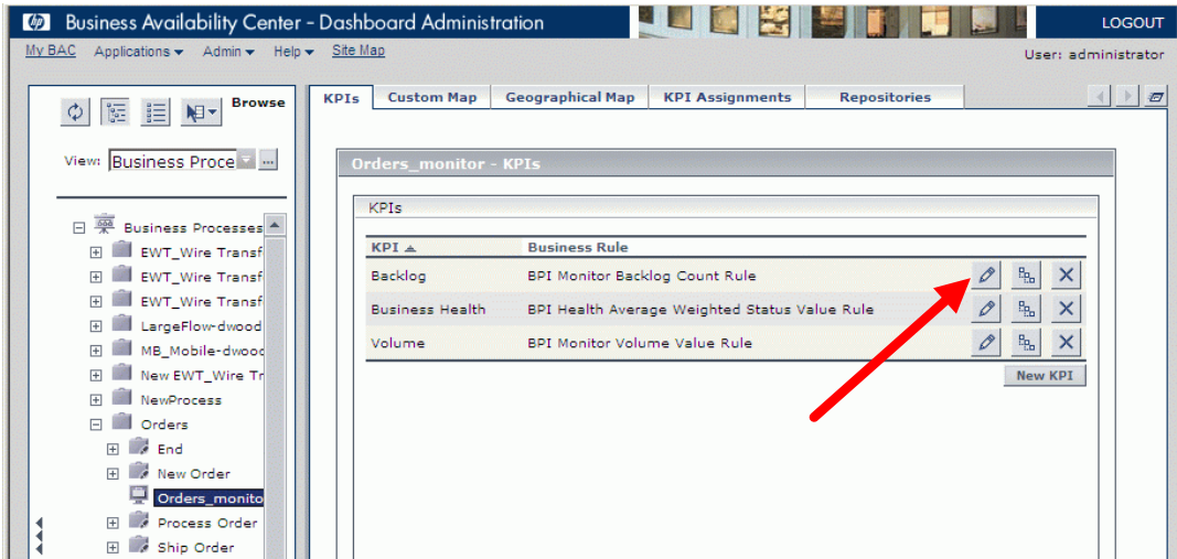
Figure 6 Switching KPIs
