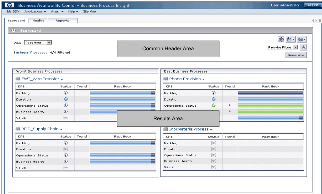
Figure 18 Scorecard Structure
