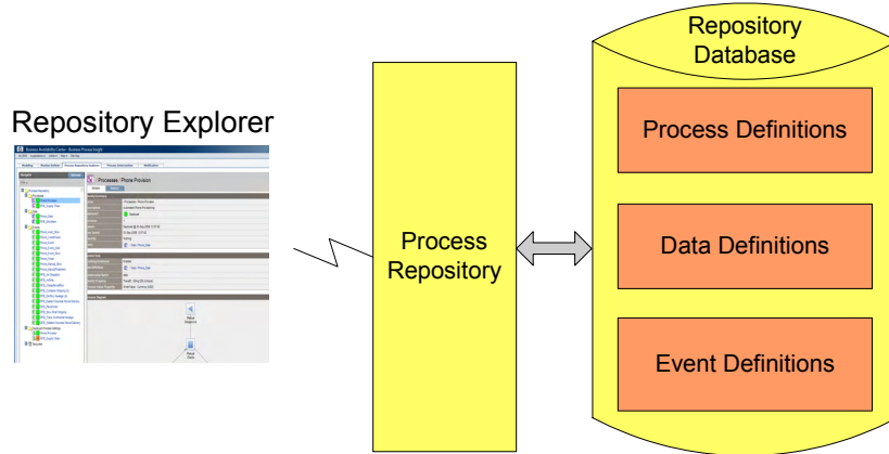
Figure 14 Repository Explorer
