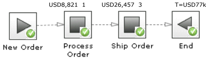
Figure 38 Process Diagram
