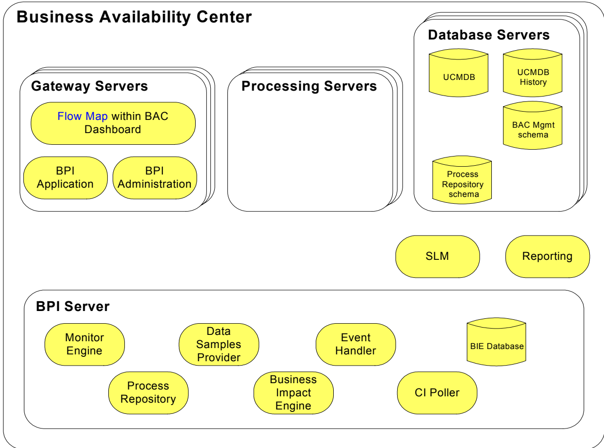
Figure 4 Run-Time - Process Instance Tracking Enabled
