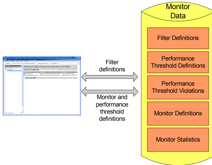
Figure 10 BPI Business Process Monitor Definer
