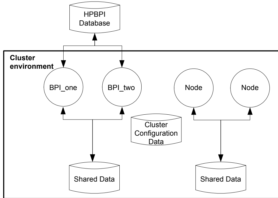
Figure 48 Cluster Licensing
