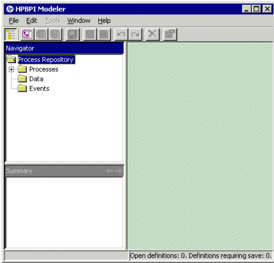
Figure 9 Modeler GUI
