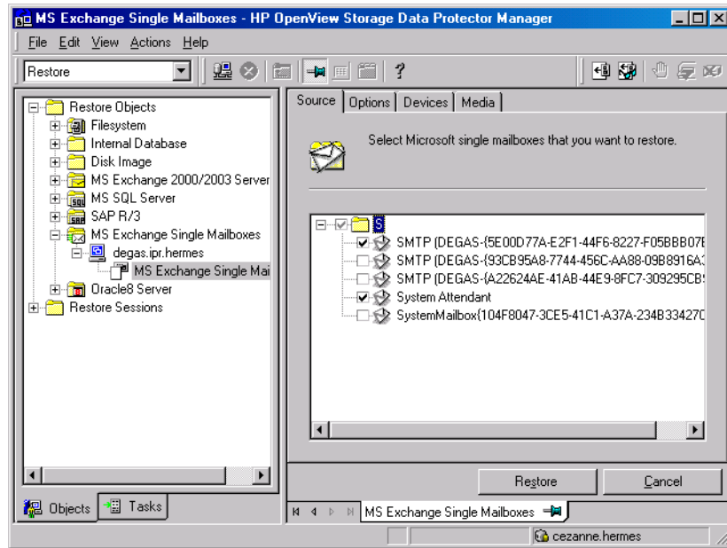
Figure 4-9 Restore Objects
