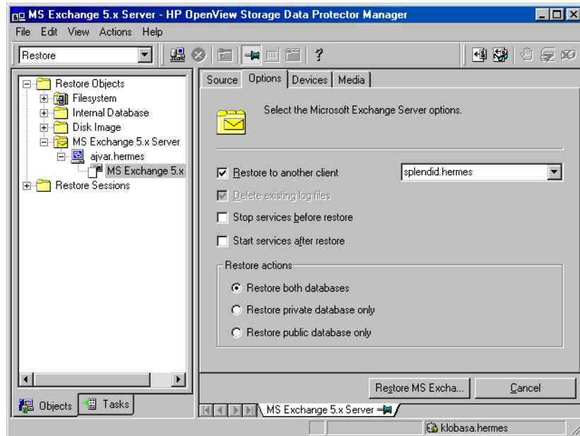
Figure 2-12 Restore Options
