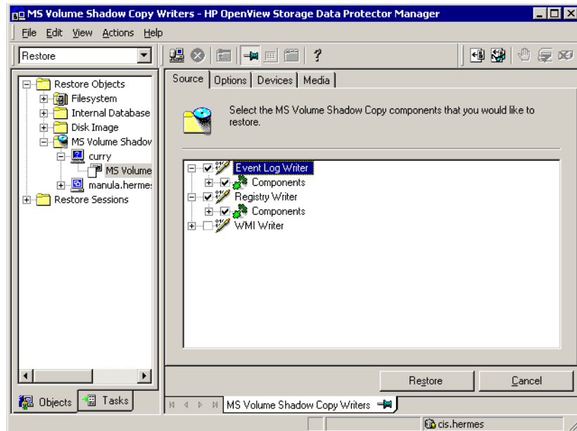
Figure 5-8 Restore Objects
