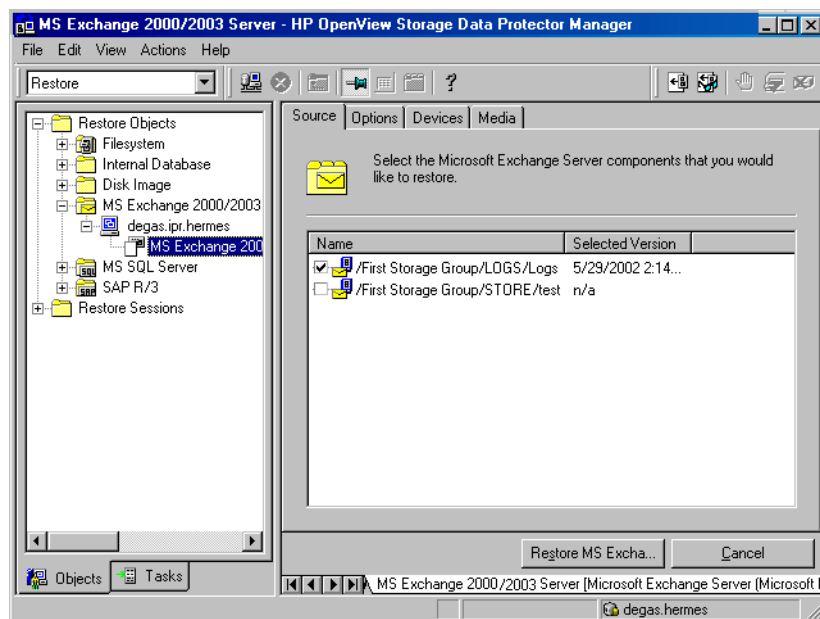
Figure 3-10 Restore Objects
