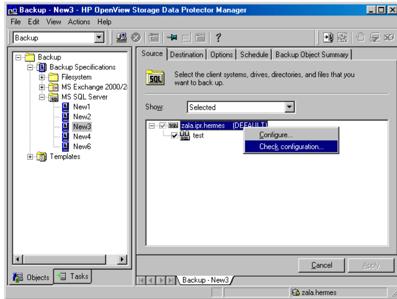
Figure 1-5 Checking Configuration
