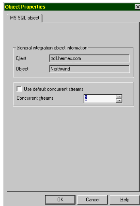
Figure 1-10 Object Properties
