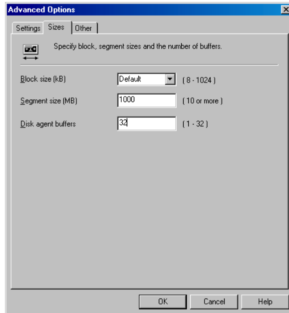
Figure 1-16 Advanced Options
