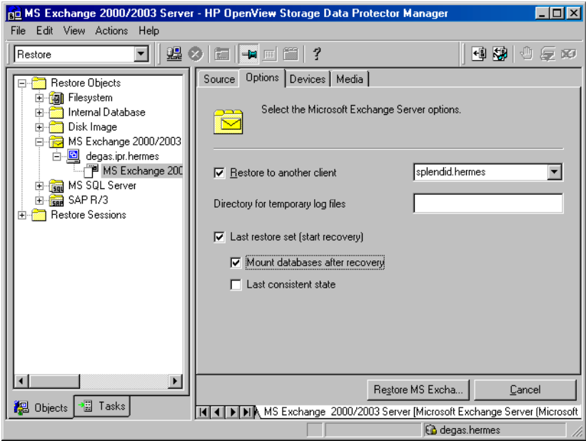
Figure 3-12 Restore Options
