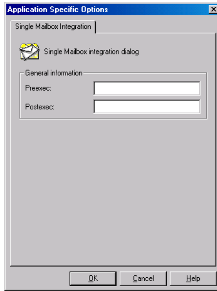
Figure 4-6 Backup Options
