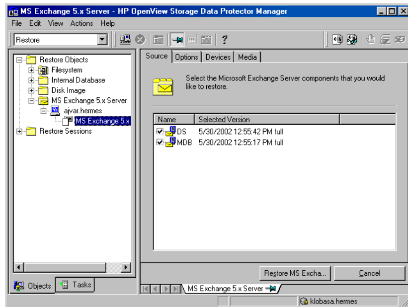
Figure 2-10 Restore Objects
