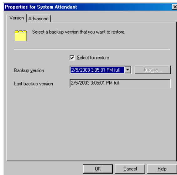
Figure 4-10 Version Properties
