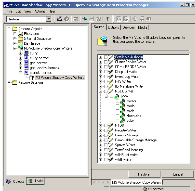
Figure 5-9 MSDE writer
