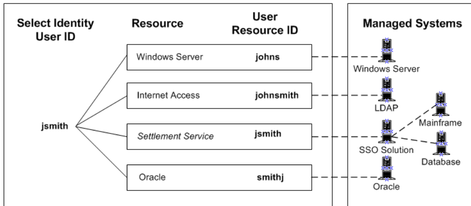
Figure 9 Select Identity Linking Example
