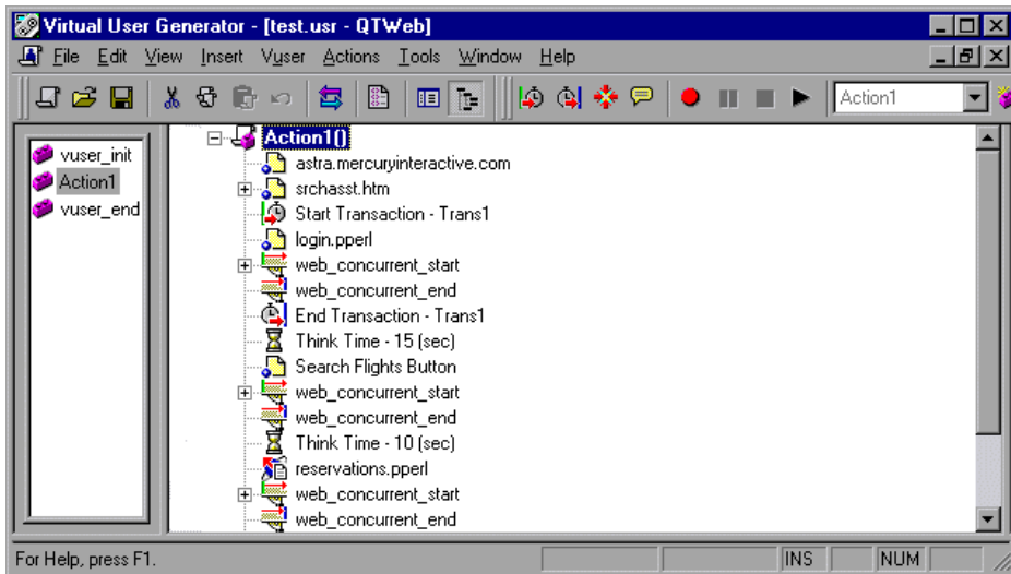
Tree view of a Web Vuser script
