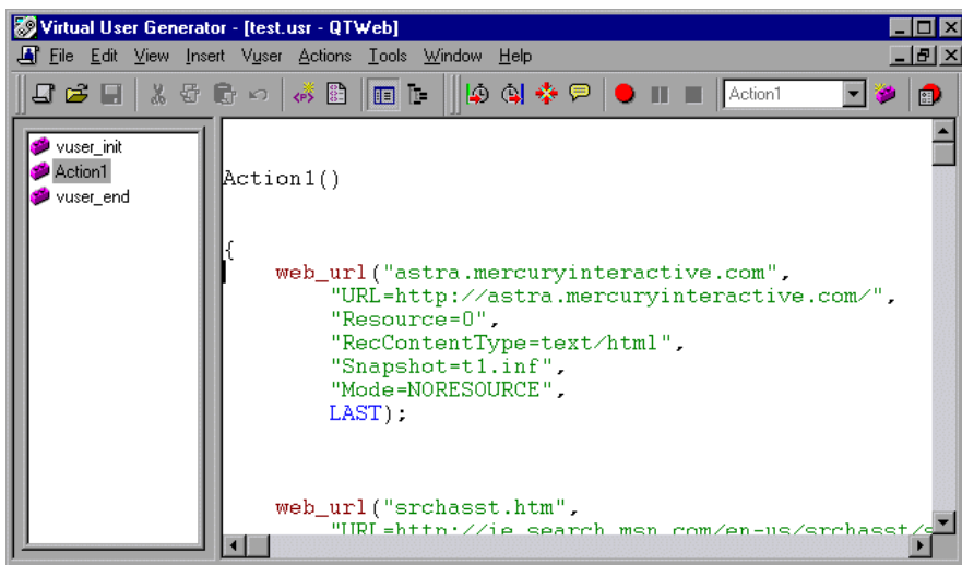
Script view of a Web Vuser script
