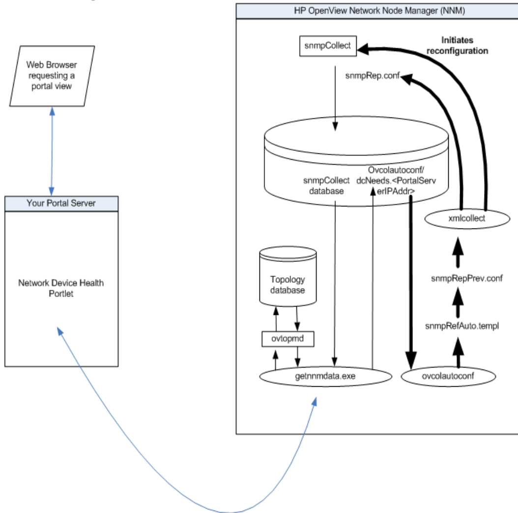
Figure 3 Communication Process for the Network Health Portlet
