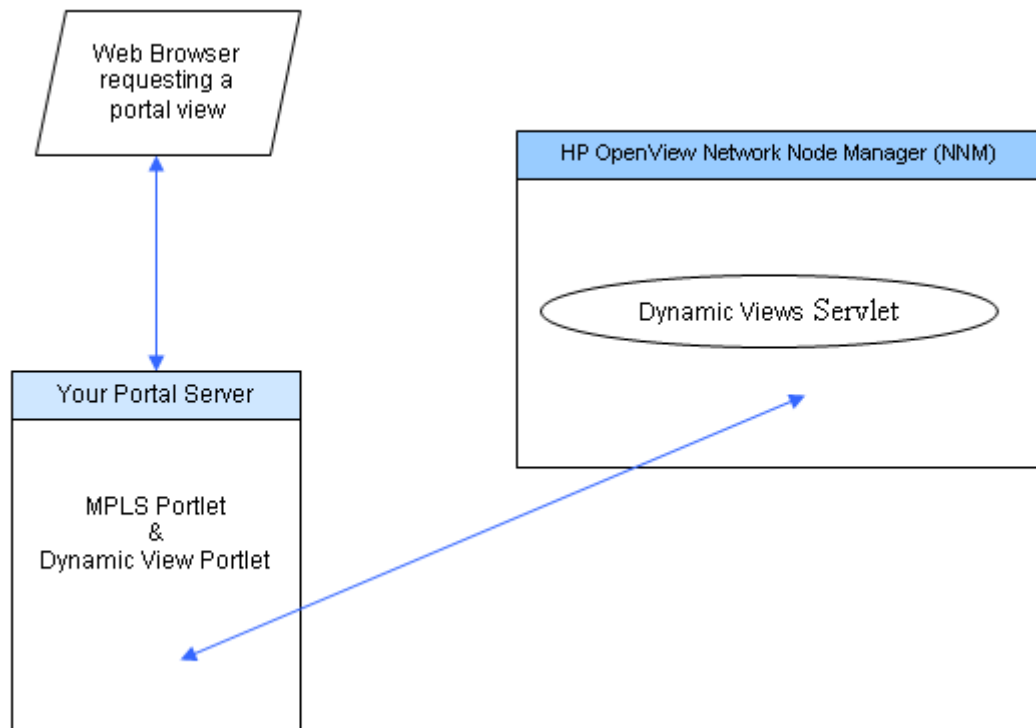
Figure 5 Communication Process for the MPLS and Dynamic View Portlet
