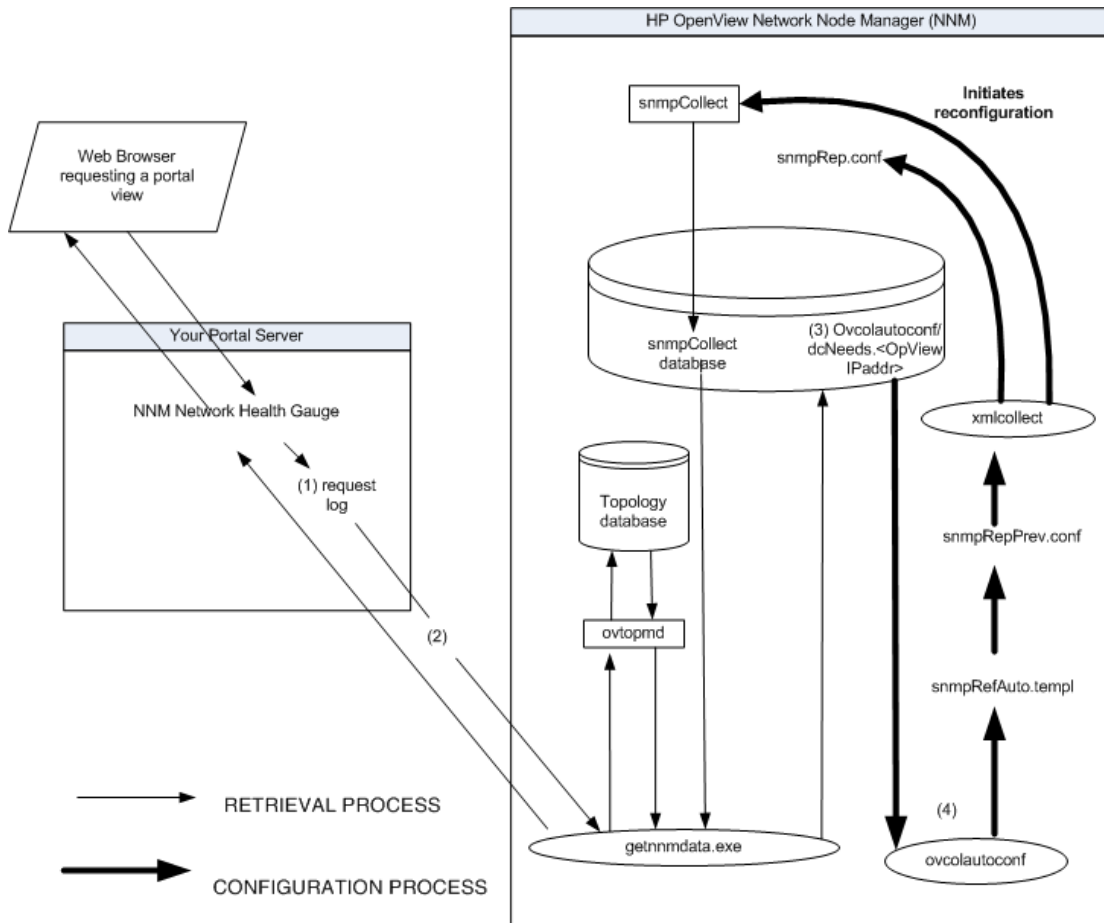
Figure 9 Communication Process for the Network Health Portlet
