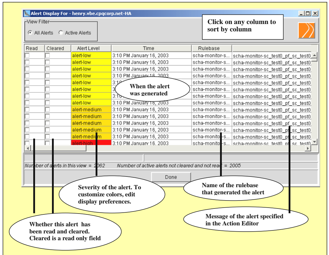
Figure 11: TIBCO Hawk Display: Result of Show Alerts on platform agent
