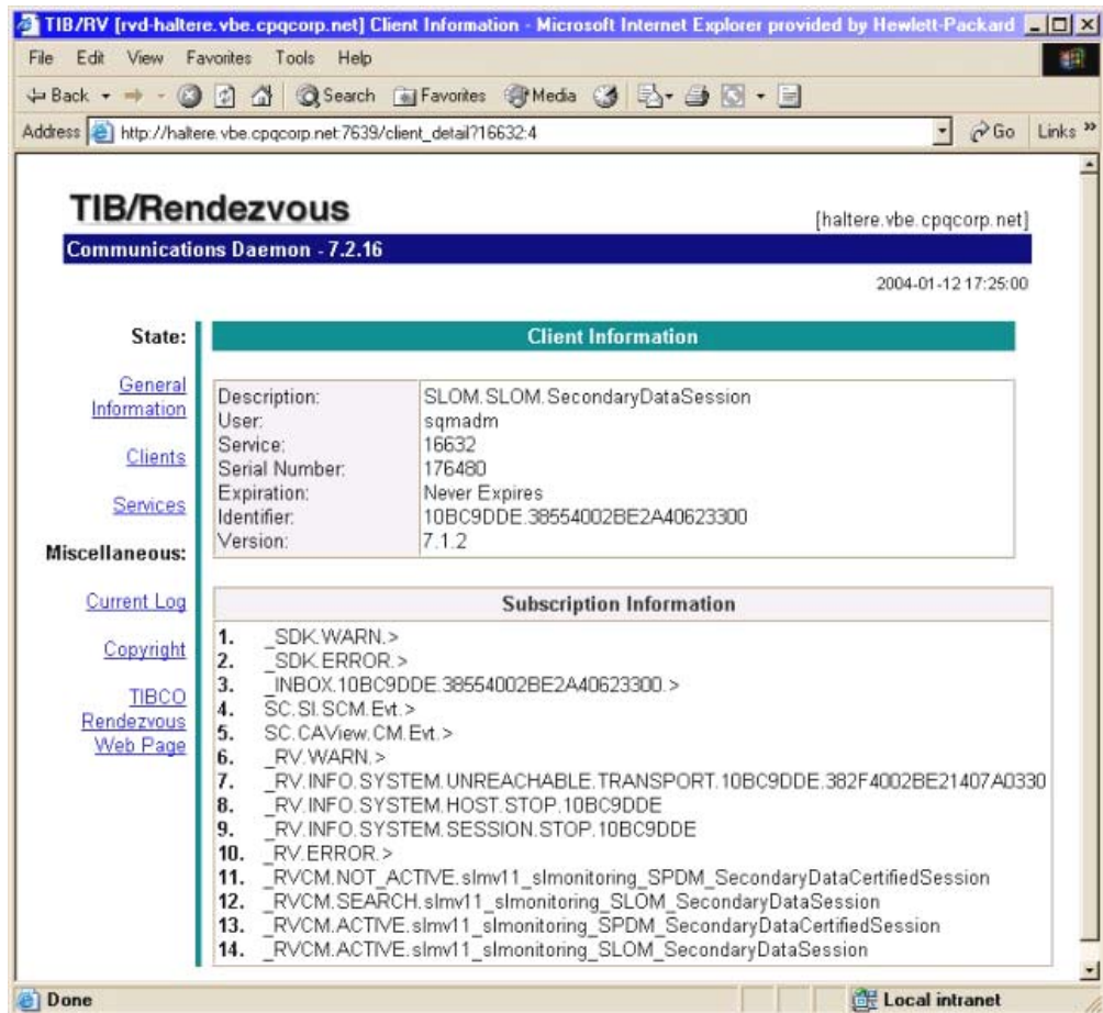
Figure 22: TIBCO Rendezvous Clients detailed information page
