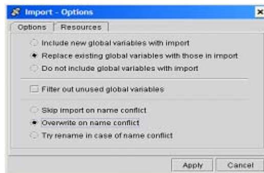
Figure 31: Import options
