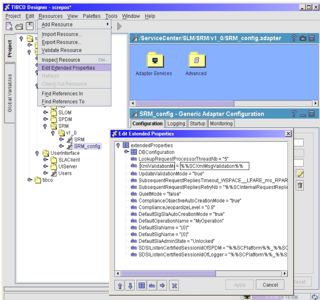
Figure 33: SRM_config display using the TIBCO Designer
