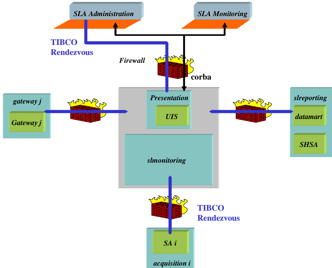
Figure 16: SQM and firewalls
