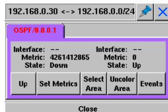
Figure 100 Link Information Panel
