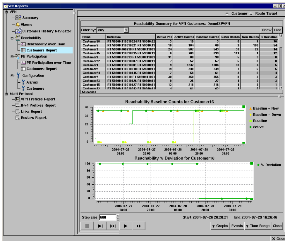
Figure 109 RT Reachability Summary with Graph
