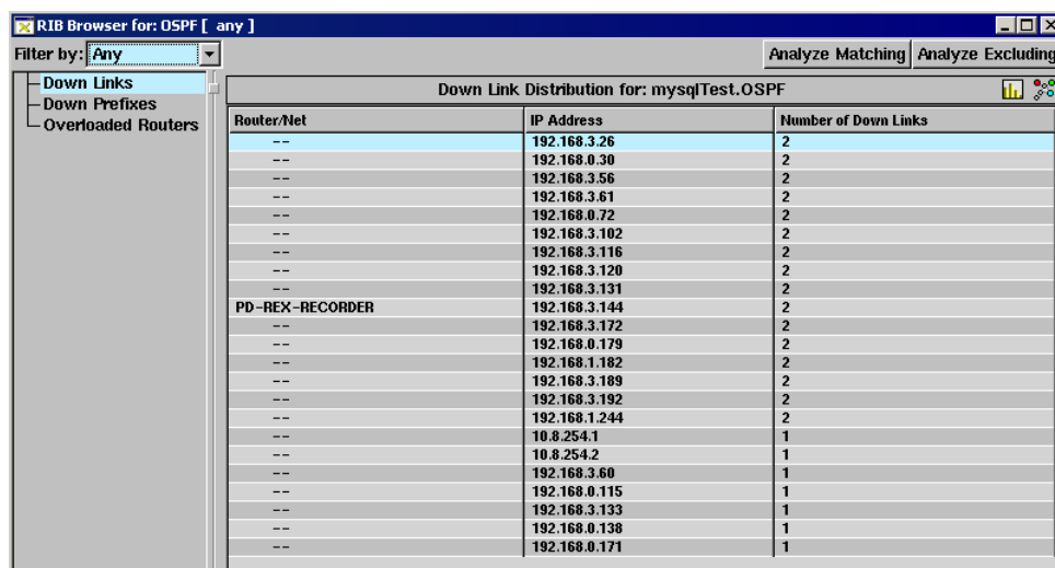
Figure 61 RIB Browser Dialog Box For IGP
