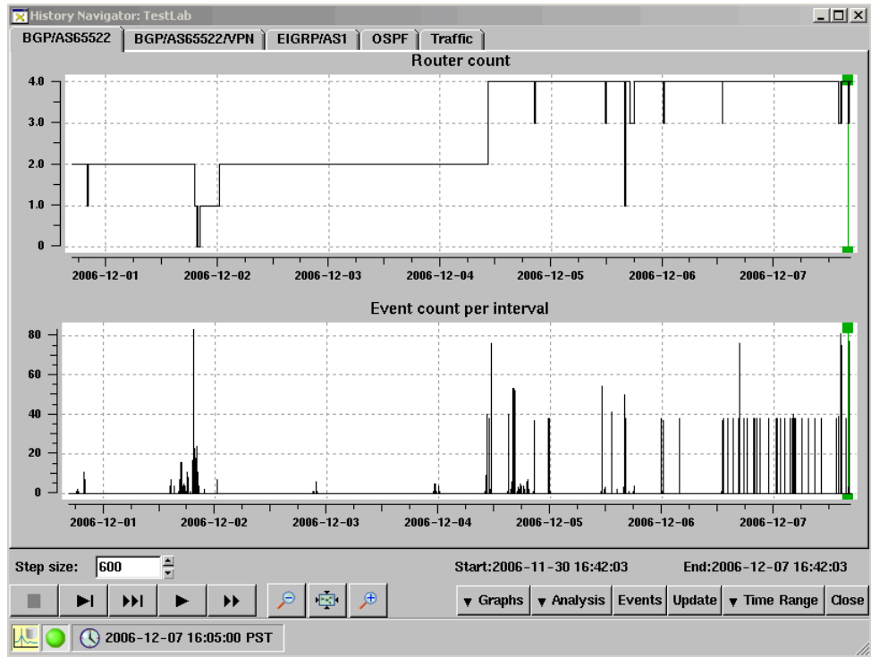
Figure 55 History Navigator Window in History Mode
