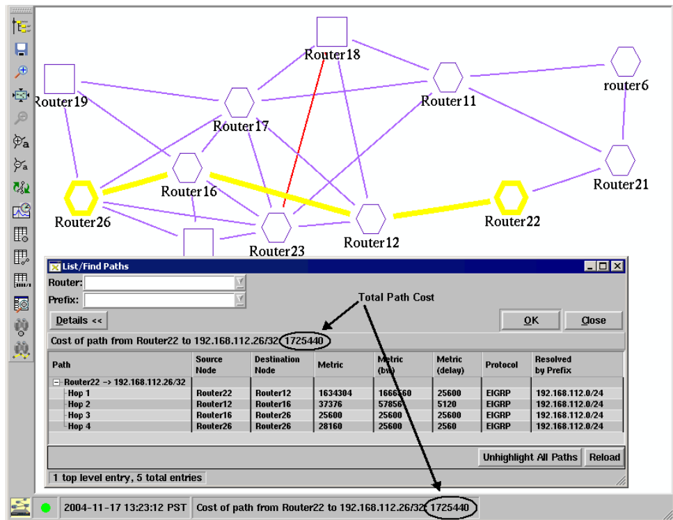
Figure 51 Highlighted Path Details for EIGRP
