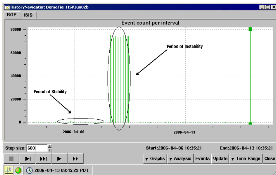
Figure 72 Stability and Instability
