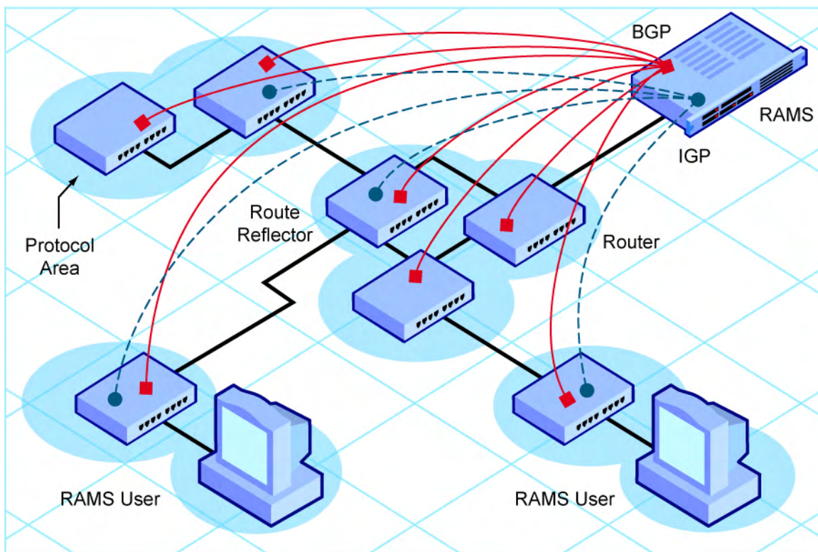
Figure 1 Connection to a Network
