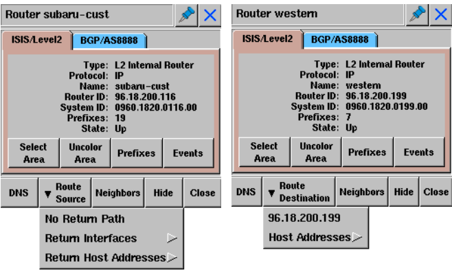
Figure 50 Source and Destination Node Information Panels
