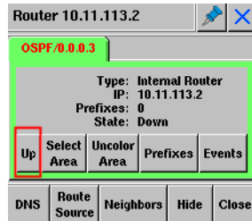
Figure 96 Node Information Panel
