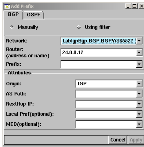
Figure 91 Add BGP Prefix Manually Dialog Box
