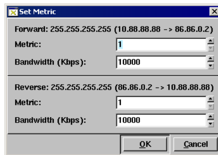
Figure 101 Set Metric Dialog Box - OSPF
