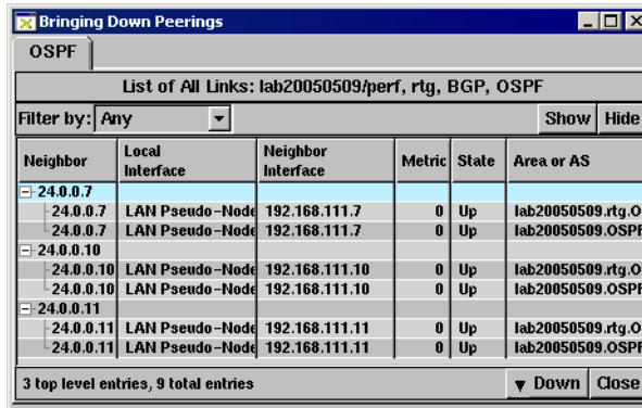
Figure 97 Bringing Down Peerings Dialog Box
