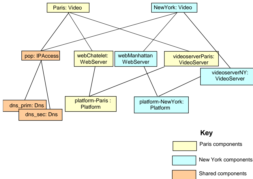
Figure 35 Instantiation of the Video Service
