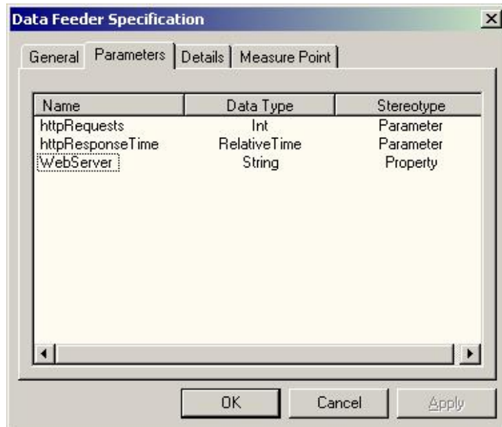
Figure 38 OpenView Service Designer UI: Data Feeder Attributes
