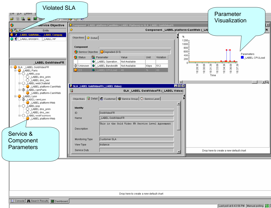
Figure 26 OpenView SQM SLA Monitoring UI
