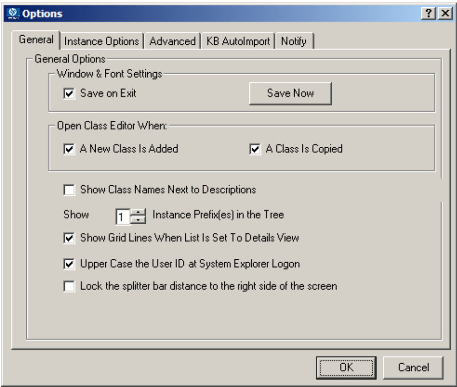
Figure 8 System Explorer Options General tab
