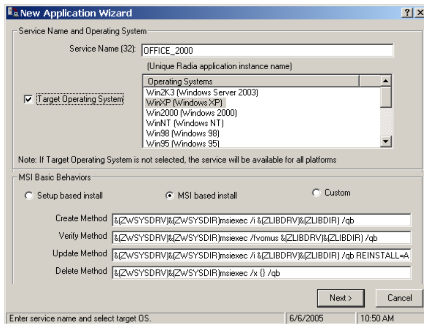
Figure 32 MSI Basic Behaviors in New Application Wizard
