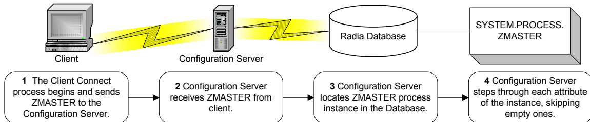
Figure 47 Configuration Server performing resolution
