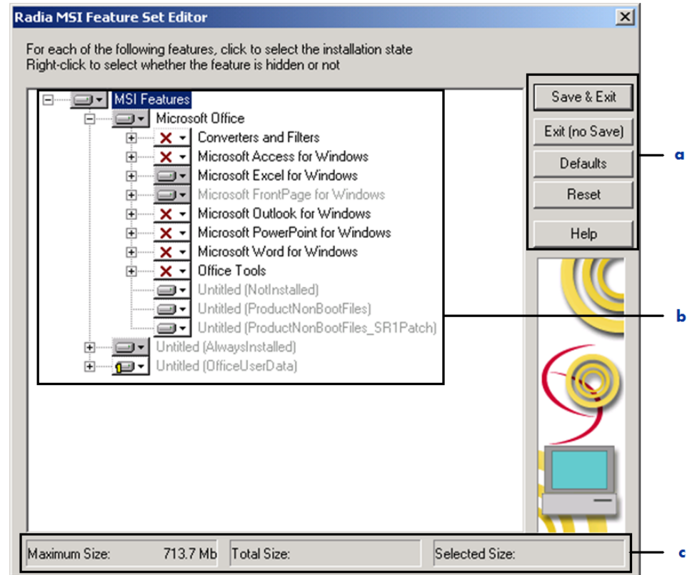
Figure 56 Feature Set Editor dialog box
