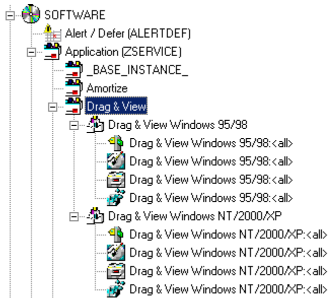
Figure 22 Example of Drag & View service and its connections.
