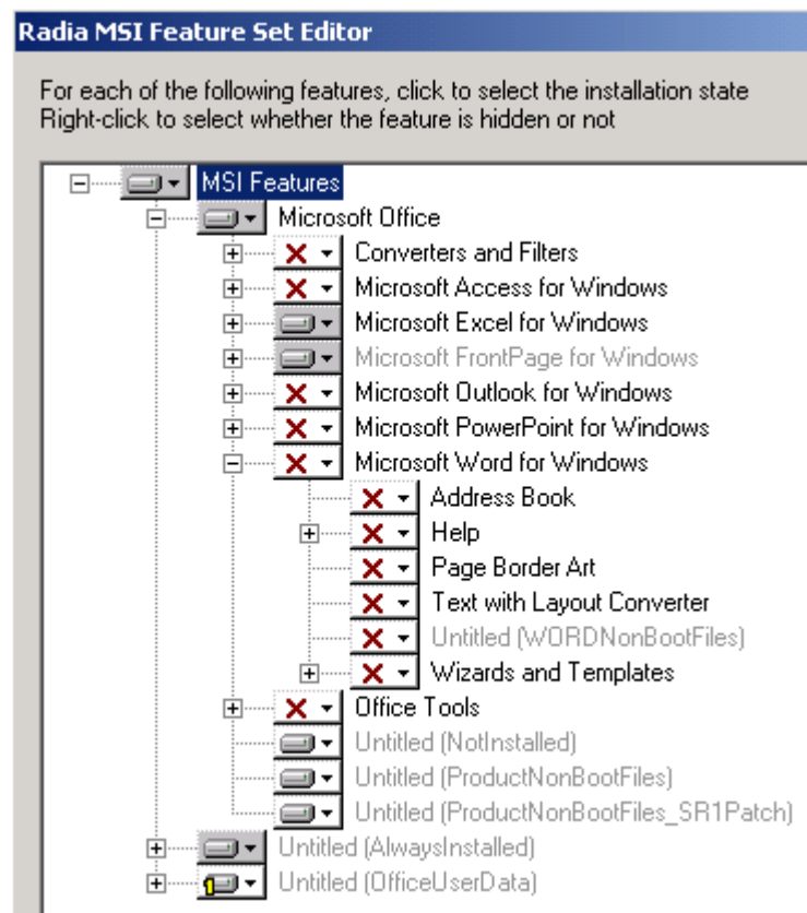
Figure 57 Child features displayed
