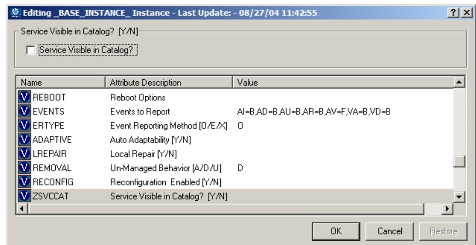
Figure 16 Attribute Description for ZSVCCAT variable terminates with [Y/N], indicating a flag attribute
