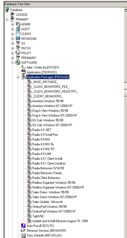
Figure 20 Application Packages (PACKAGE) class
