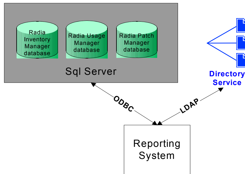
Figure 69 Radia Reporting Environment
