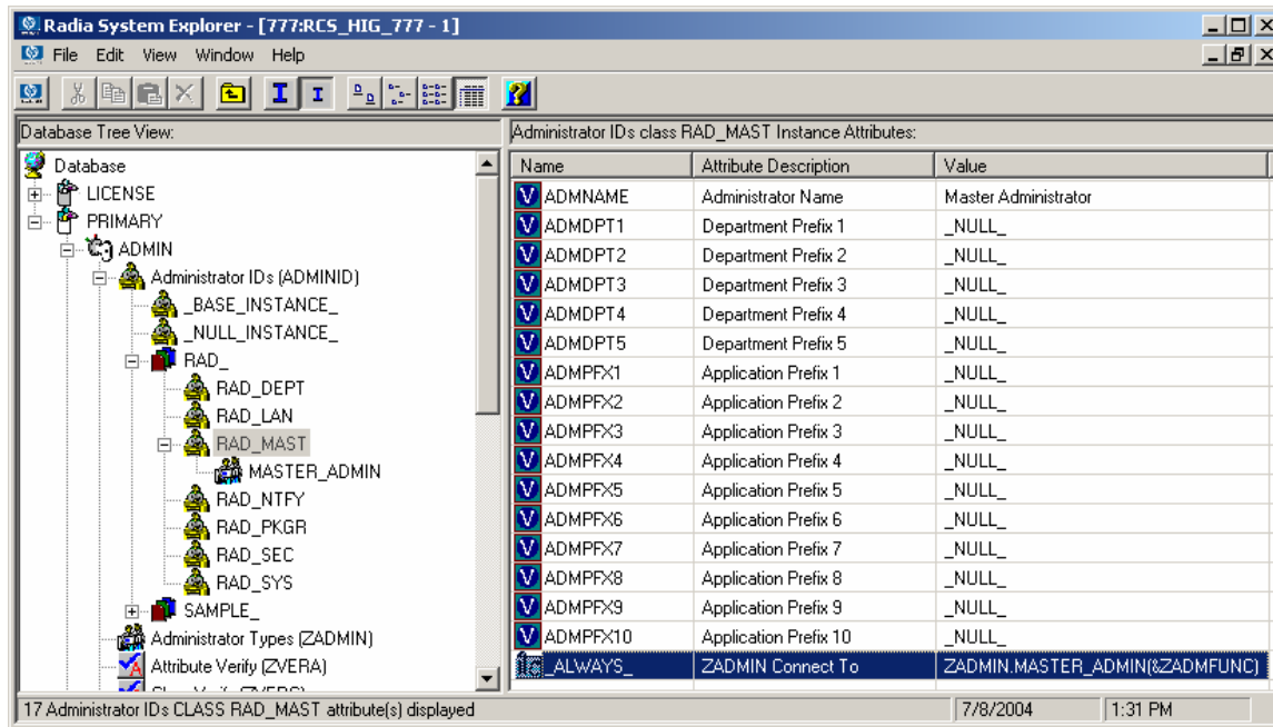
Figure 41 The RAD_MAST instance connections
