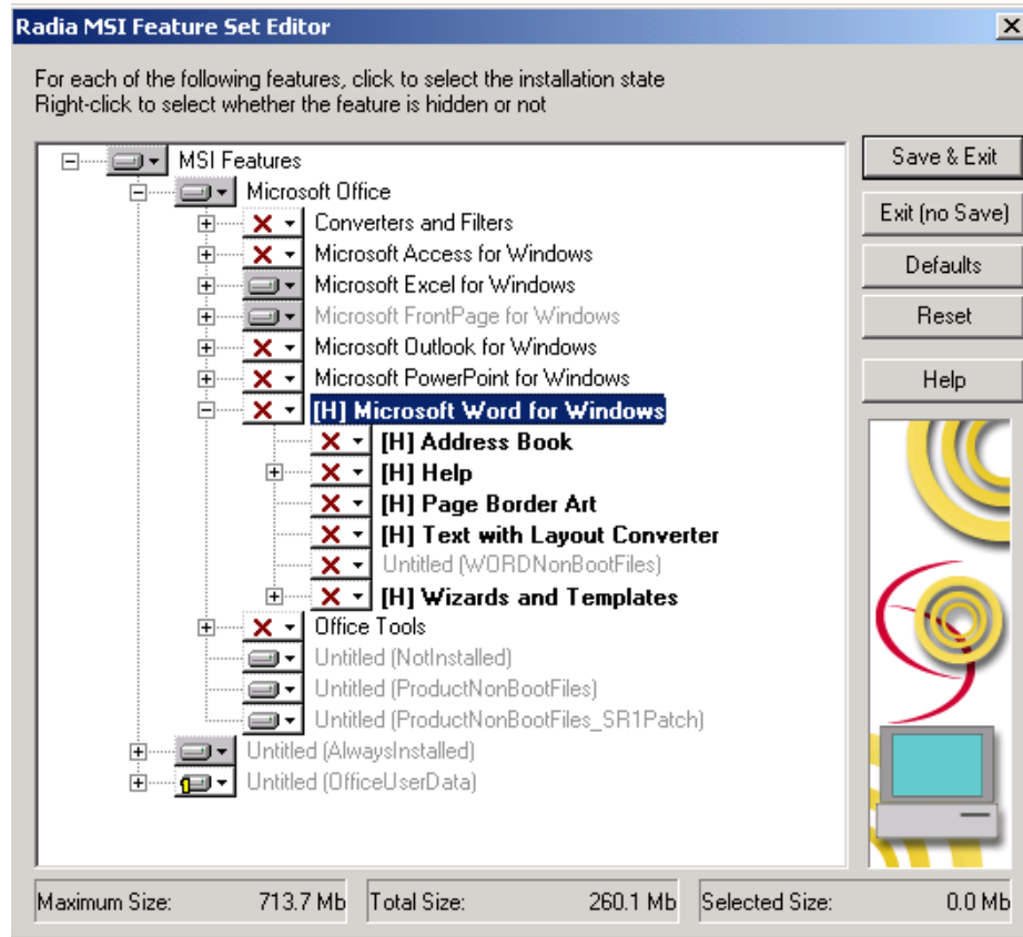
Figure 63 Hidden features have the prefix (H) before their names
