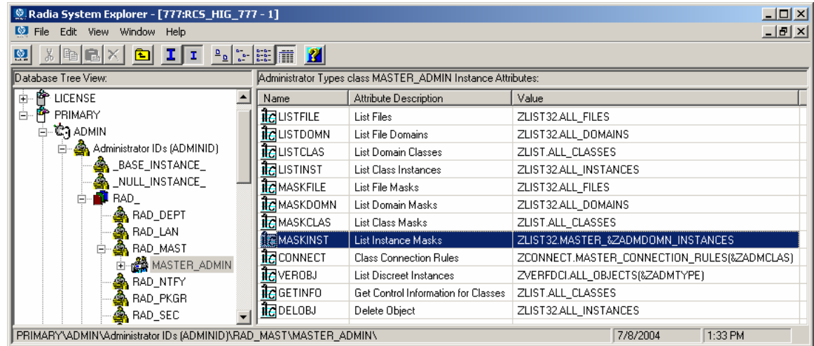
Figure 42 ZADMFUNC variable set to MASKINST
