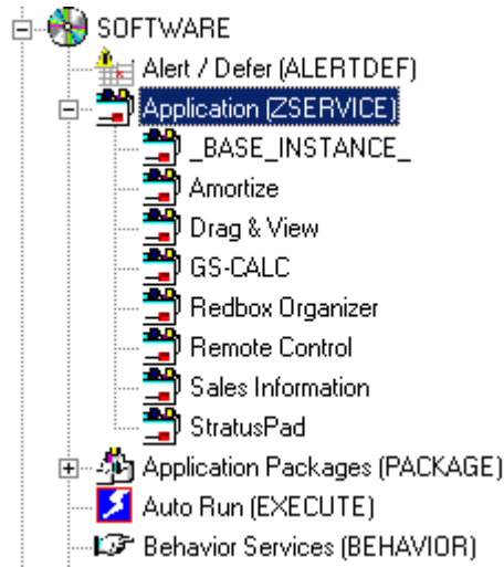
Figure 21 Sample Application (ZSERVICE) instances
