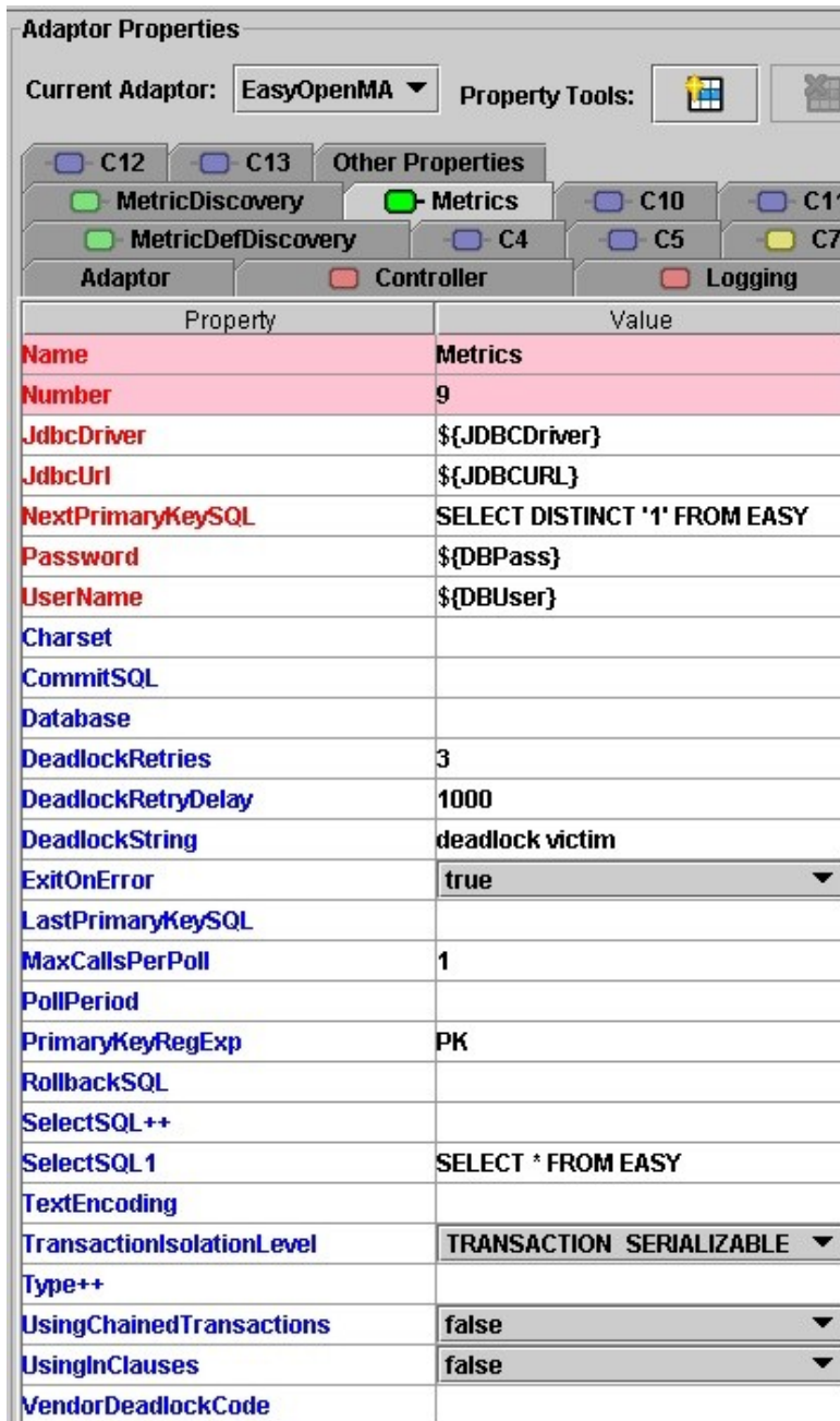
Figure 19: Configuration of the Metric Data Values Collection Source
