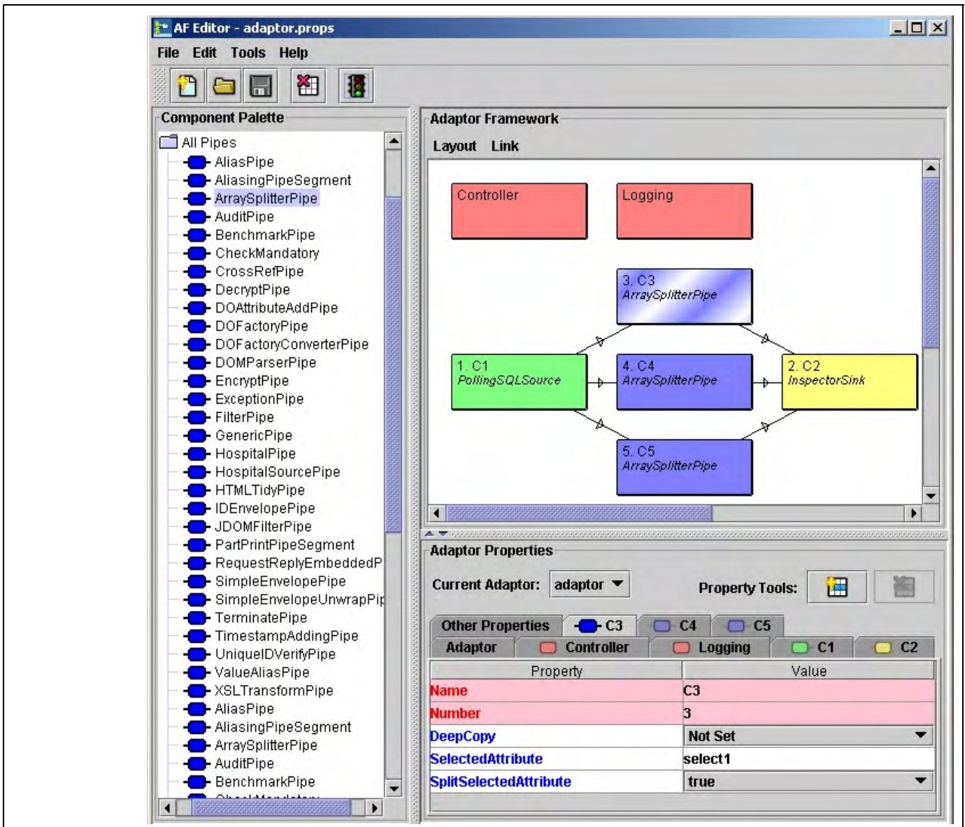
Figure 34: Revise the Example Adaptor with ArraySplitterPipe
