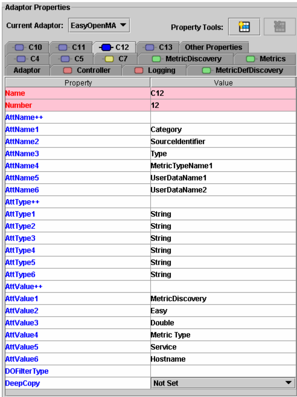
Figure 21: Configuration of One DOAttributeAddPipe
