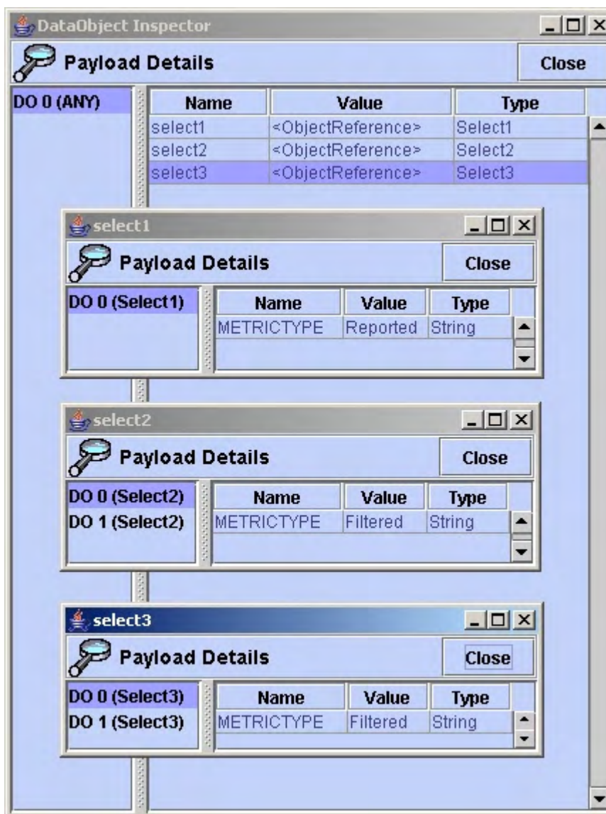
Figure 32: Values of Attributes “select1”, “select2” and “select3”
