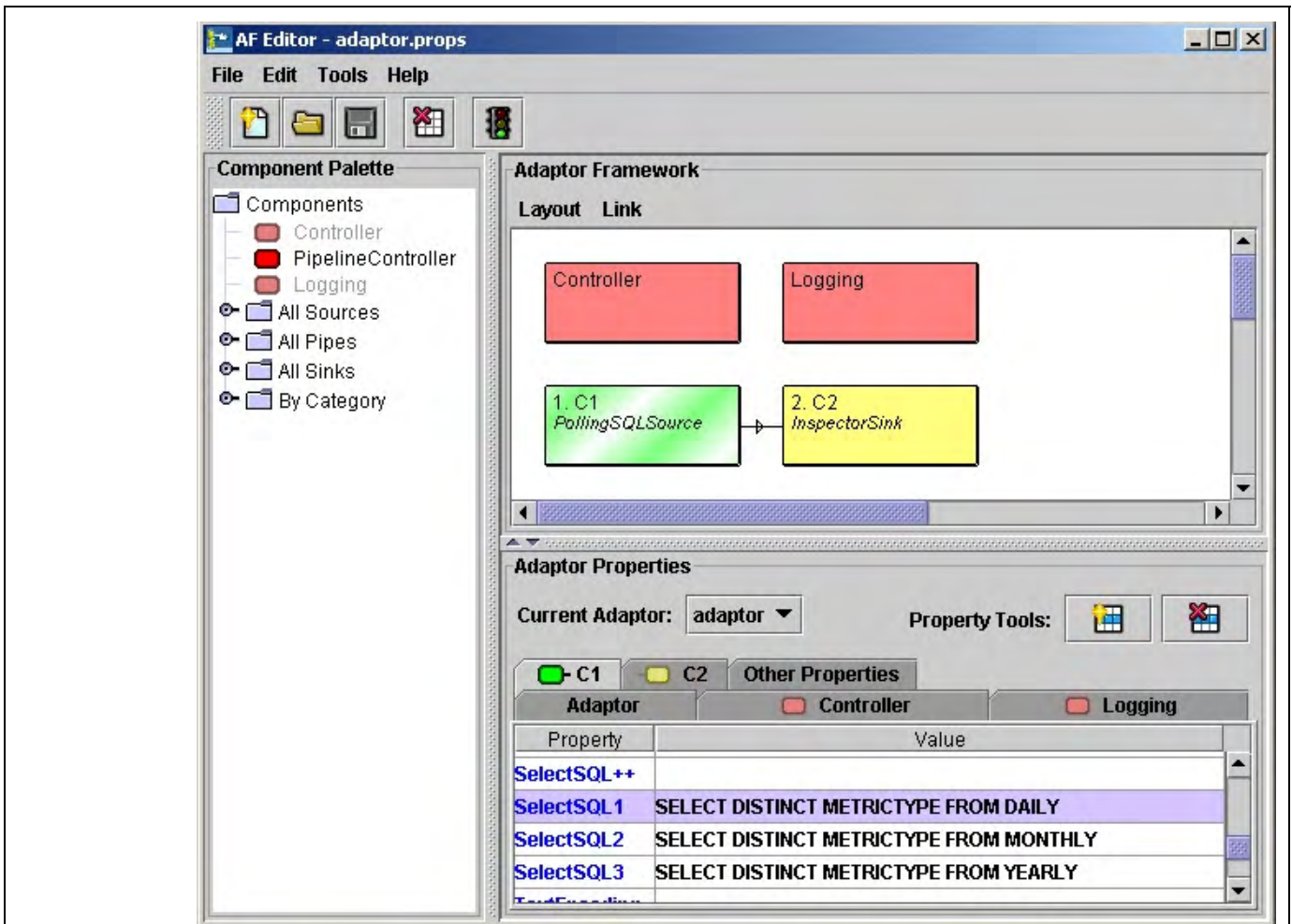
Figure 30: Adaptor Containing a PollingSQLSource With Three Select Statements
