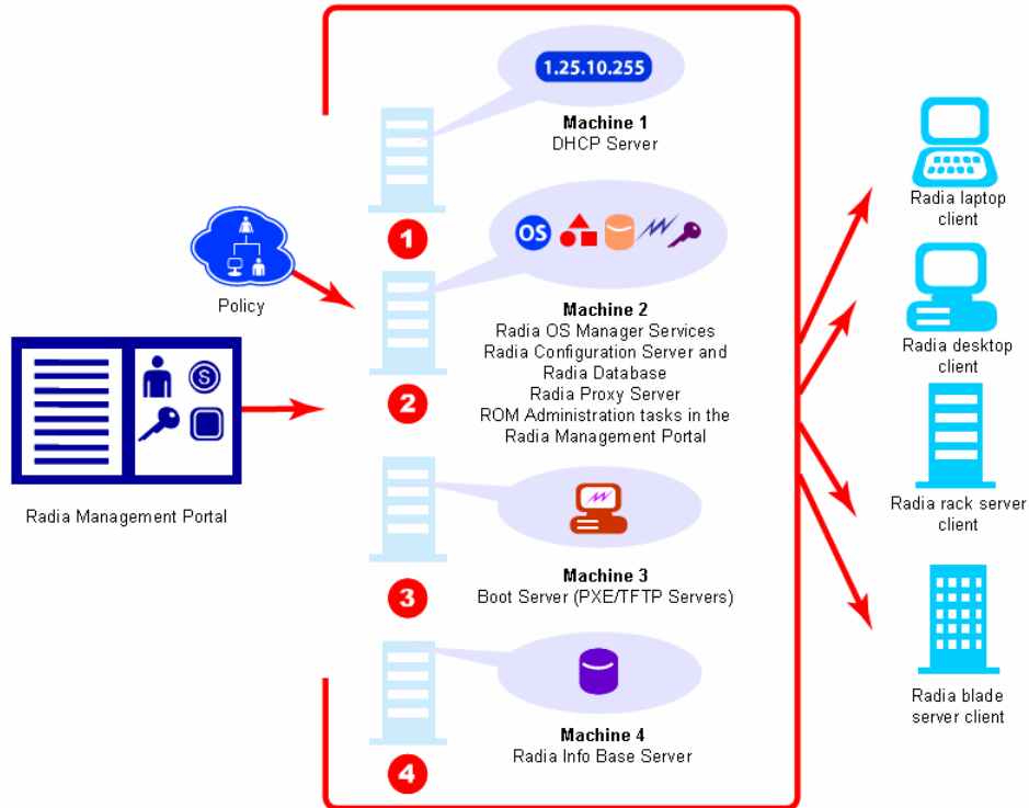
Figure 3.21 ~ Deployment architecture.
