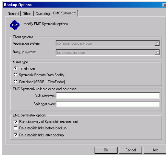
Figure 19 Backup options
