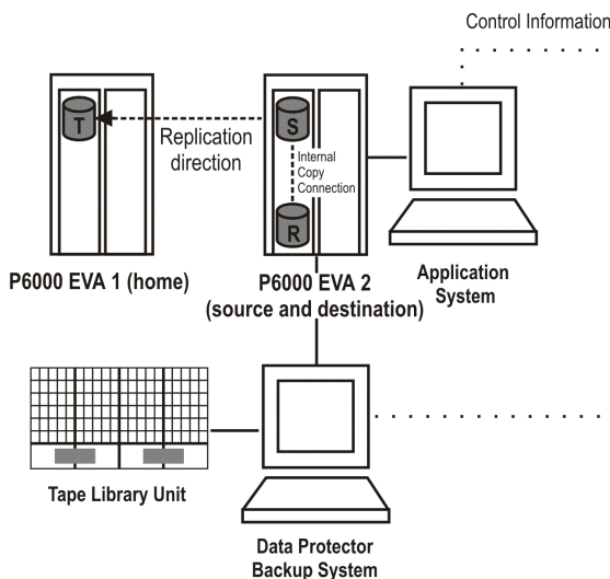
Figure 6 Failover scenario 2
