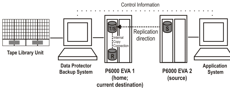
Figure 5 Failover scenario 1
