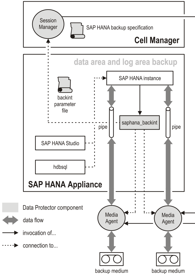
Figure 54 SAP HANA integration architecture
