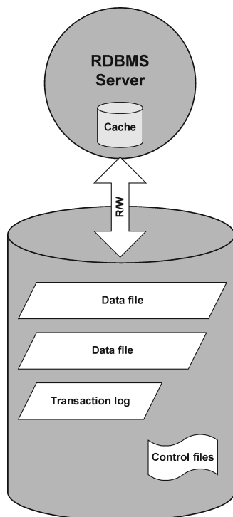
Figure 73 Relational database
