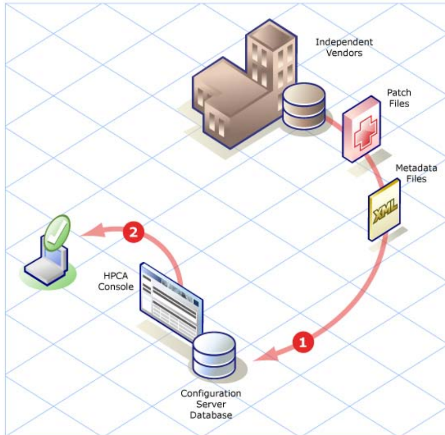
Figure 49 Patch Management Model - traditional
