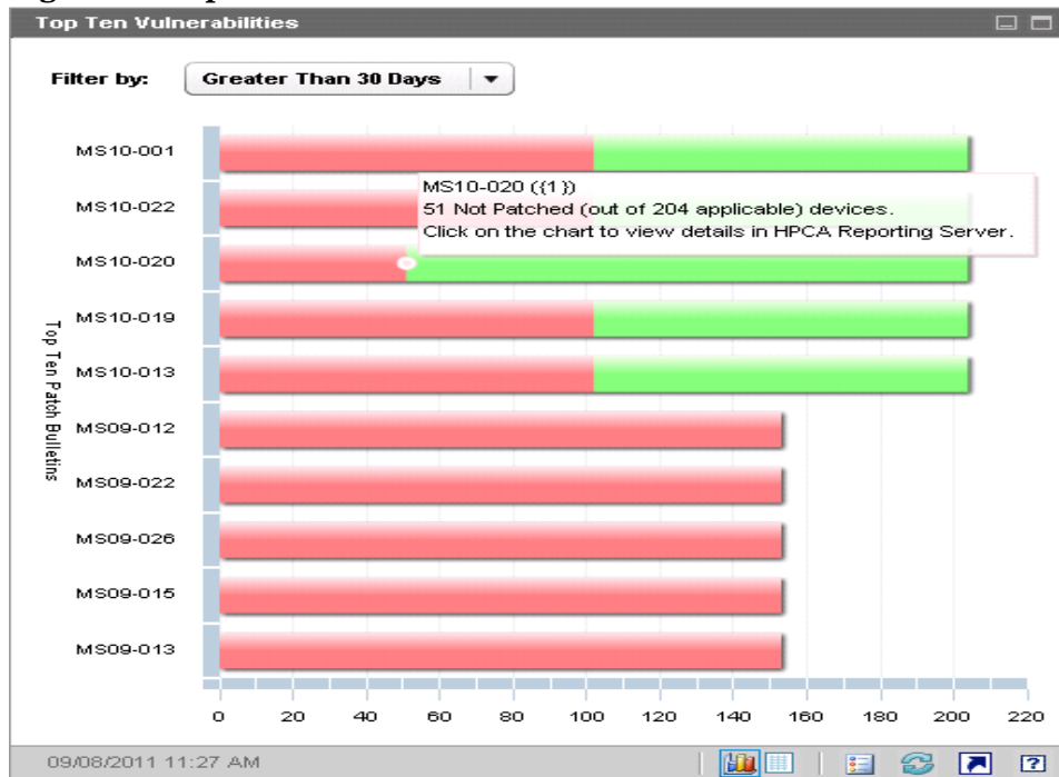
Figure 35 Top Ten Vulnerabilities
