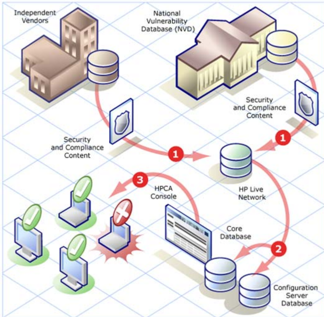
Figure 1 Security and Compliance Management in HPCA
