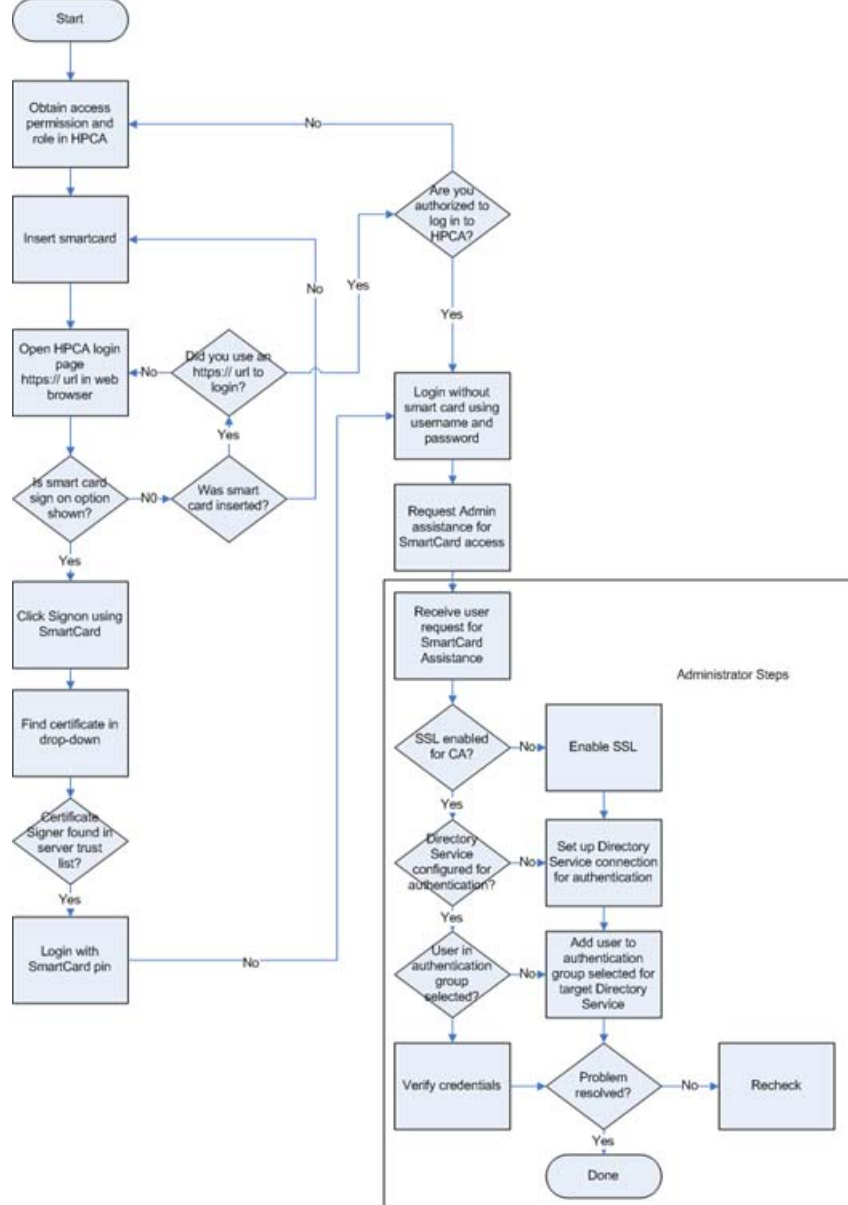
Figure 58 Smart card Login Process
