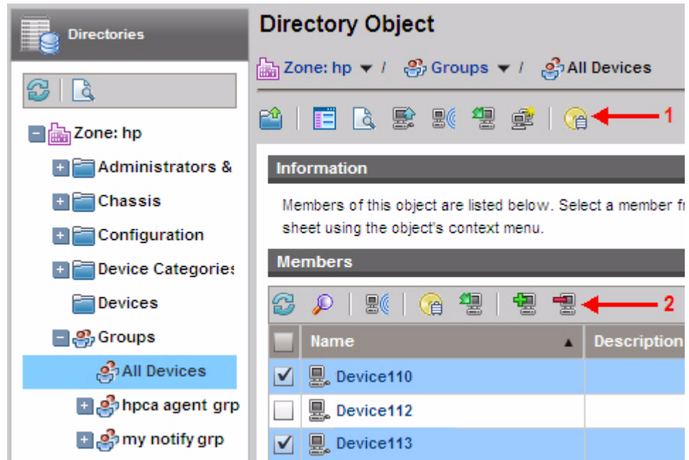
Figure 41 Directory Object View Toolbars
