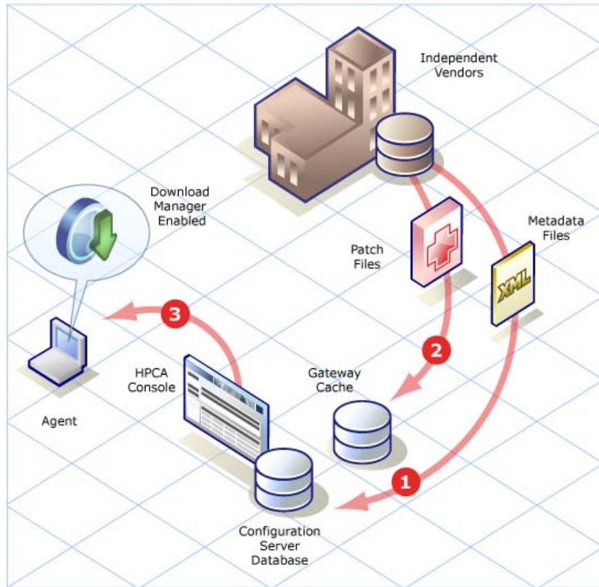
Figure 48 Patch Management using Metadata Model
