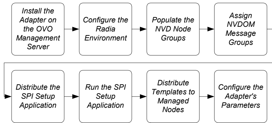
Figure 2: Eight installation steps of Adapter for HP OpenView Operations.
