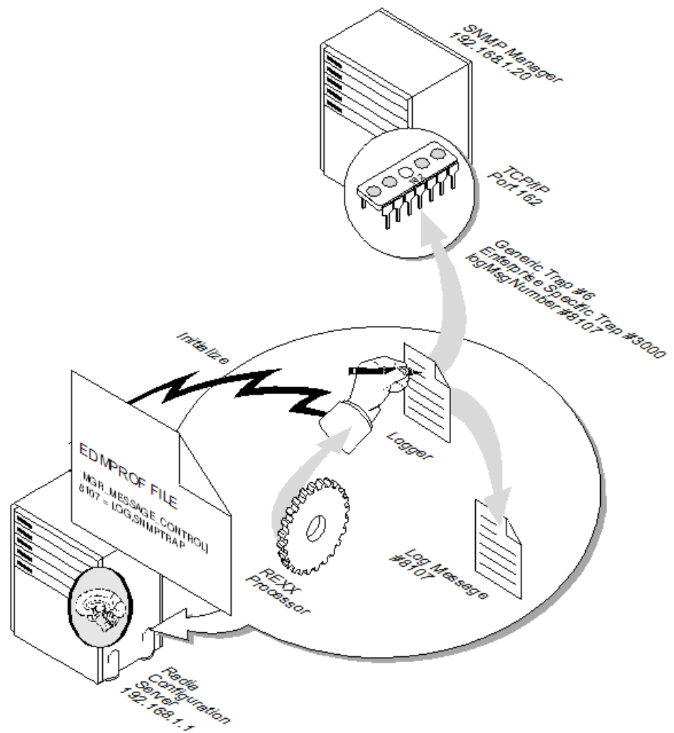
Figure 3: LOG and SNMPTRAP as destinations for message 8107.
