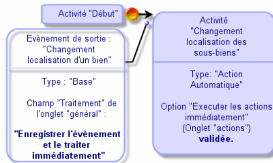
Figure 8.6. Exemple de workflow synchrone
