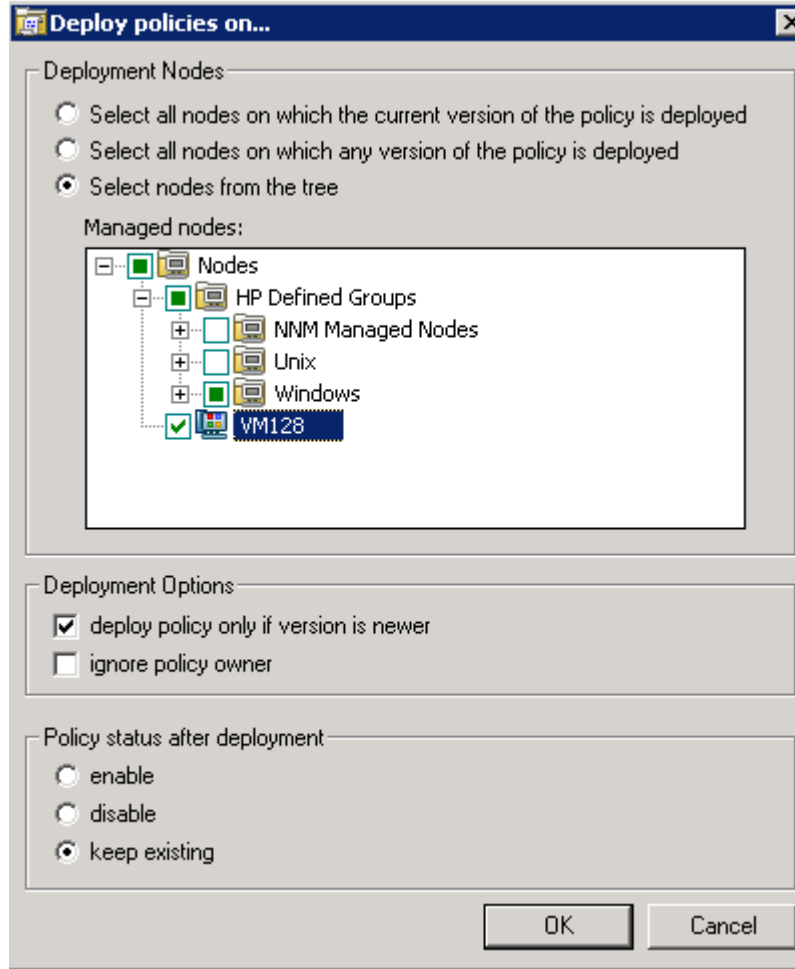
Figure 3 Deploy policies on dialog box
