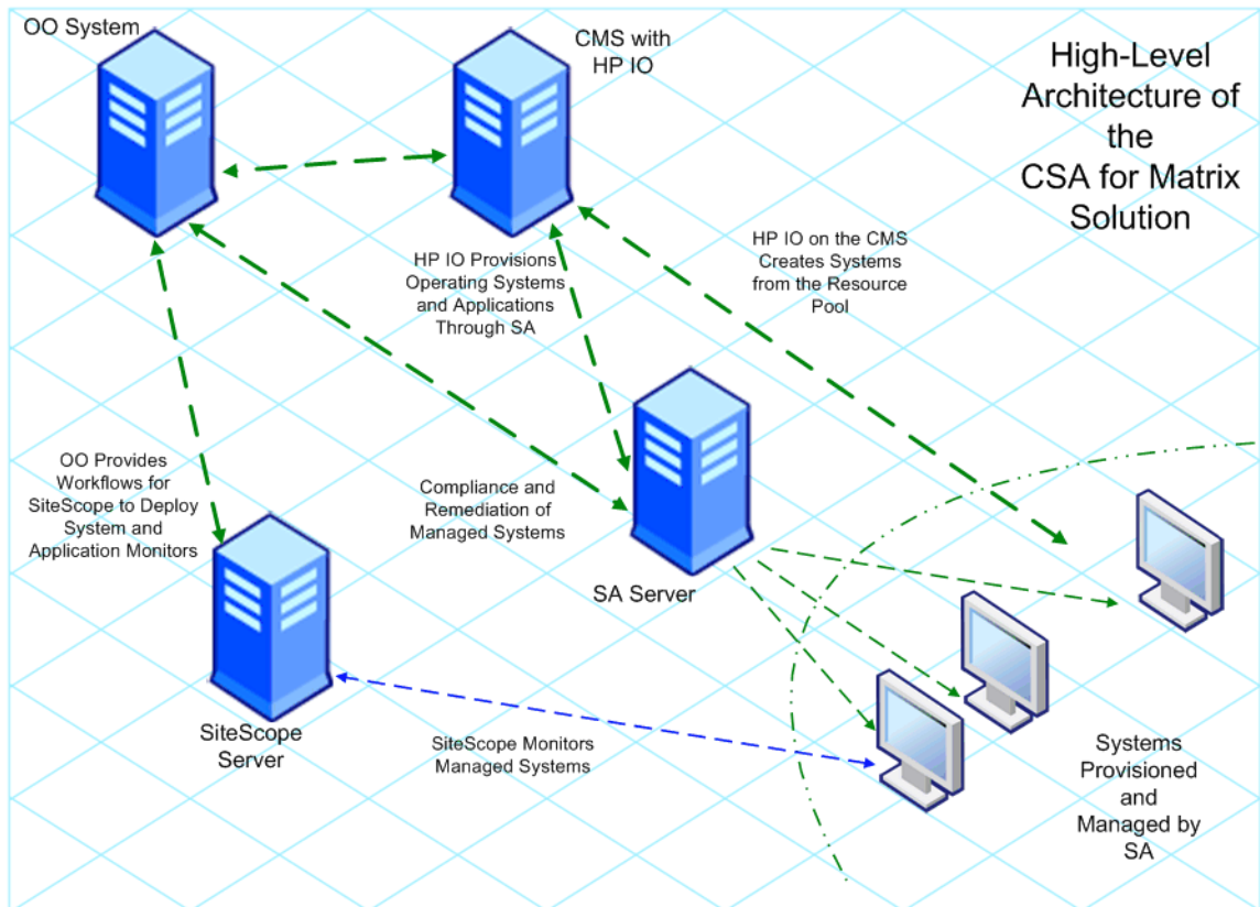
Figure 2 High-Level Architecture
