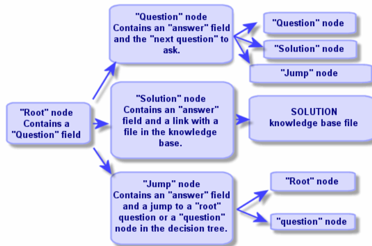
Figure 1 1.1. Decision trees - logical links between node types
