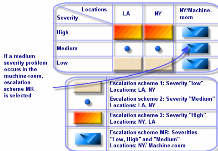
Figure 9.2. Escalation schemes - the role of locations and severities
