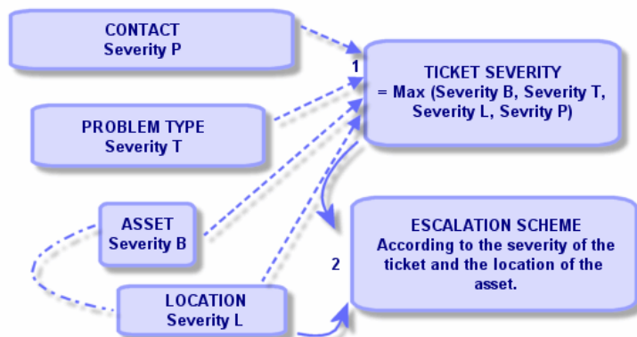
Figure 9.1. Escalation schemes - automatic assignment of a ticket
