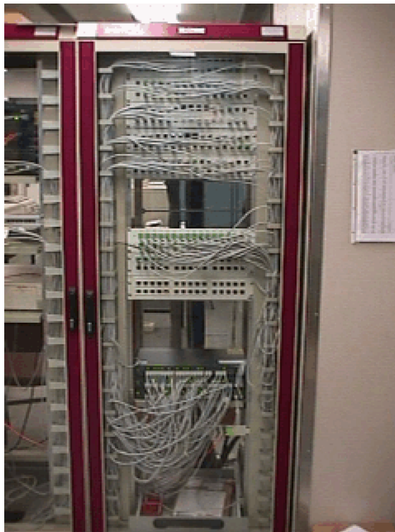
Figure 8.7. Rack - photo
