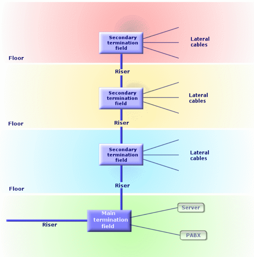
Figure 8.10. Lateral distribution of a cable network - representation
