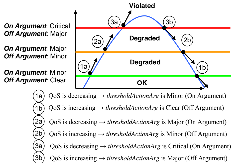
Figure 4 Threshold Crossing SNMP Traps Severity
