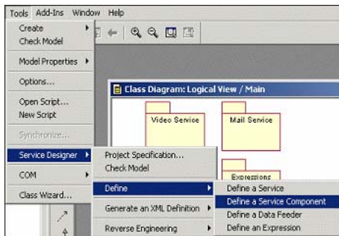
Figure 66 Definition Menus
