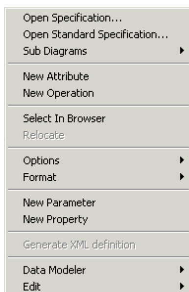
Figure 17 Definition Options
