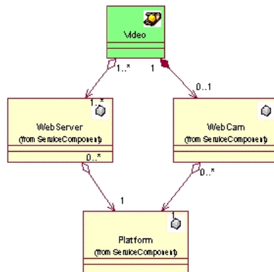
Figure 36 Part of a Model showing Unidirectional Aggregation
