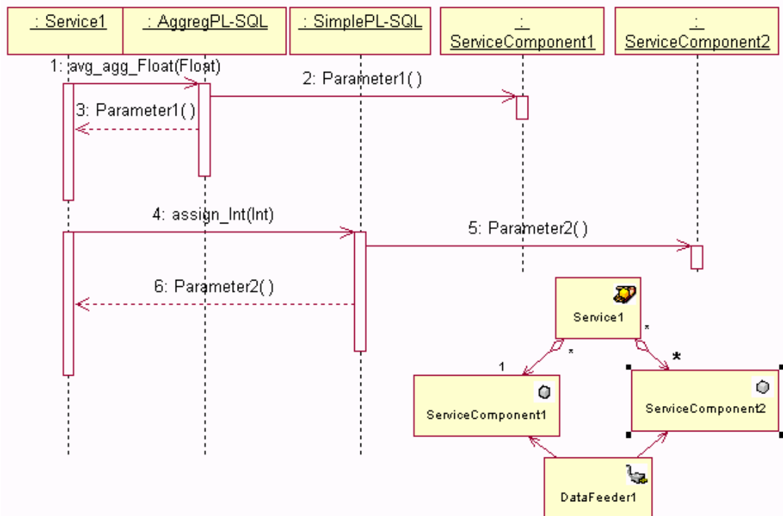
Figure 55 Case 4, Example of an Incorrect Sequence Diagram
