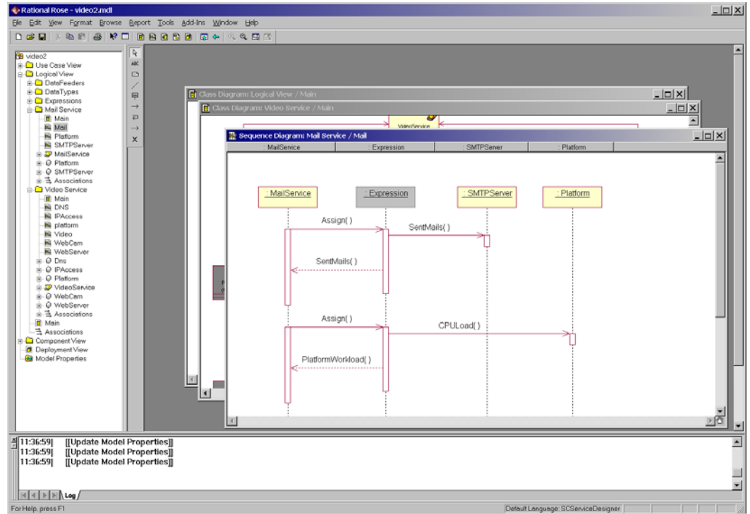
Figure 45 Sequence Diagram for a Mail Service (Component of Video2)
