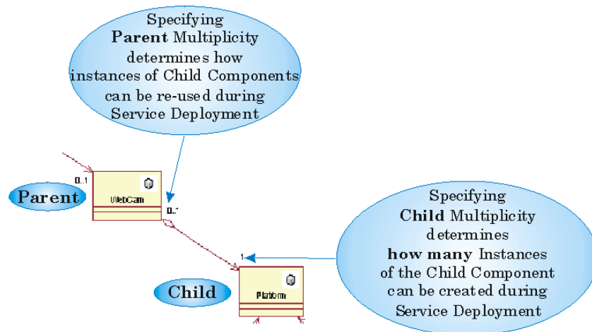
Figure 37 Parent and Child Multiplicity
