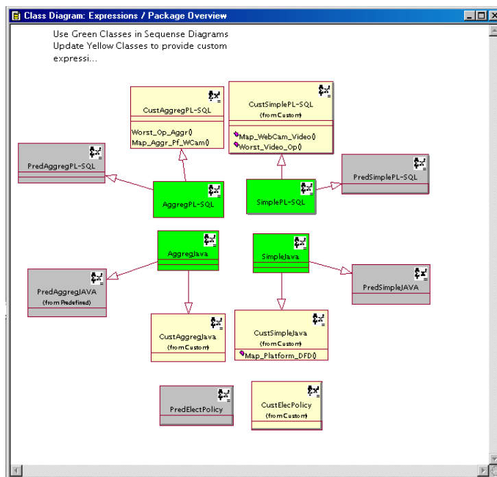
Figure 43 Expression Classes
