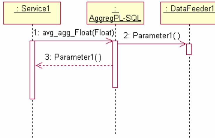
Figure 53 Case 2, Example of an Incorrect Sequence Diagram
