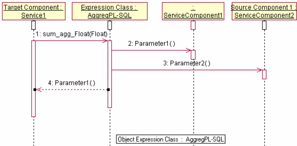
Figure 52 Case 1, Example of an Incorrect Sequence Diagram
