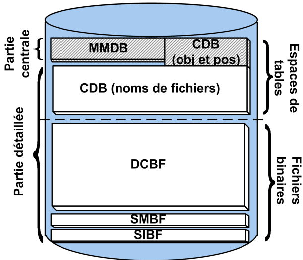
Figure 58 Parties de l'IDB
