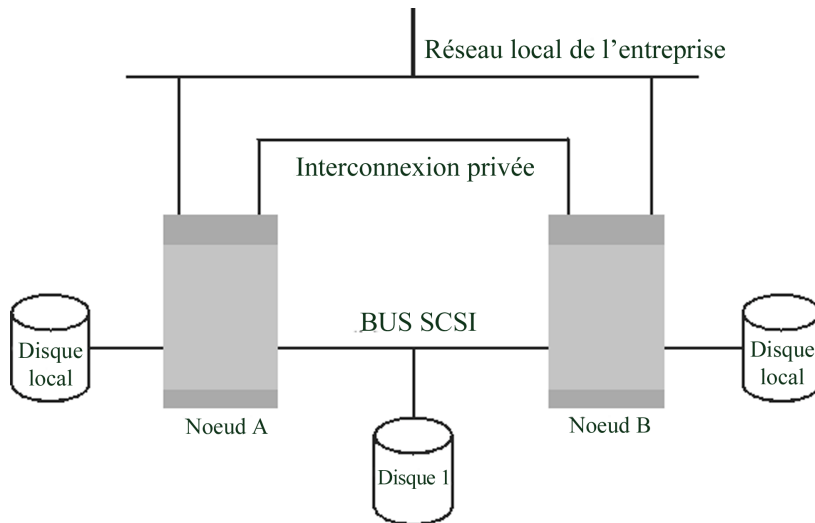
Figure 21 Structure d'un cluster type
