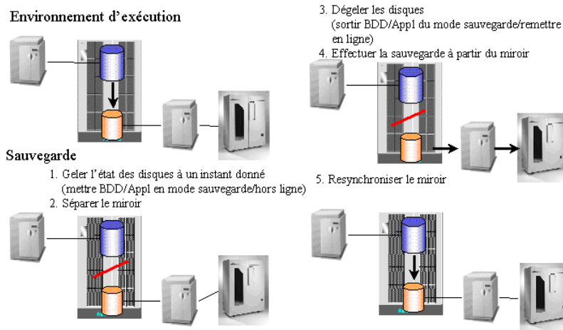
Figure 73 Concept de la sauvegarde Split Mirror
