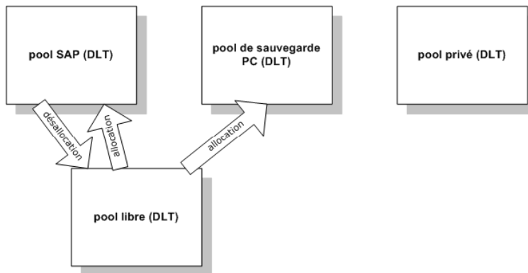
Figure 38 Pools libres
