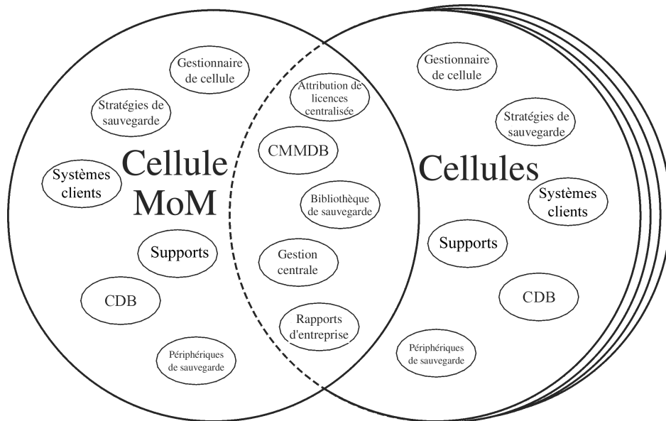
Figure 11 Environnement Manager-of-Managers
