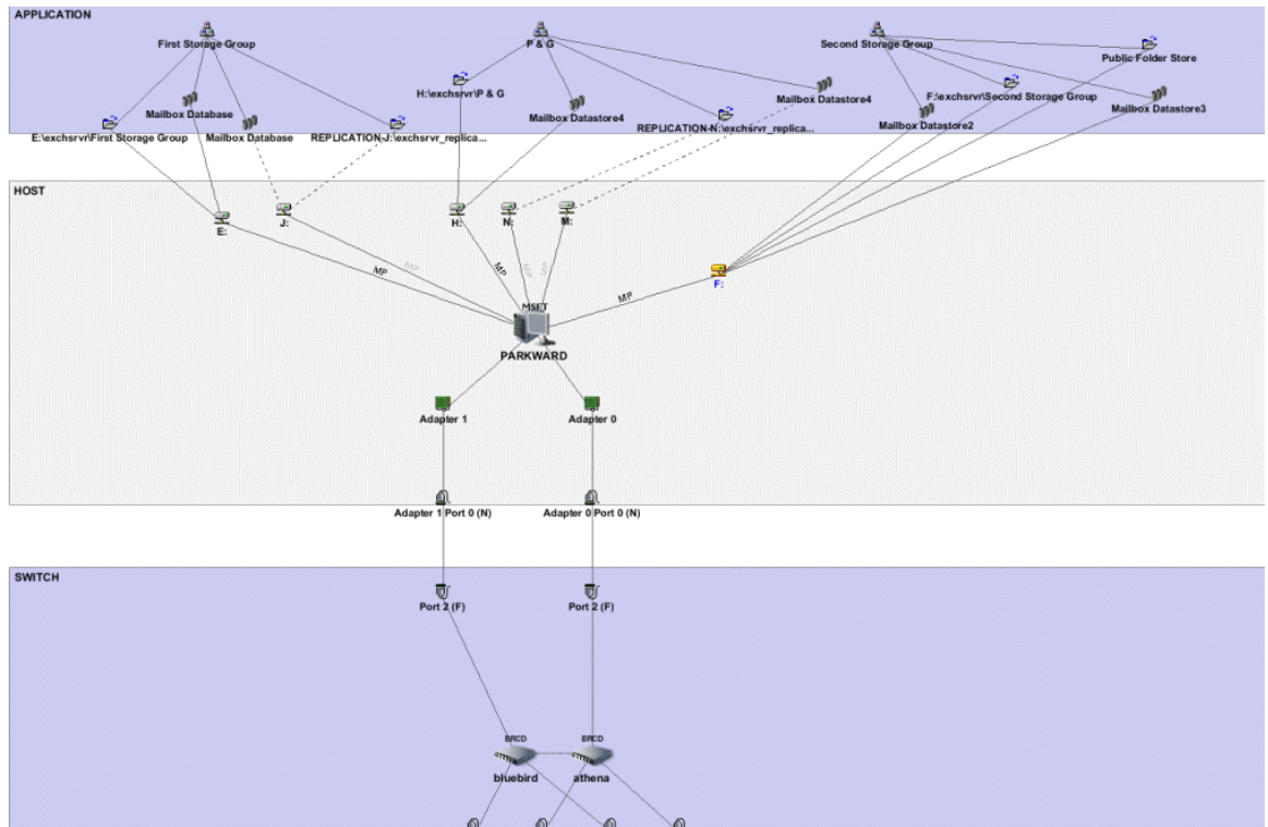
Figure 6 Topology of Microsoft Exchange LCR Cluster
