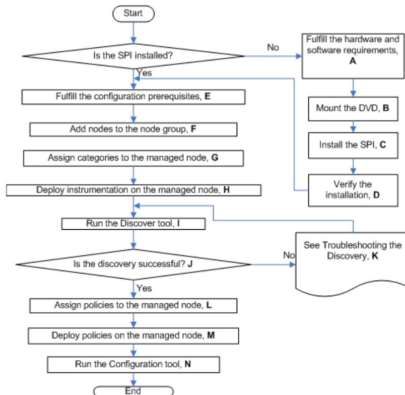
Figure 5 Flowchart for installing and configuring the SPI on HP-UX
