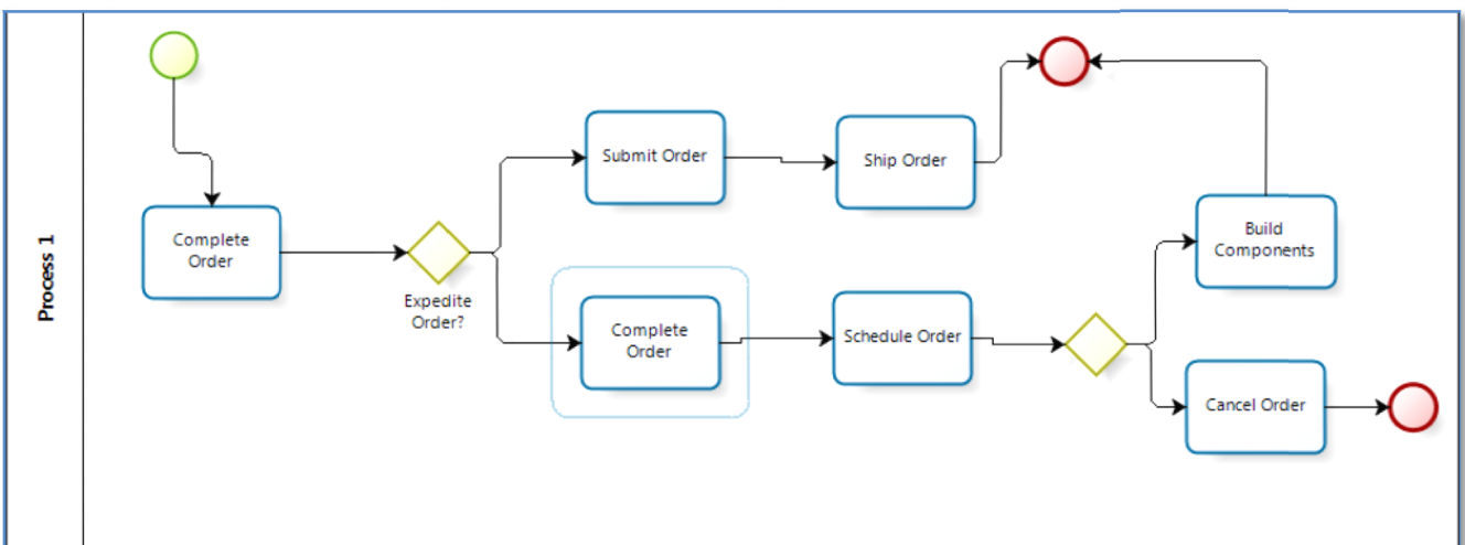
Figure 7: Sample business process diagram
