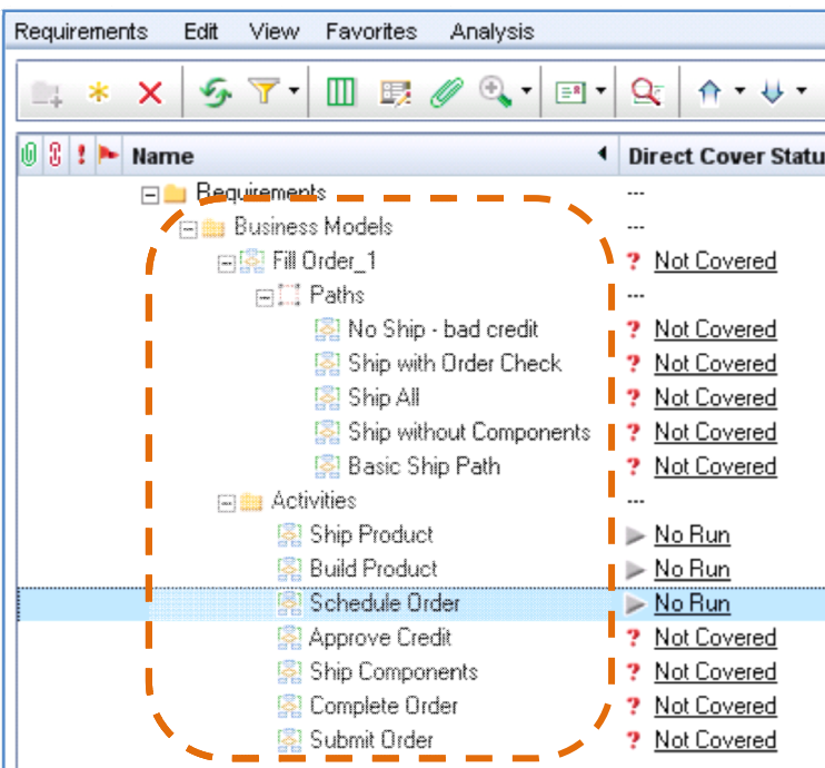
Figure 3: Screenshot of ALM Requirements module. The requirements tree includes the Business Models system folder, which contains all the newly created representative requirements.
