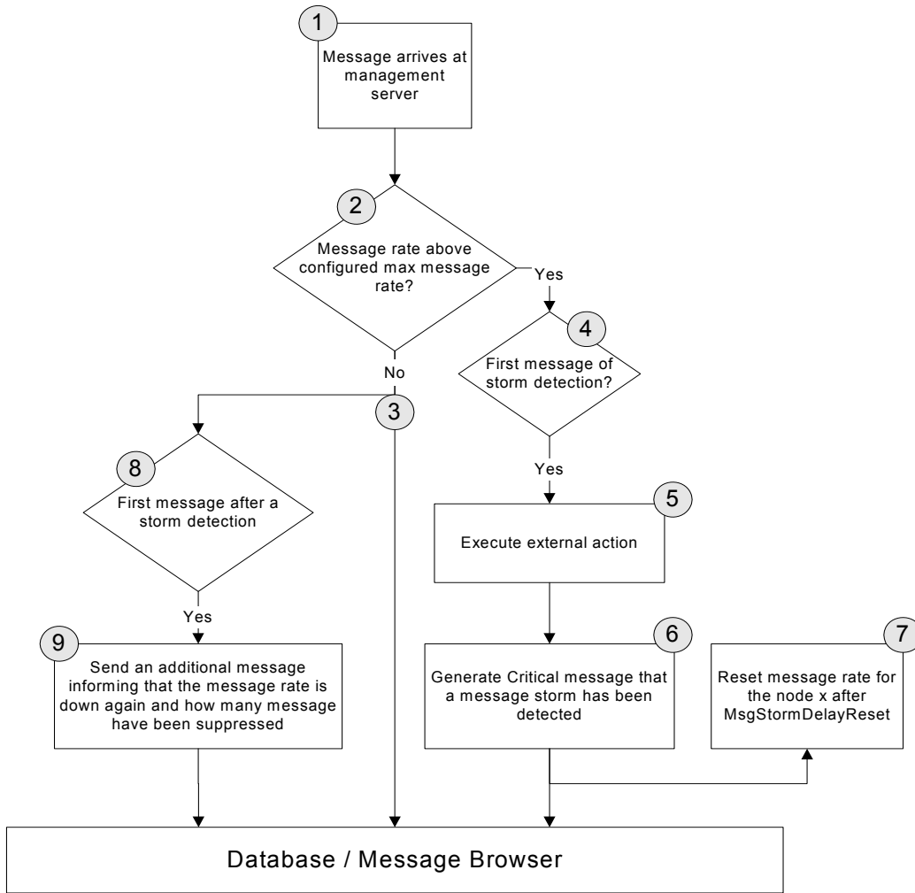
Figure A. Message flow when suppression is enabled
