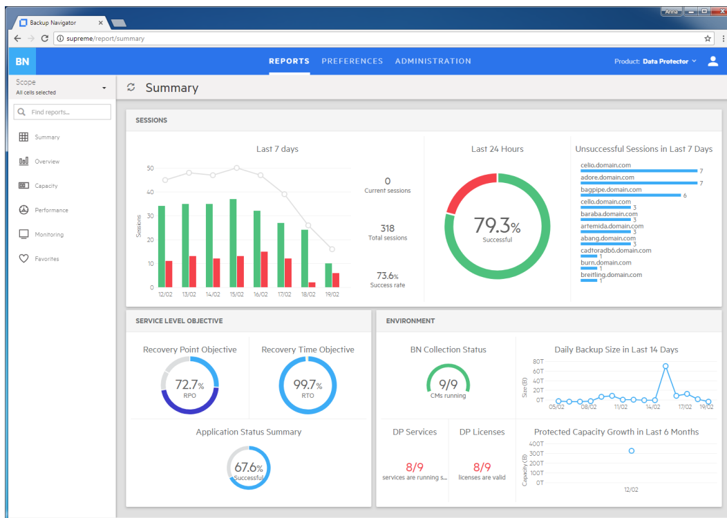
Figure 34: Summary dashboard
