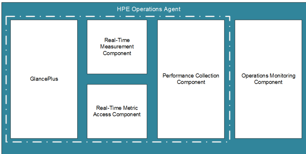
Figure 5: Components Enabled by the Glance Pak Software LTU
