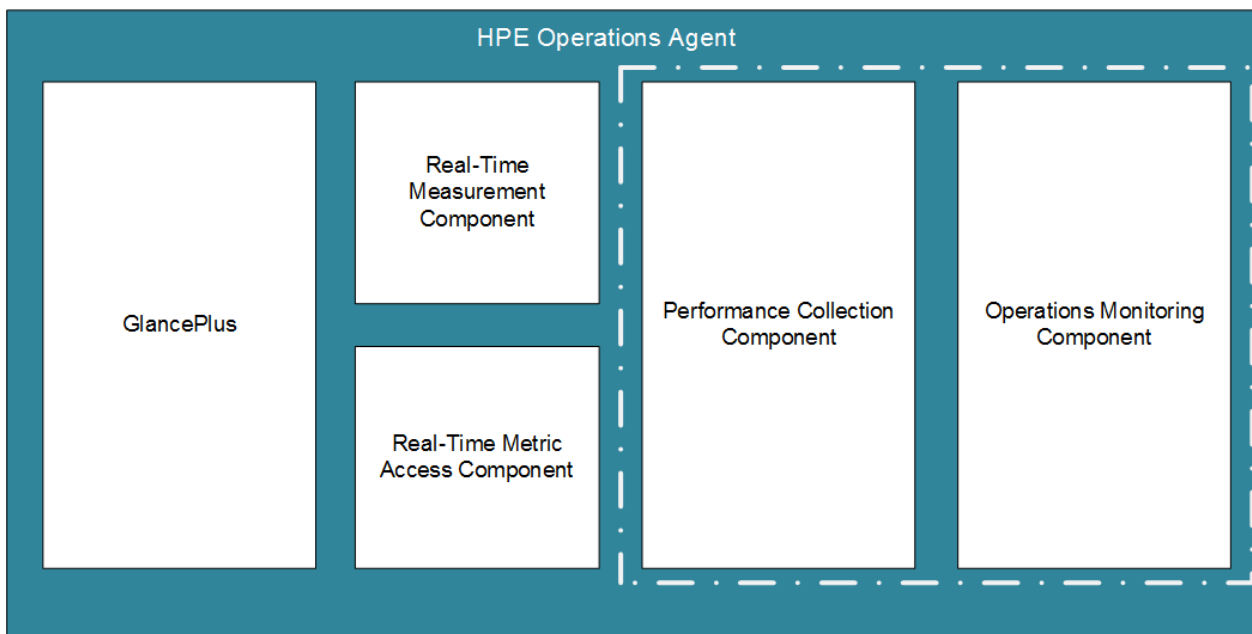
Figure 1: Components Enabled with the HP Operations OS Inst Adv SW LTU
