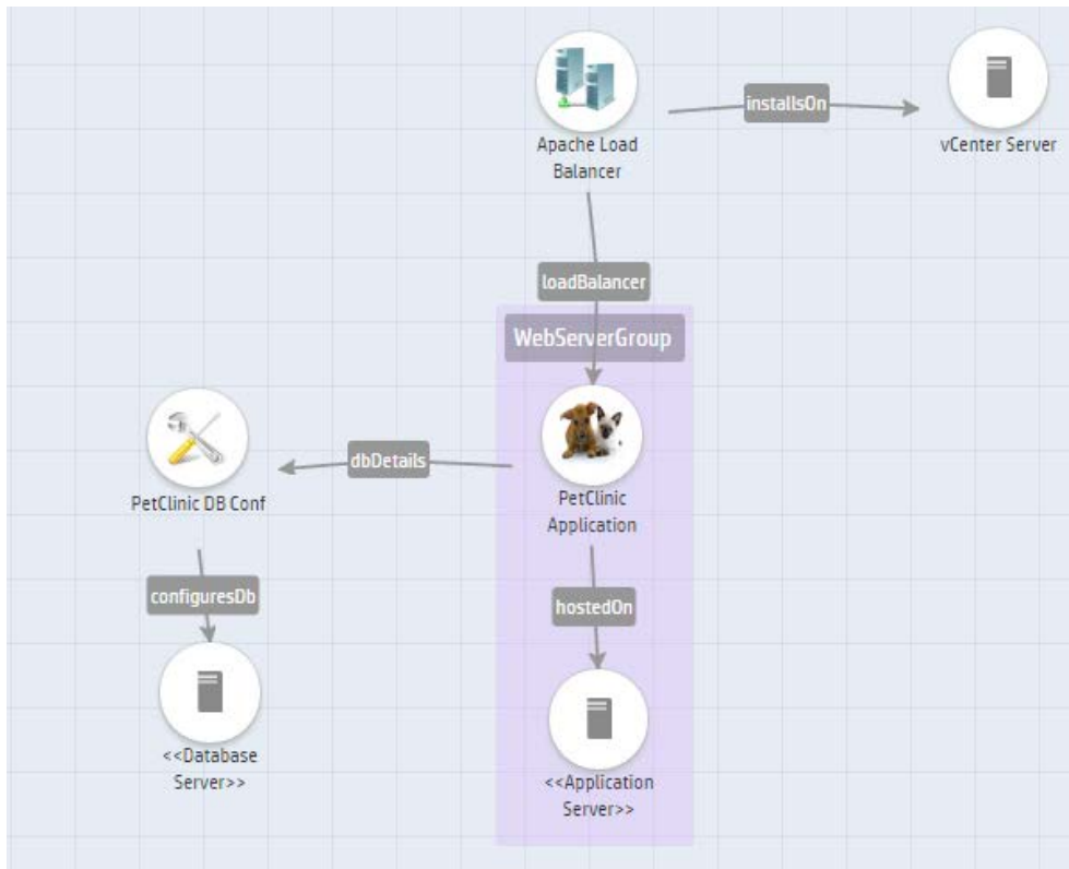
Figure 7: Partial design that contains Application and Database components with Apache load balancer
