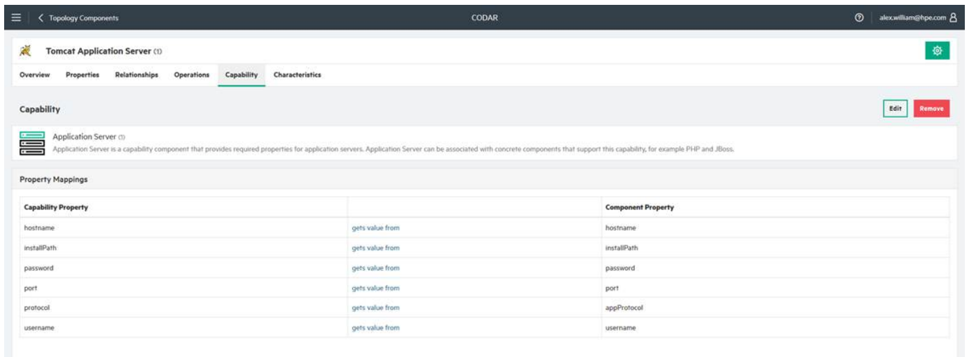
Figure 4.1: An application server capability is set for the component that can install the Tomcat server
