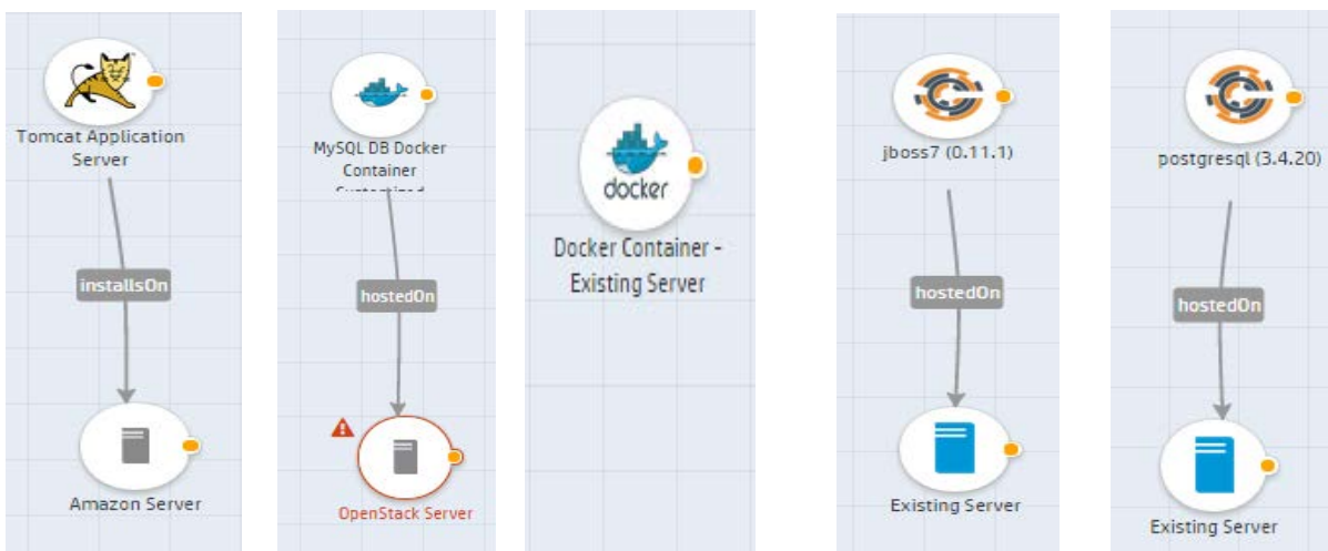
Figure 6: Single-tier AWS & OpenStack infrastructure Figure 6.1: Single-tier existing infrastructure
