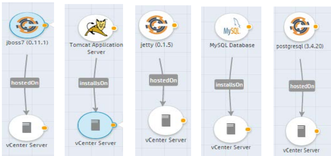
Figure 5.1: Micro Service Infrastructure designs to certify on multiple servers like Tomcat, JBoss, PostgreSQL and MySQL
