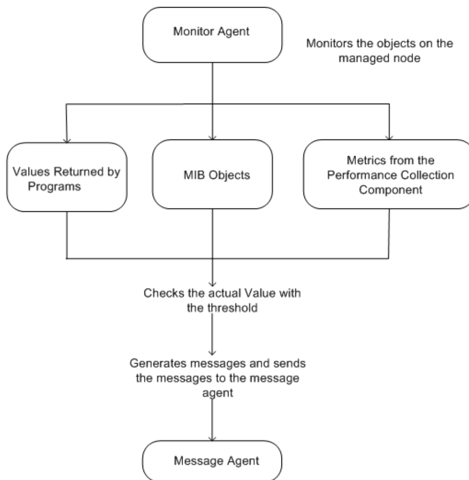
Figure 8: Workflow of the Monitor Agent
